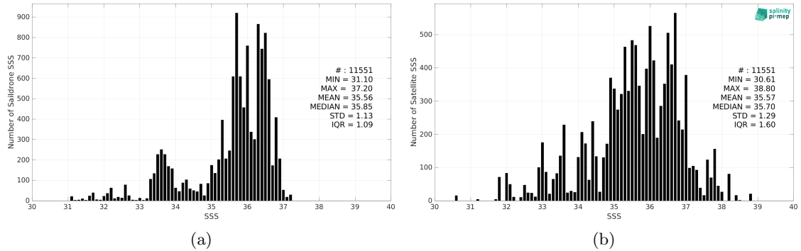
Figure 2: Histograms of SSS from Saildrone (a) and SMOS SSS L2Q v331 - 0.25 Deg (CATDS-CPDC) (b) considering all match-up pairs per bins of 0.1 over the Atlantic Ocean Pi-MEP region and for the full satellite product period.
