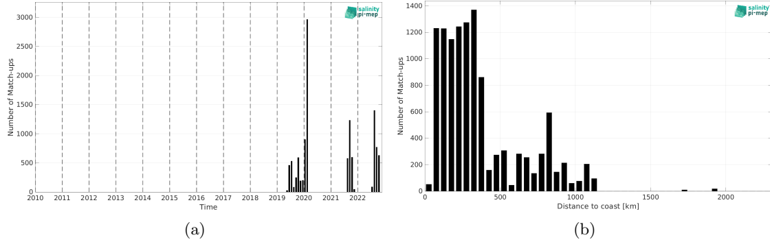
Figure 1: Number of match-ups between Saildrone and SMOS SSS L2Q v331 - 0.25 Deg (CATDS-CPDC) SSS as a function of time (a) and as function of the distance to coast (b) over the Atlantic Ocean Pi-MEP region and for the full satellite product period.
