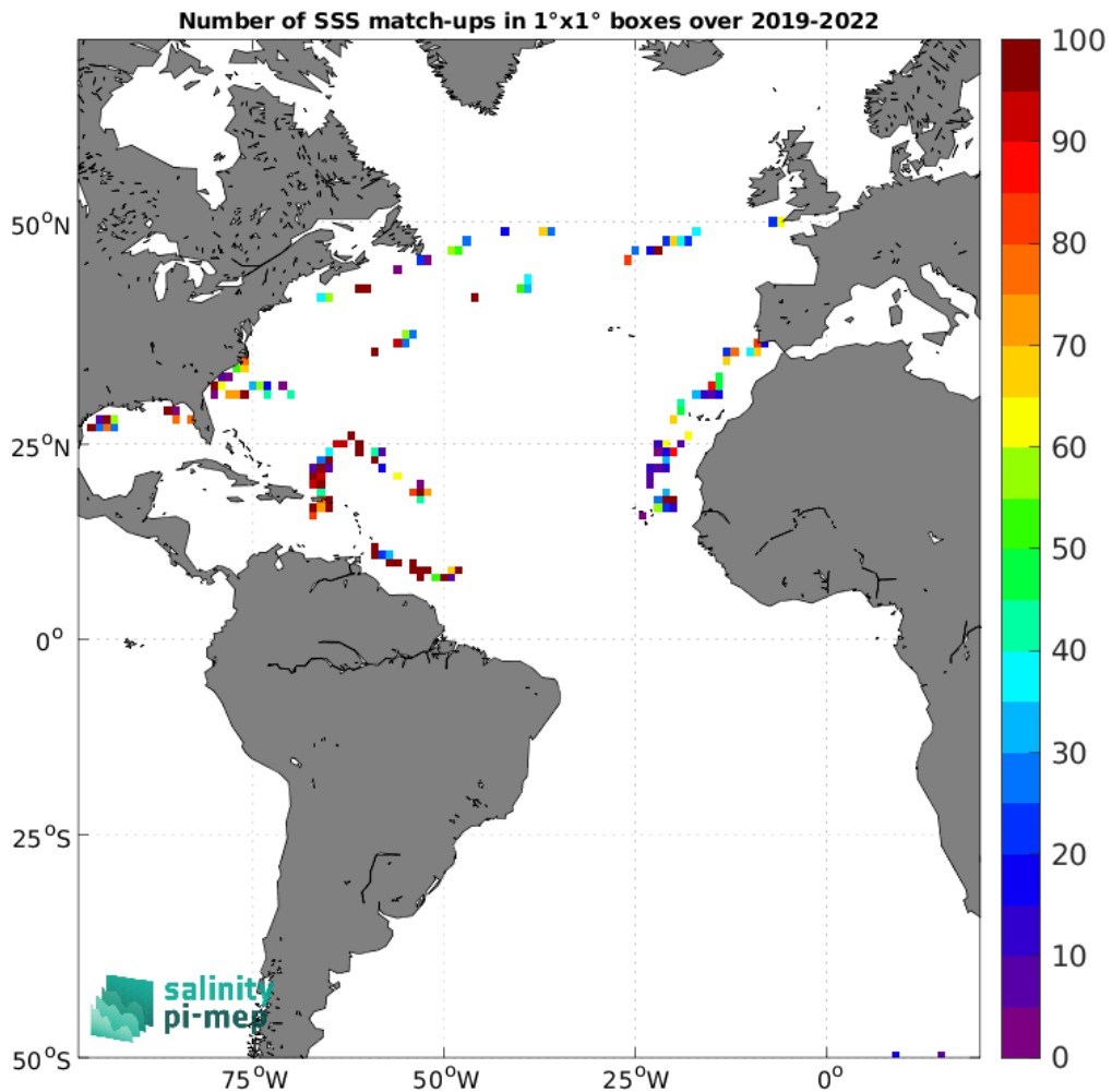
Figure 4: Number of SSS match-ups between Saildrone SSS and the SMOS SSS L2Q v331 - 0.25 Deg (CATDS-CPDC) SSS product for the Atlantic Ocean Pi-MEP region over 1°x1° boxes and for the full satellite product period.
