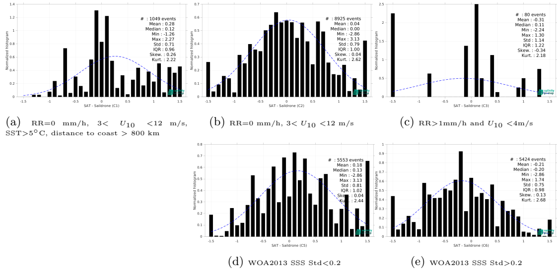
Figure 13: Normalized histogram of \Delta SSS (SMOS SSS L2Q v331 - 0.25 Deg (CATDS-CPDC) - Sailability) for 5 different subdatasets corresponding to: RR=0 mm/h, 3 < U_{10} < 12 m/s, SST>5°C, distance to coast > 800 km (a), RR=0 mm/h, 3 < U_{10} < 12 m/s (b), RR>1mm/h and U_{10} < 4 m/s (c), WOA2013 SSS Std<0.2 (d), WOA2013 SSS Std>0.2 (e).
