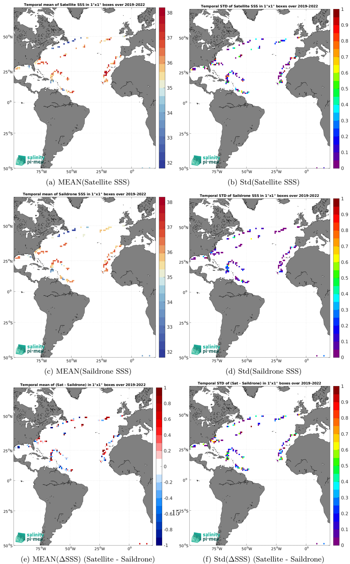
Figure 6: Temporal mean (left) and Std (right) of SSS from SMOS SSS L2Q v331 - 0.25 Deg (CATDS-CPDC) (top), Saildrone (middle), and of \Delta SSS (Satellite - Saildrone). Only match-up pairs are used to generate these maps.
