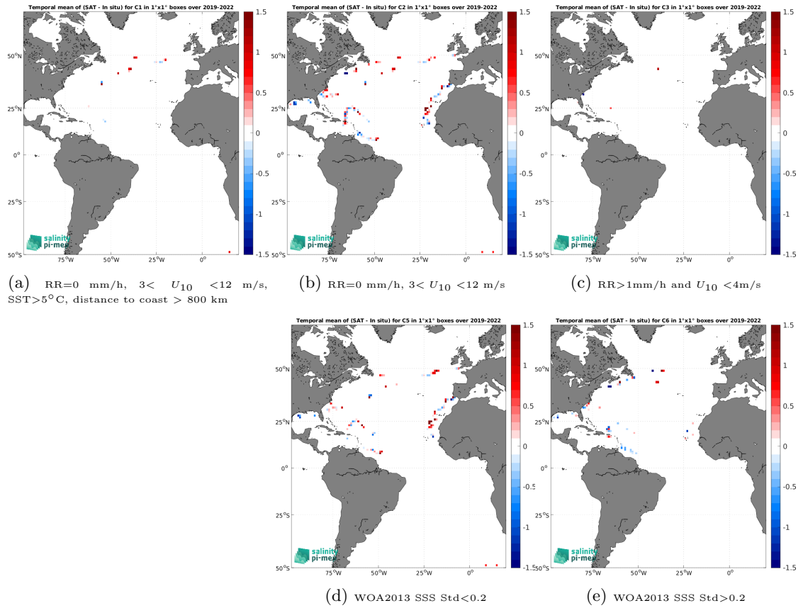
Figure 12: Temporal mean gridded over spatial boxes of size 1^\circ \times 1^\circ of \Delta\text{SSS} (SMOS SSS L2Q v331 - 0.25 Deg (CATDS-CPDC) - Sailydrone) for 5 different subdatasets corresponding to:RR=0 mm/h, 3 < U_{10} < 12 m/s, SST >5^\circ\text{C} , distance to coast > 800 km (a), RR=0 mm/h, 3 < U_{10} < 12 m/s (b), RR >1 mm/h and U_{10} < 4 m/s (c), WOA2013 SSS Std <0.2 (d), WOA2013 SSS Std >0.2 (e).
