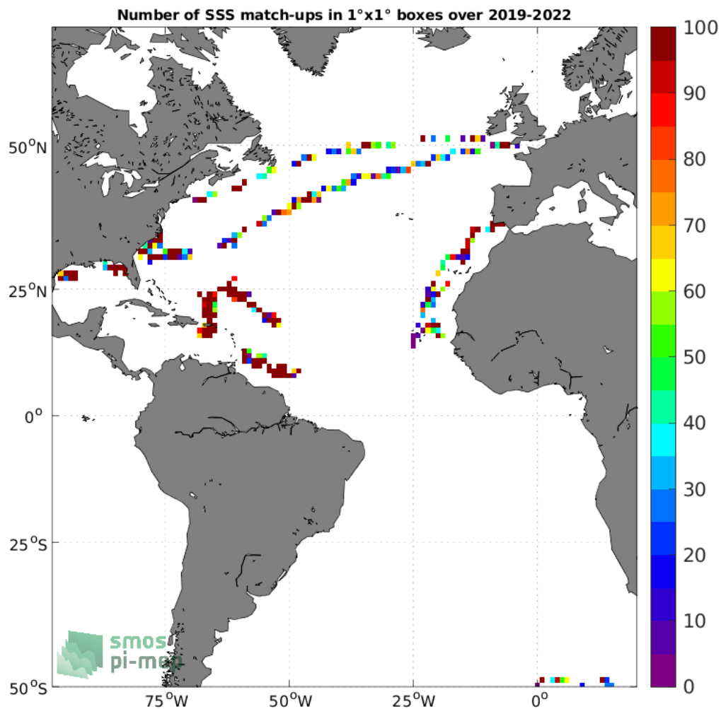
Figure 4: Number of SSS match-ups between Sairdrone SSS and the SMOS SSS L2Q v331 - 0.25 Deg (CATDS-CPDC) SSS product for the Atlantic Ocean Pi-MEP region over 1°x1° boxes and for the full satellite product period.
