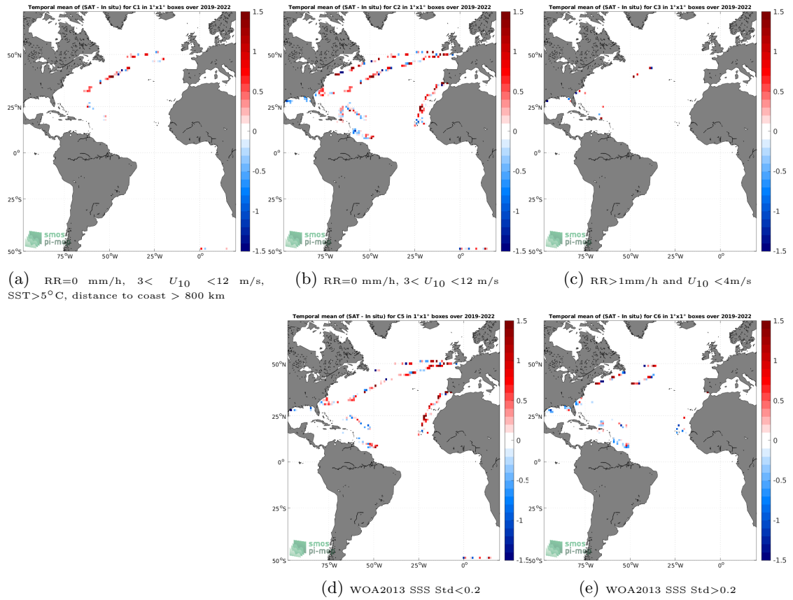
Figure 12: Temporal mean gridded over spatial boxes of size 1^\circ \times 1^\circ of \Delta SSS (SMOS SSS L2Q v331 - 0.25 Deg (CATDS-CPDC) - Sailydrone) for 5 different subdatasets corresponding to:RR=0 mm/h, 3 < U_{10} < 12 m/s, SST >5^\circ\text{C} , distance to coast > 800 km (a), RR=0 mm/h, 3 < U_{10} < 12 m/s (b), RR >1 mm/h and U_{10} < 4 m/s (c), WOA2013 SSS Std <0.2 (d), WOA2013 SSS Std >0.2 (e).
