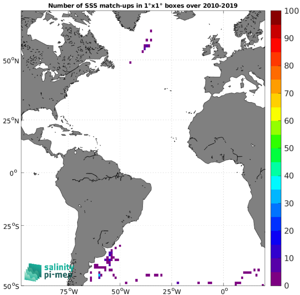
Figure 4: Number of SSS match-ups between Marine mammals SSS and the SMOS SSS L2Q v331 - 0.25 Deg (CATDS-CPDC) SSS product for the Atlantic Ocean Pi-MEP region over 1^\circ \times 1^\circ boxes and for the full satellite product period.
