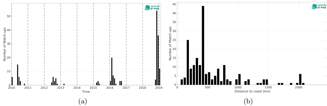
Figure 1: Number of match-ups between Marine mammals and SMOS SSS L2Q v331 - 0.25 Deg (CATDS-CPDC) SSS as a function of time (a) and as function of the distance to coast (b) over the Atlantic Ocean Pi-MEP region and for the full satellite product period.
