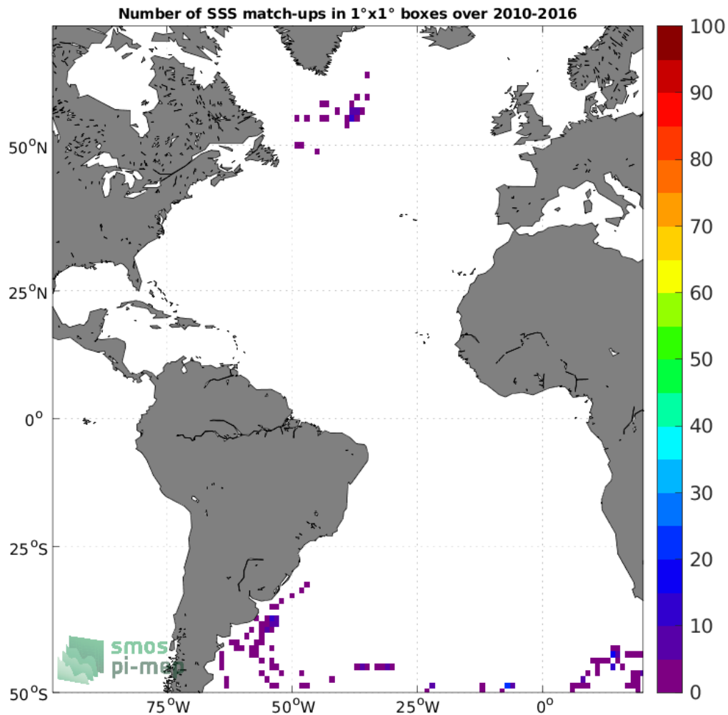
Figure 4: Number of SSS match-ups between Marine mammals SSS and the SMOS SSS L2Q v331 - 0.25 Deg (CATDS-CPDC) SSS product for the Atlantic Ocean Pi-MEP region over 1°x1° boxes and for the full satellite product period.
