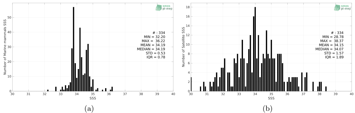
Figure 2: Histograms of SSS from Marine mammals (a) and SMOS SSS L2Q v331 - 0.25 Deg (CATDS-CPDC) (b) considering all match-up pairs per bins of 0.1 over the Atlantic Ocean Pi-MEP region and for the full satellite product period.
