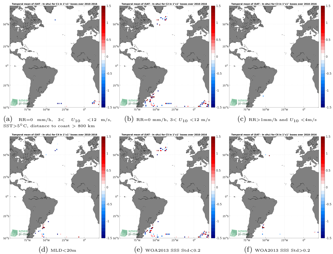
Figure 12: Temporal mean gridded over spatial boxes of size 1^\circ \times 1^\circ of \Delta SSS (SMOS SSS L2Q v331 - 0.25 Deg (CATDS-CPDC) - Marine mammals) for 6 different subdatasets corresponding to:RR=0 mm/h, 3 < U_{10} < 12 m/s, SST >5^\circ C, distance to coast > 800 km (a), RR=0 mm/h, 3 < U_{10} < 12 m/s (b), RR >1 mm/h and U_{10} < 4 m/s (c),MLD <20 m (d),WOA2013 SSS Std <0.2 (e),WOA2013 SSS Std >0.2 (f).
