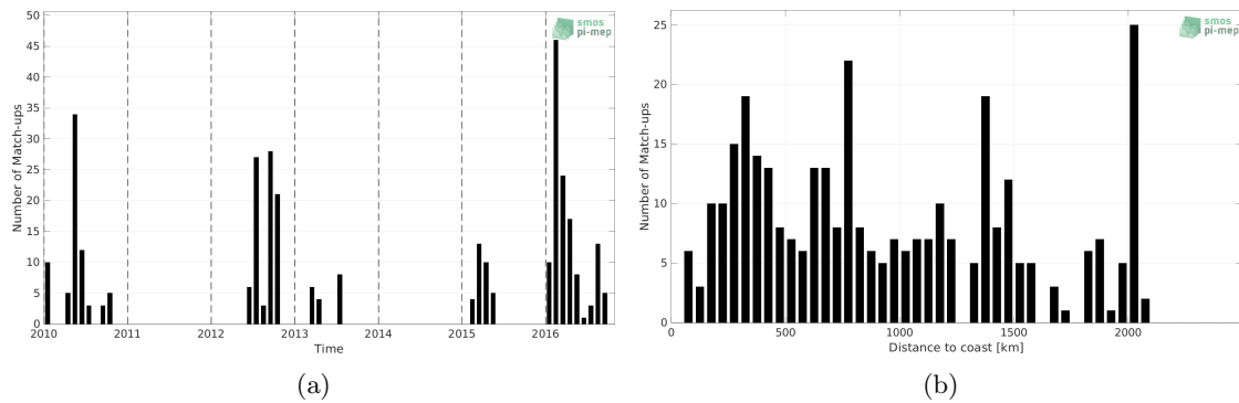
Figure 1: Number of match-ups between Marine mammals and SMOS SSS L2Q v331 - 0.25 Deg (CATDS-CPDC) SSS as a function of time (a) and as function of the distance to coast (b) over the Atlantic Ocean Pi-MEP region and for the full satellite product period.
