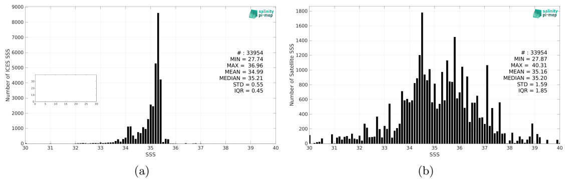
Figure 2: Histograms of SSS from ICES (a) and SMOS SSS L2Q v331 - 0.25 Deg (CATDS-CPDC) (b) considering all match-up pairs per bins of 0.1 over the Atlantic Ocean Pi-MEP region and for the full satellite product period.
