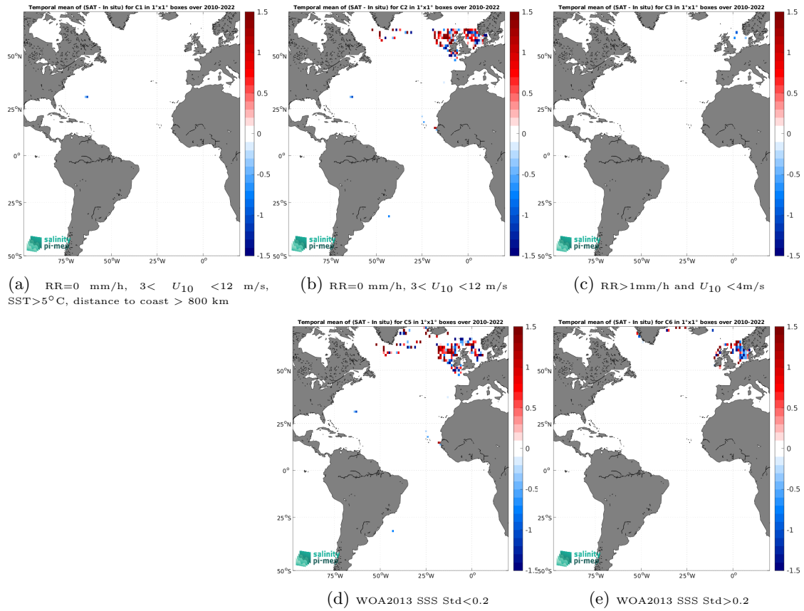
Figure 12: Temporal mean gridded over spatial boxes of size 1^\circ \times 1^\circ of \Delta SSS (SMOS SSS L2Q v331 - 0.25 Deg (CATDS-CPDC) - ICES) for 5 different subdatasets corresponding to:RR=0 mm/h, 3 < U_{10} < 12 m/s, SST >5^\circ\text{C} , distance to coast > 800 km (a), RR=0 mm/h, 3 < U_{10} < 12 m/s (b), RR >1 mm/h and U_{10} < 4 m/s (c), WOA2013 SSS Std <0.2 (d), WOA2013 SSS Std >0.2 (e).
