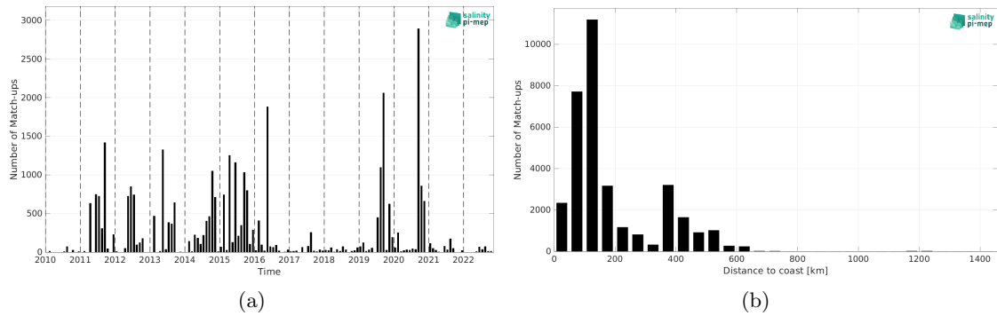
Figure 1: Number of match-ups between ICES and SMOS SSS L2Q v331 - 0.25 Deg (CATDS-CPDC) SSS as a function of time (a) and as function of the distance to coast (b) over the Atlantic Ocean Pi-MEP region and for the full satellite product period.
