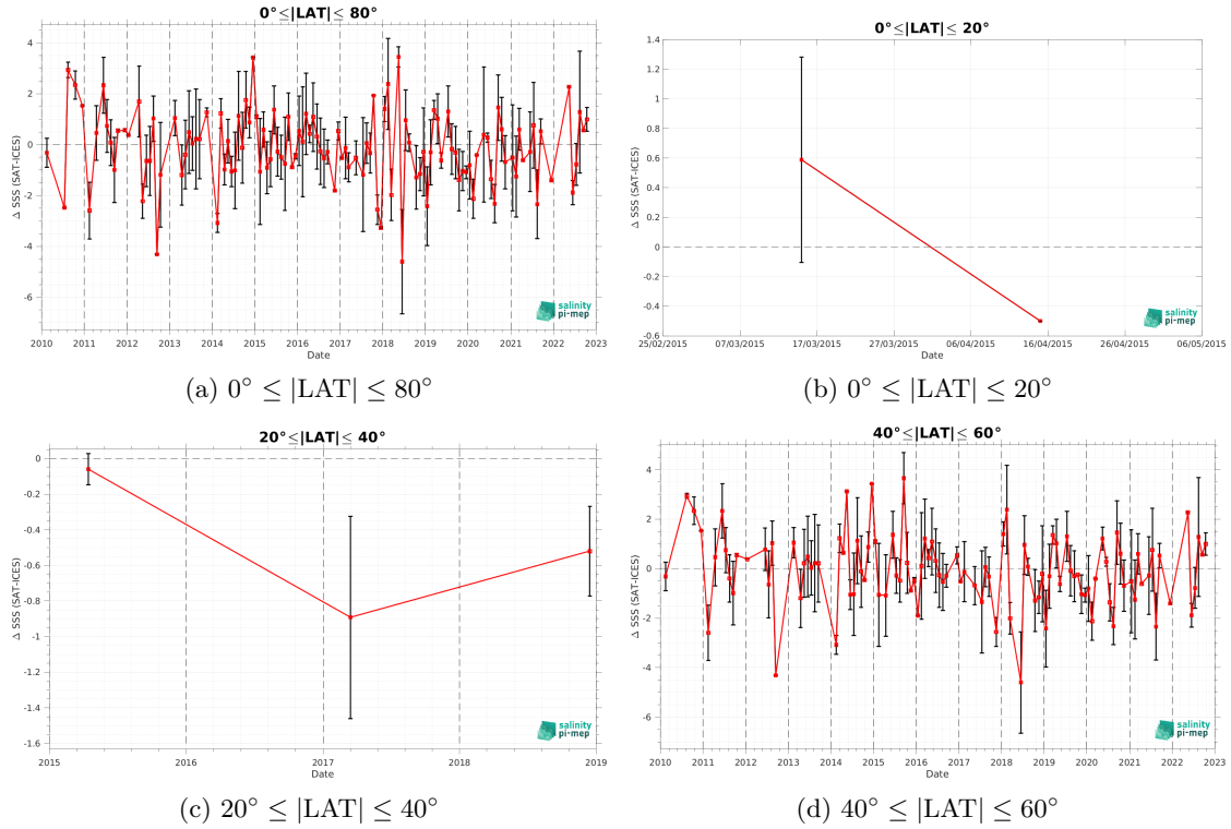
Figure 10: Monthly median (red curves) of \Delta SSS (Satellite - ICES) and \pm 1 Std (black vertical thick bars) as function of time for all the collected Pi-MEP match-up pairs estimated over the Atlantic Ocean Pi-MEP region and for the full satellite product period are shown for different latitude bands: (a) 80°S-80°N, (b) 20°S-20°N, (c) 40°S-20°S and 20°N-40°N and (d) 60°S-40°S and 40°N-60°N.
