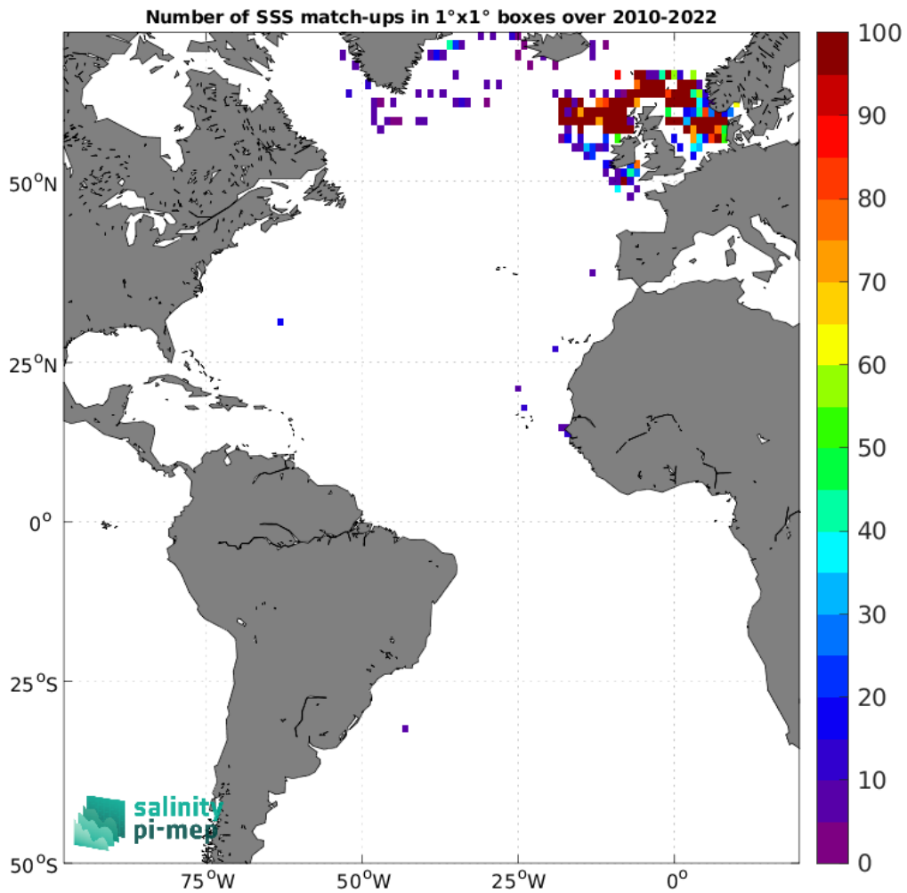
Figure 4: Number of SSS match-ups between ICES SSS and the SMOS SSS L2Q v331 - 0.25 Deg (CATDS-CPDC) SSS product for the Atlantic Ocean Pi-MEP region over 1°×1° boxes and for the full satellite product period.
