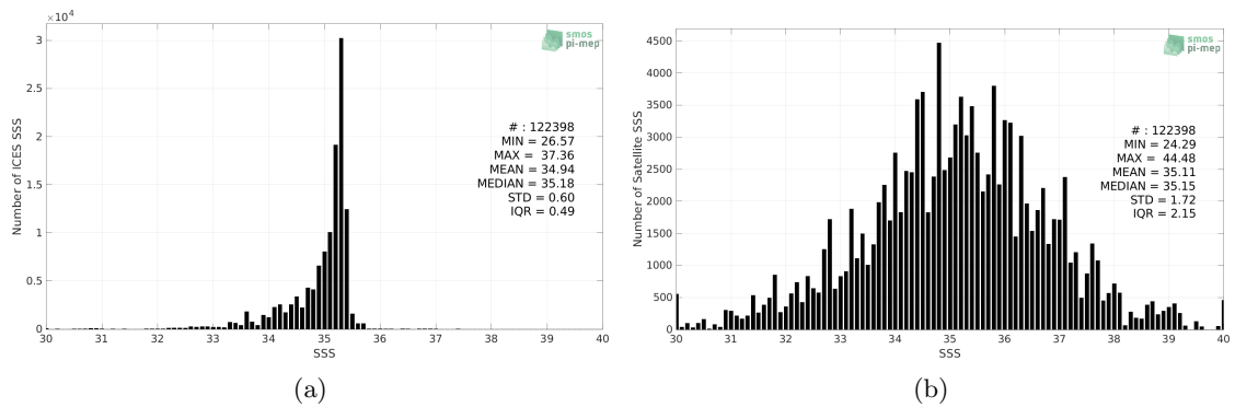
Figure 2: Histograms of SSS from ICES (a) and SMOS SSS L2Q v331 - 0.25 Deg (CATDS-CPDC) (b) considering all match-up pairs per bins of 0.1 over the Atlantic Ocean Pi-MEP region and for the full satellite product period.
