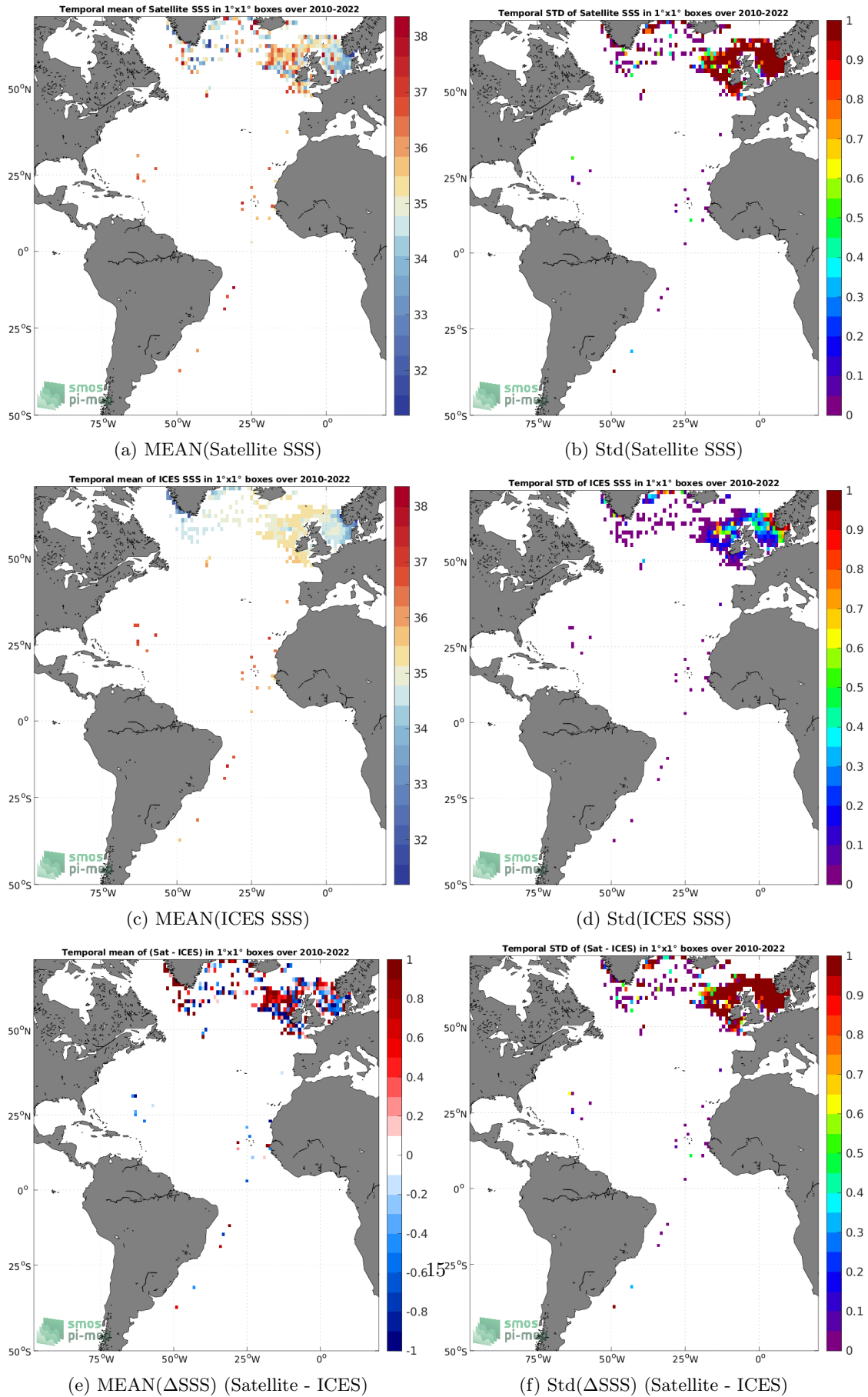
Figure 6: Temporal mean (left) and Std (right) of SSS from SMOS SSS L2Q v331 - 0.25 Deg (CATDS-CPDC) (top), ICES (middle), and of \Delta SSS (Satellite - ICES). Only match-up pairs are used to generate these maps.
