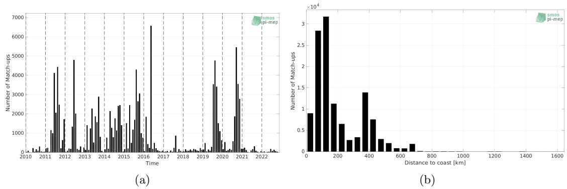
Figure 1: Number of match-ups between ICES and SMOS SSS L2Q v331 - 0.25 Deg (CATDS-CPDC) SSS as a function of time (a) and as function of the distance to coast (b) over the Atlantic Ocean Pi-MEP region and for the full satellite product period.
