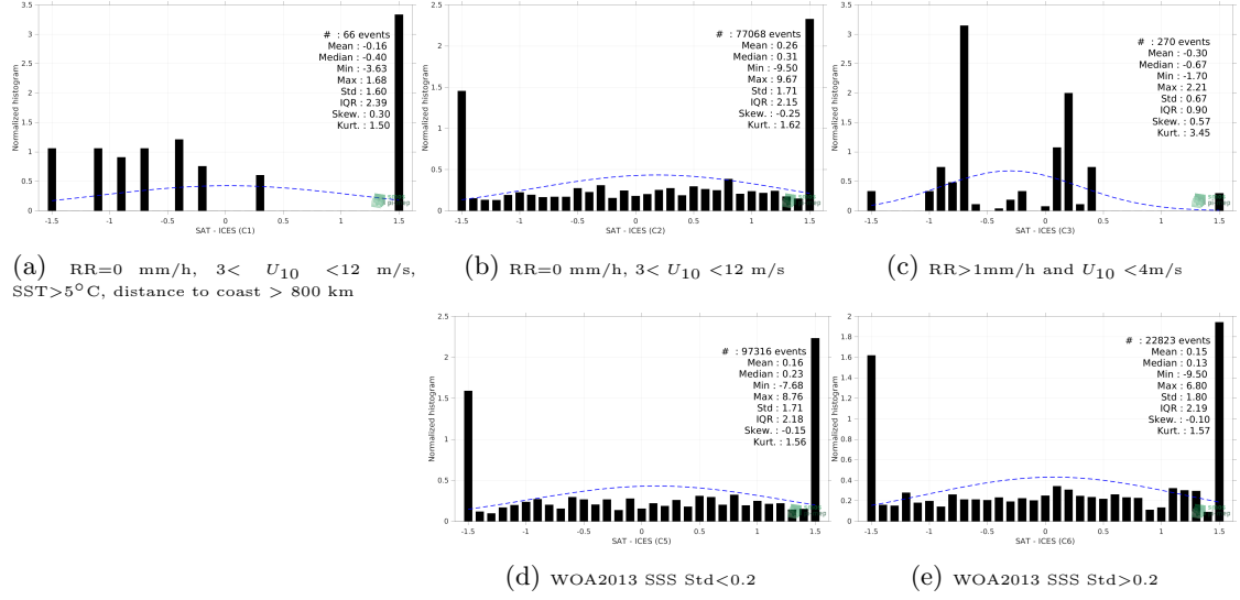
Figure 13: Normalized histogram of \Delta SSS (SMOS SSS L2Q v331 - 0.25 Deg (CATDS-CPDC) - ICES) for 5 different subdatasets corresponding to: RR=0 mm/h, 3 < U_{10} < 12 m/s, SST > 5°C, distance to coast > 800 km (a), RR=0 mm/h, 3 < U_{10} < 12 m/s (b), RR > 1mm/h and U_{10} < 4 m/s (c), WOA2013 SSS Std < 0.2 (d), WOA2013 SSS Std > 0.2 (e).
