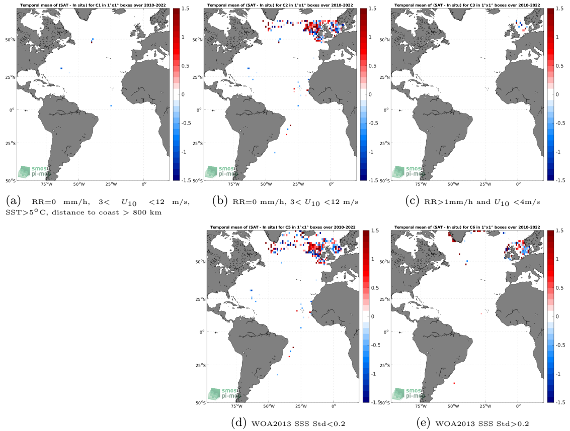
Figure 12: Temporal mean gridded over spatial boxes of size 1^\circ \times 1^\circ of \Delta SSS (SMOS SSS L2Q v331 - 0.25 Deg (CATDS-CPDC) - ICES) for 5 different subdatasets corresponding to:RR=0 mm/h, 3 < U_{10} < 12 m/s, SST >5^\circ C, distance to coast > 800 km (a), RR=0 mm/h, 3 < U_{10} < 12 m/s (b), RR >1 mm/h and U_{10} < 4 m/s (c), WOA2013 SSS Std <0.2 (d), WOA2013 SSS Std >0.2 (e).
