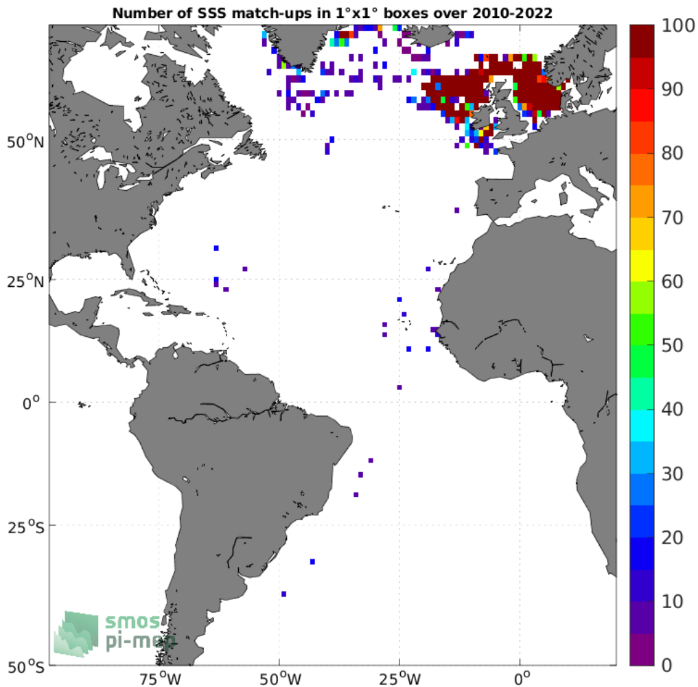
Figure 4: Number of SSS match-ups between ICES SSS and the SMOS SSS L2Q v331 - 0.25 Deg (CATDS-CPDC) SSS product for the Atlantic Ocean Pi-MEP region over 1°x1° boxes and for the full satellite product period.
