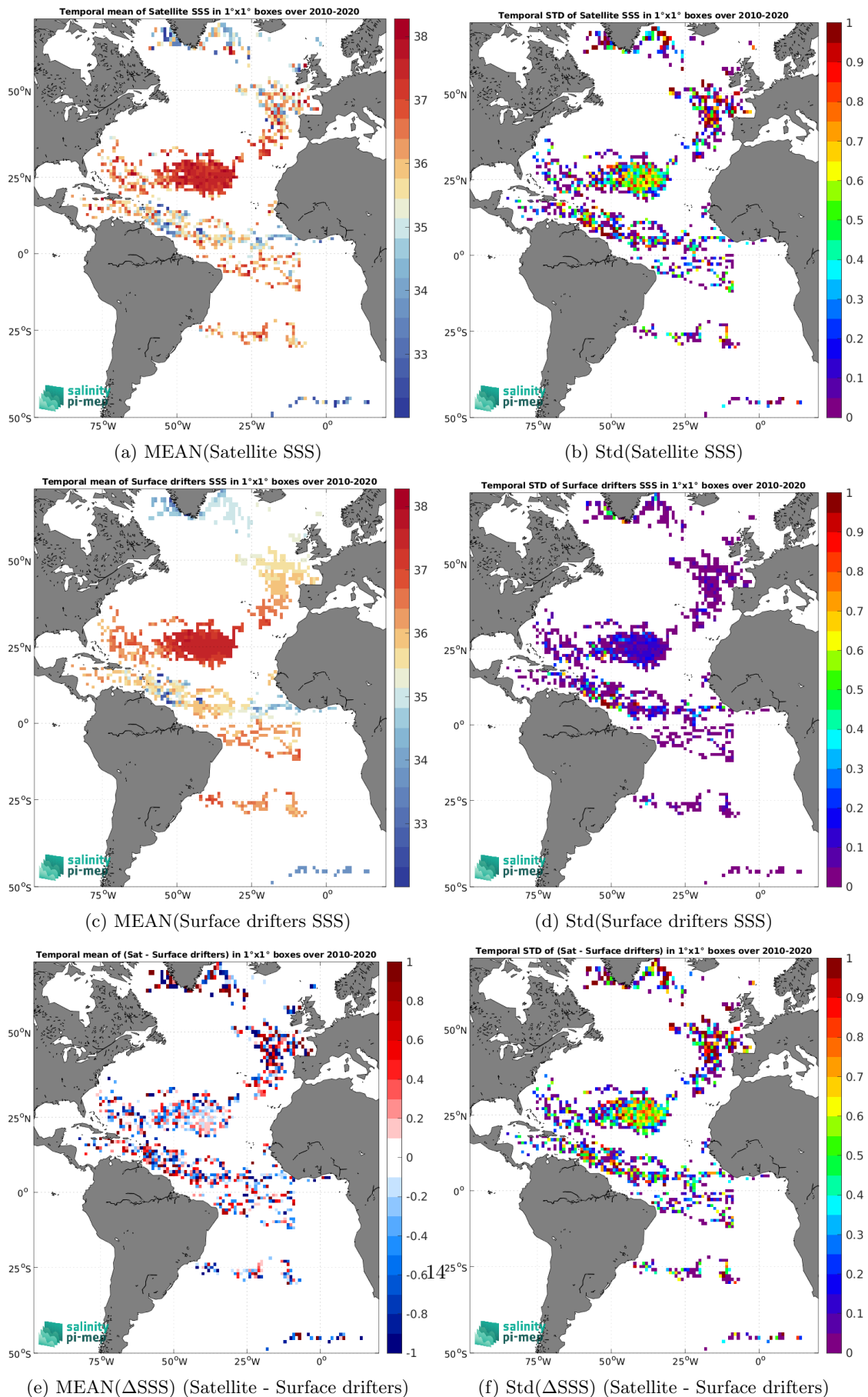
(e) MEAN( \Delta SSS) (Satellite - Surface drifters) (f) Std( \Delta SSS) (Satellite - Surface drifters) Figure 5: Temporal mean (left) and Std (right) of SSS from SMOS SSS L2Q v331 - 0.25 Deg (CATDS-CPDC) (top), Surface drifters (middle), and of \Delta SSS (Satellite - Surface drifters). Only match-up pairs are used to generate these maps.
