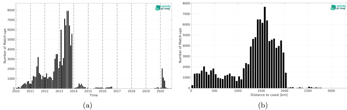
Figure 1: Number of match-ups between Surface drifters and SMOS SSS L2Q v331 - 0.25 Deg (CATDS-CPDC) SSS as a function of time (a) and as function of the distance to coast (b) over the Atlantic Ocean Pi-MEP region and for the full satellite product period.
