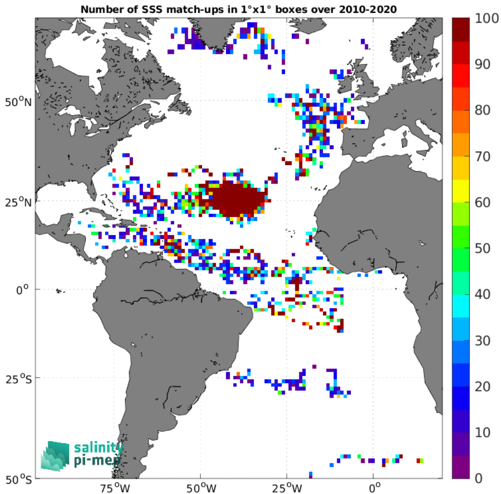
Figure 3: Number of SSS match-ups between Surface drifters SSS and the SMOS SSS L2Q v331 - 0.25 Deg (CATDS-CPDC) SSS product for the Atlantic Ocean Pi-MEP region over 1°x1° boxes and for the full satellite product period.
