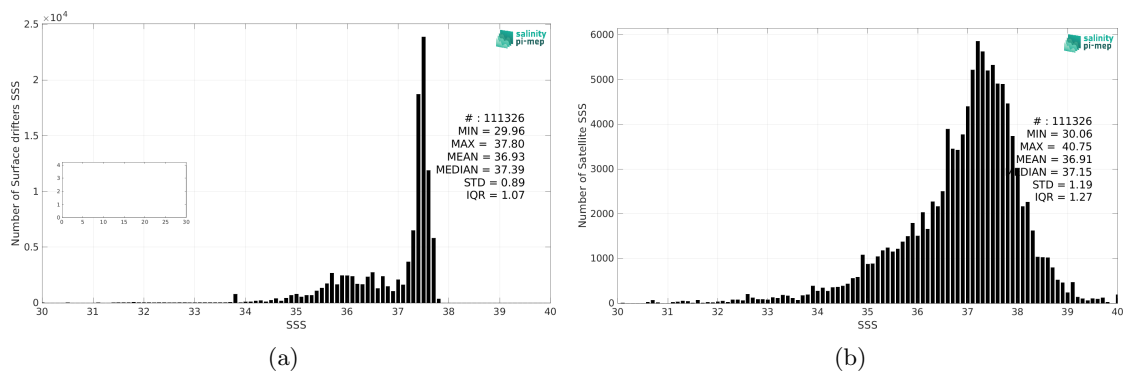
Figure 2: Histograms of SSS from Surface drifters (a) and SMOS SSS L2Q v331 - 0.25 Deg (CATDS-CPDC) (b) considering all match-up pairs per bins of 0.1 over the Atlantic Ocean Pi-MEP region and for the full satellite product period.
