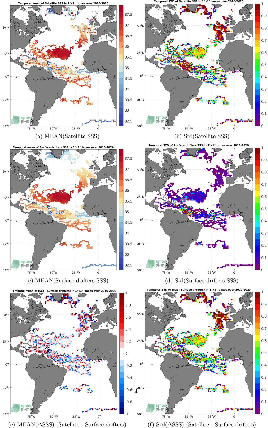
Figure 5: Temporal mean (left) and Std (right) of SSS from SMOS SSS L2Q v331 - 0.25 Deg (CATDS-CPDC) (top), Surface drifters (middle), and of \Delta SSS (Satellite - Surface drifters). Only match-up pairs are used to generate these maps.
