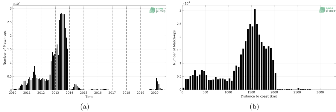
Figure 1: Number of match-ups between Surface drifters and SMOS SSS L2Q v331 - 0.25 Deg (CATDS-CPDC) SSS as a function of time (a) and as function of the distance to coast (b) over the Atlantic Ocean Pi-MEP region and for the full satellite product period.
