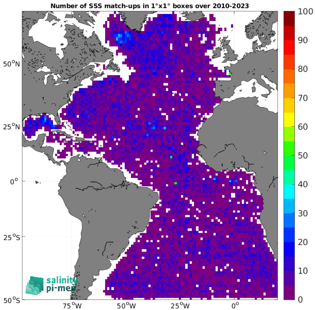
Figure 4: Number of SSS match-ups between Argo SSS and the SMOS SSS L2Q v331 - 0.25 Deg (CATDS-CPDC) SSS product for the Atlantic Ocean Pi-MEP region over 1^\circ \times 1^\circ boxes and for the full satellite product period.
