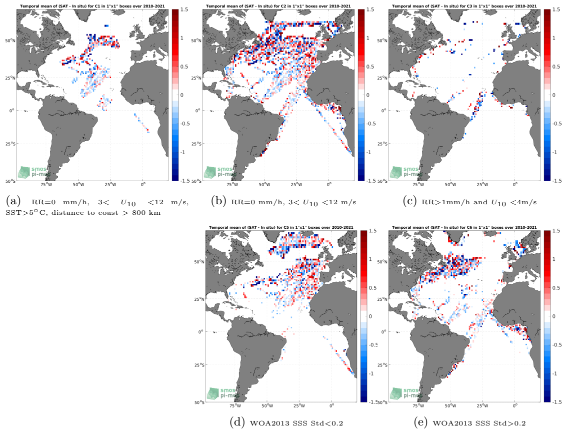
Figure 12: Temporal mean gridded over spatial boxes of size 1^\circ \times 1^\circ of \Delta SSS (SMOS SSS L2Q v330 - 0.25 Deg (CATDS-CPDC) - TSG (LEGOS-DM)) for 5 different subdatasets corresponding to:RR=0 mm/h, 3 < U_{10} < 12 m/s, SST >5^\circ\text{C} , distance to coast > 800 km (a), RR=0 mm/h, 3 < U_{10} < 12 m/s (b), RR >1 mm/h and U_{10} < 4 m/s (c), WOA2013 SSS Std <0.2 (d), WOA2013 SSS Std >0.2 (e).
