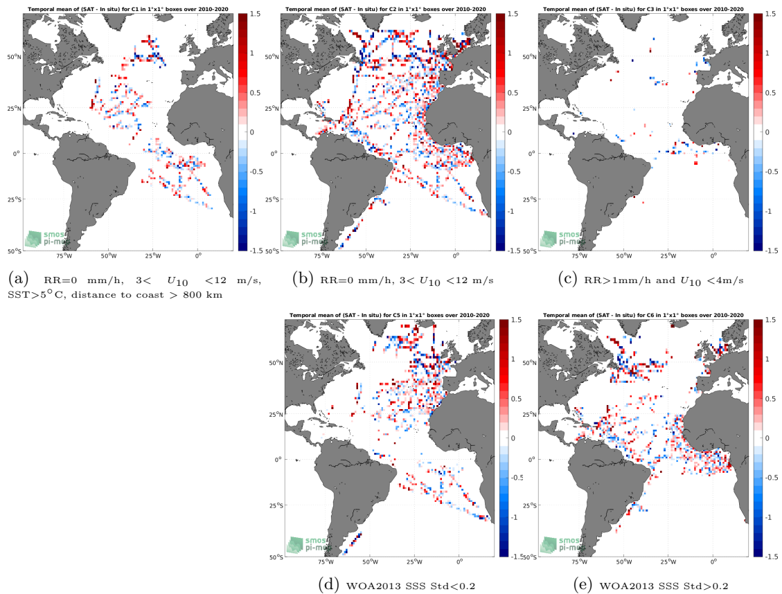
Figure 12: Temporal mean gridded over spatial boxes of size 1^\circ \times 1^\circ of \Delta\text{SSS} (SMOS SSS L2Q v330 - 0.25 Deg (CATDS-CPDC) - TSG (GOSUD-Research-vessel)) for 5 different subdatasets corresponding to:RR=0 mm/h, 3 < U_{10} < 12 m/s, SST>5°C, distance to coast > 800 km (a), RR=0 mm/h, 3 < U_{10} < 12 m/s (b), RR>1mm/h and U_{10} < 4 m/s (c), WOA2013 SSS Std<0.2 (d), WOA2013 SSS Std>0.2 (e).
