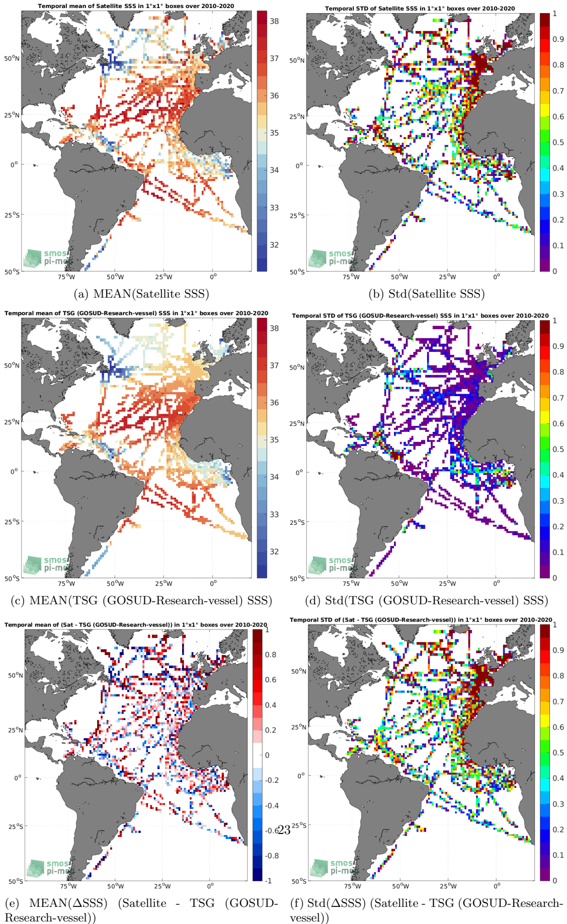
Figure 6: Temporal mean (left) and Std (right) of SSS from SMOS SSS L2Q v330 - 0.25 Deg (CATDS-CPDC) (top), TSG (GOSUD-Research-vessel) (middle), and of \Delta SSS (Satellite - TSG (GOSUD-Research-vessel)). Only match-up pairs are used to generate these maps.
