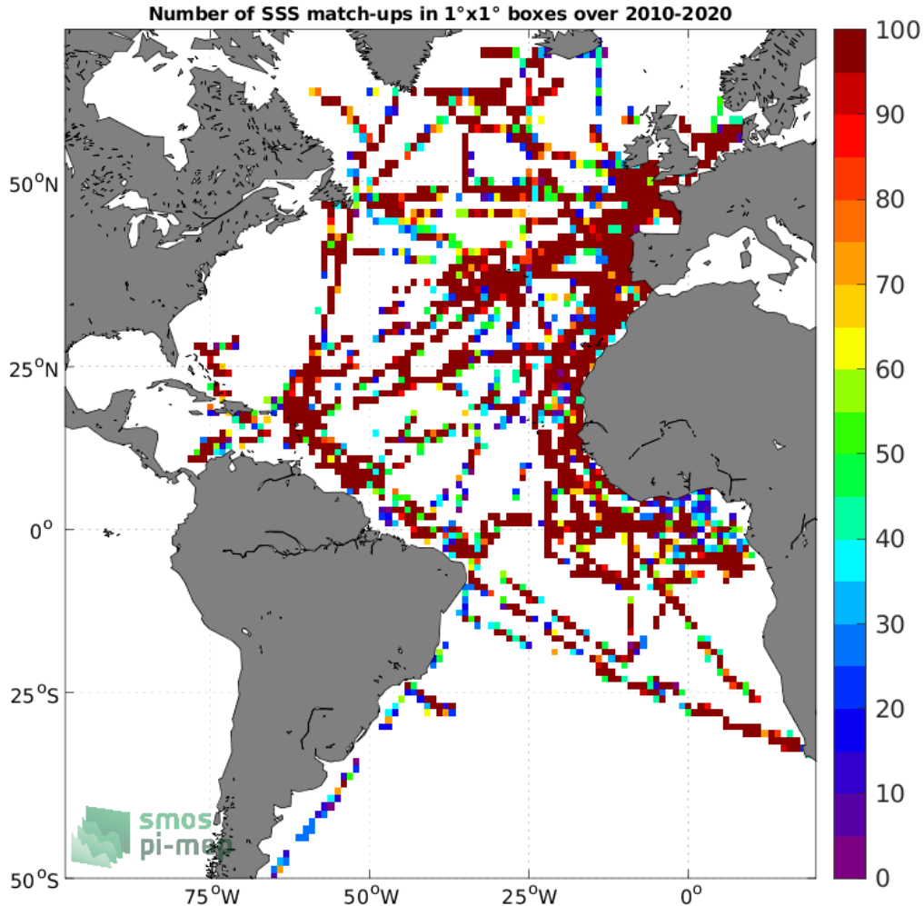
Figure 4: Number of SSS match-ups between TSG (GOSUD-Research-vessel) SSS and the SMOS SSS L2Q v330 - 0.25 Deg (CATDS-CPDC) SSS product for the Atlantic Ocean Pi-MEP region over 1^\circ \times 1^\circ boxes and for the full satellite product period.
