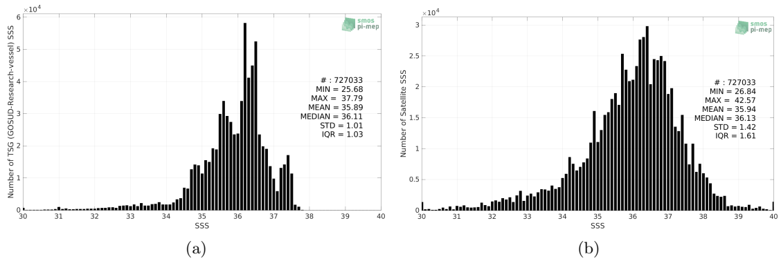
Figure 2: Histograms of SSS from TSG (GOSUD-Research-vessel) (a) and SMOS SSS L2Q v330 - 0.25 Deg (CATDS-CPDC) (b) considering all match-up pairs per bins of 0.1 over the Atlantic Ocean Pi-MEP region and for the full satellite product period.
