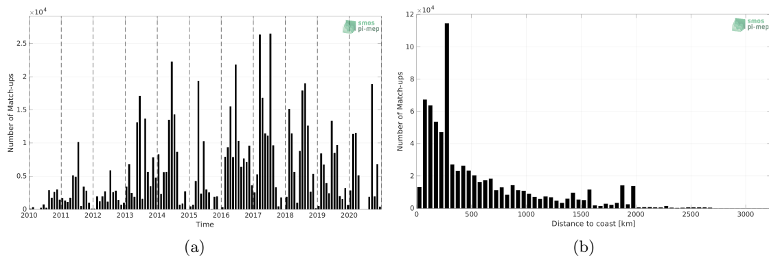
Figure 1: Number of match-ups between TSG (GOSUD-Research-vessel) and SMOS SSS L2Q v330 - 0.25 Deg (CATDS-CPDC) SSS as a function of time (a) and as function of the distance to coast (b) over the Atlantic Ocean Pi-MEP region and for the full satellite product period.
