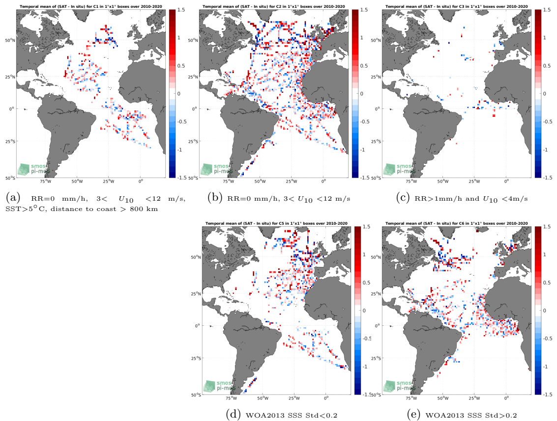
Figure 12: Temporal mean gridded over spatial boxes of size 1^\circ \times 1^\circ of \Delta\text{SSS} (SMOS SSS L2Q v330 - 0.25 Deg (CATDS-CPDC) - TSG (GOSUD-Research-vessel)) for 5 different subdatasets corresponding to:RR=0 mm/h, 3 < U_{10} < 12 m/s, SST>5°C, distance to coast > 800 km (a), RR=0 mm/h, 3 < U_{10} < 12 m/s (b), RR>1mm/h and U_{10} < 4 m/s (c), WOA2013 SSS Std<0.2 (d), WOA2013 SSS Std>0.2 (e).
