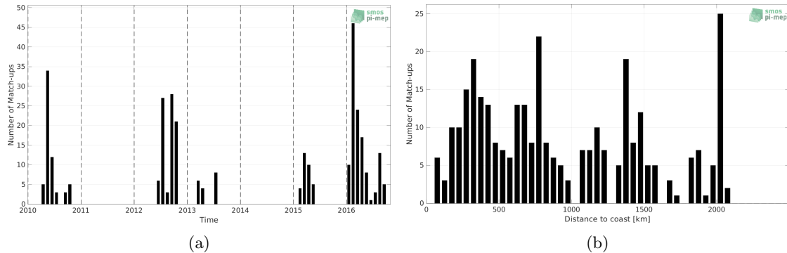
Figure 1: Number of match-ups between Marine mammals and SMOS SSS L2Q v330 - 0.25 Deg (CATDS-CPDC) SSS as a function of time (a) and as function of the distance to coast (b) over the Atlantic Ocean Pi-MEP region and for the full satellite product period.
