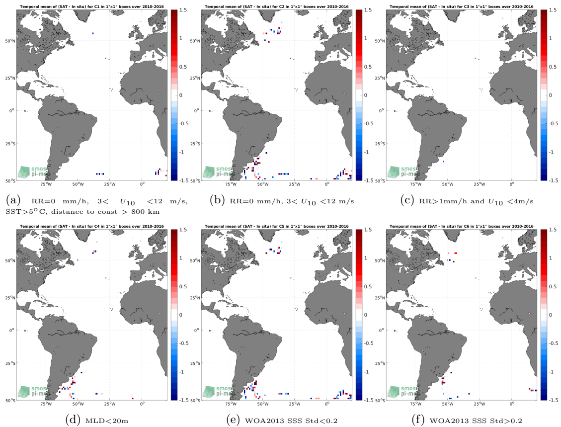
Figure 12: Temporal mean gridded over spatial boxes of size 1^\circ \times 1^\circ of \Delta SSS (SMOS SSS L2Q v330 - 0.25 Deg (CATDS-CPDC) - Marine mammals) for 6 different subdatasets corresponding to:RR=0 mm/h, 3 < U_{10} < 12 m/s, SST >5^\circ C, distance to coast > 800 km (a), RR=0 mm/h, 3 < U_{10} < 12 m/s (b), RR >1 mm/h and U_{10} < 4 m/s (c),MLD <20 m (d),WOA2013 SSS Std <0.2 (e),WOA2013 SSS Std >0.2 (f).
