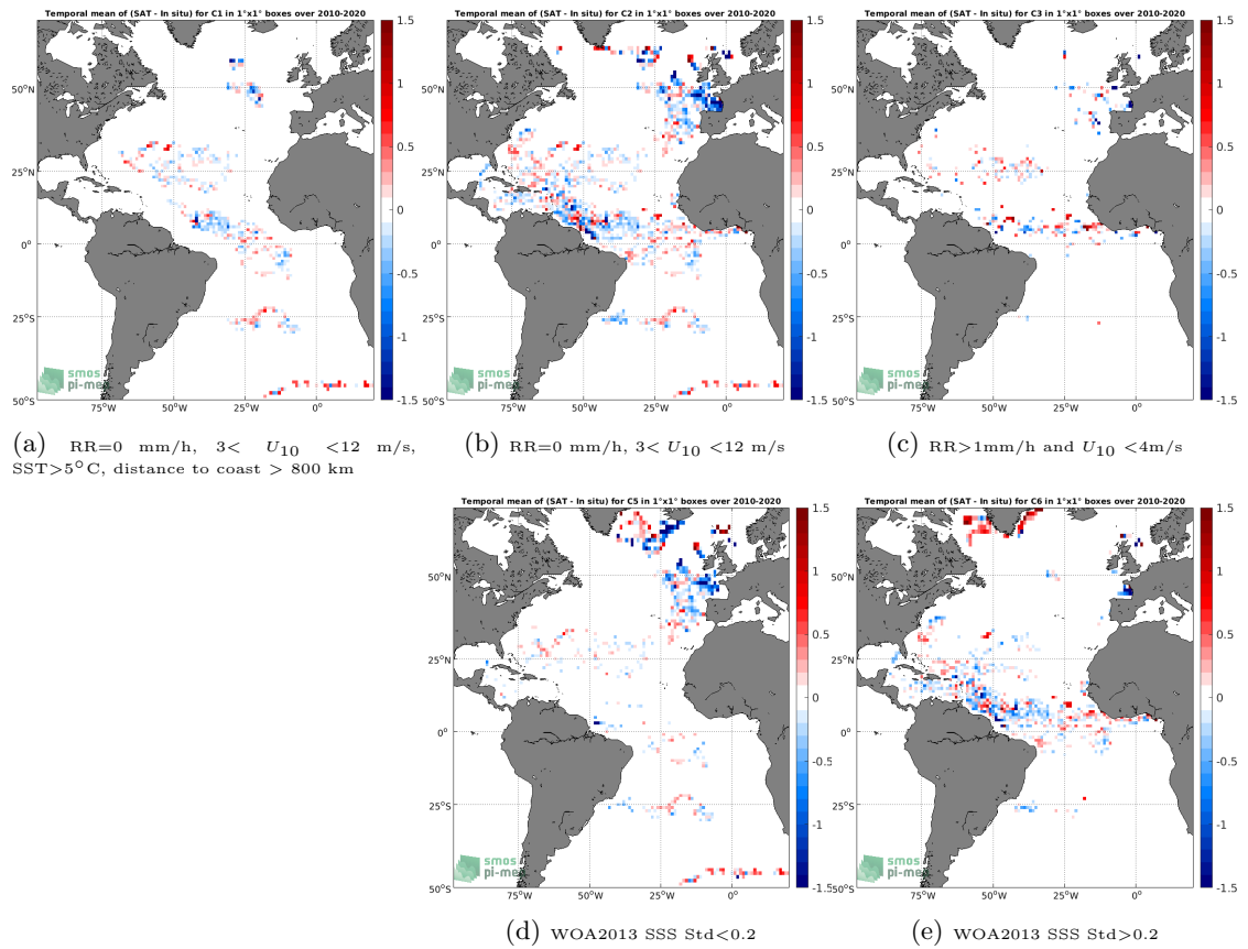
Figure 11: Temporal mean gridded over spatial boxes of size 1^\circ \times 1^\circ of \Delta SSS (SMOS SSS L3 v317 - 10 Days - 25 km (CATDS-CPDC) - Surface drifters) for 5 different subdatasets corresponding to:RR=0 mm/h, 3 < U_{10} < 12 m/s, SST>5°C, distance to coast > 800 km (a), RR=0 mm/h, 3 < U_{10} < 12 m/s (b), RR>1mm/h and U_{10} < 4 m/s (c), WOA2013 SSS Std<0.2 (d), WOA2013 SSS Std>0.2 (e).
