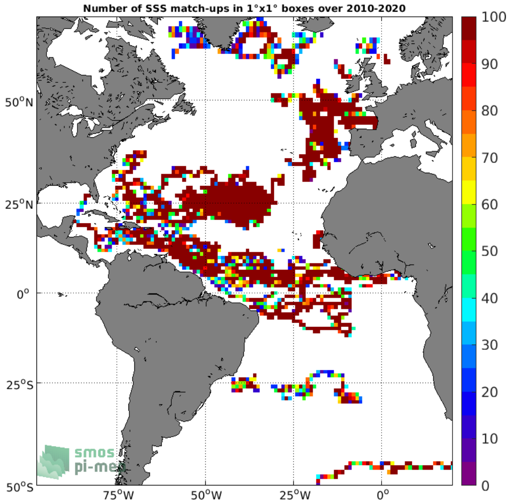
Figure 3: Number of SSS match-ups between Surface drifters SSS and the SMOS SSS L3 v317 - 10 Days - 25 km (CATDS-CPDC) SSS product for the Atlantic Ocean Pi-MEP region over 1^\circ \times 1^\circ boxes and for the full satellite product period.
