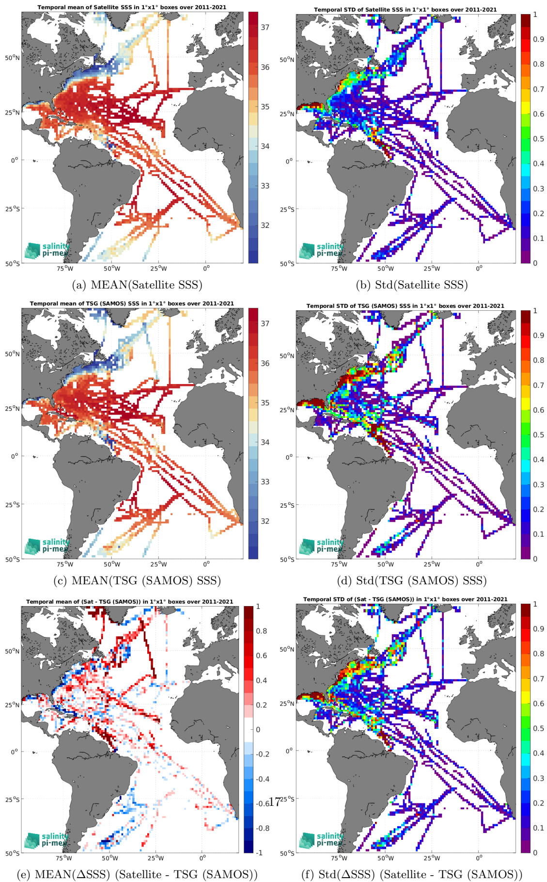
Figure 7: Temporal mean (left) and Std (right) of SSS from SMOS SSS L3 v2 - 9-Days (BEC) (top), TSG (SAMOS) (middle), and of \Delta SSS (Satellite - TSG (SAMOS)). Only match-up pairs are used to generate these maps.
