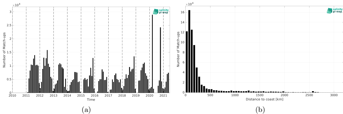
Figure 2: Number of match-ups between TSG (SAMOS) and SMOS SSS L3 v2 - 9-Days (BEC) SSS as a function of time (a) and as function of the distance to coast (b) over the Atlantic Ocean Pi-MEP region and for the full satellite product period.
