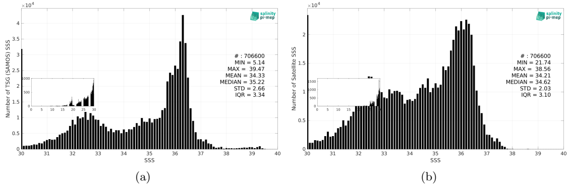
Figure 3: Histograms of SSS from TSG (SAMOS) (a) and SMOS SSS L3 v2 - 9-Days (BEC) (b) considering all match-up pairs per bins of 0.1 over the Atlantic Ocean Pi-MEP region and for the full satellite product period.
