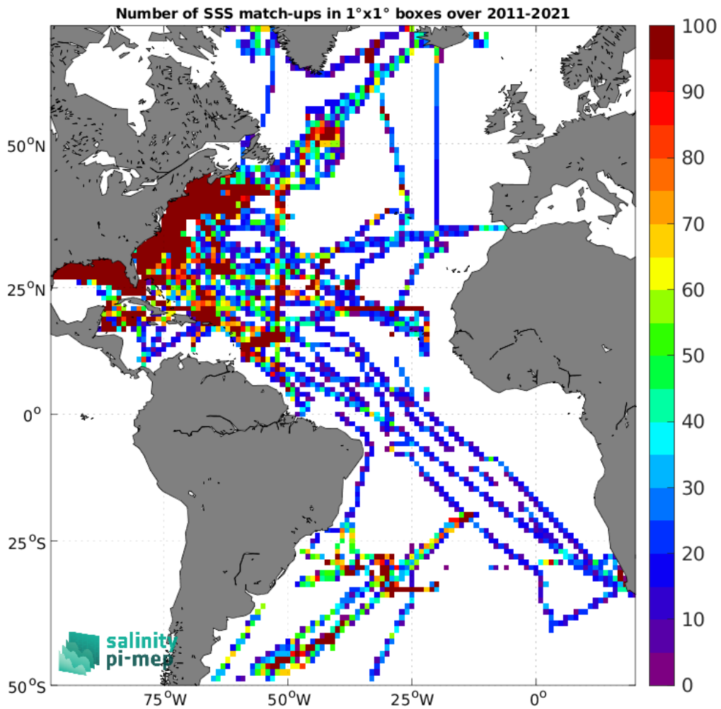
Figure 5: Number of SSS match-ups between TSG (SAMOS) SSS and the SMOS SSS L3 v2 - 9-Days (BEC) SSS product for the Atlantic Ocean Pi-MEP region over 1^\circ \times 1^\circ boxes and for the full satellite product period.
