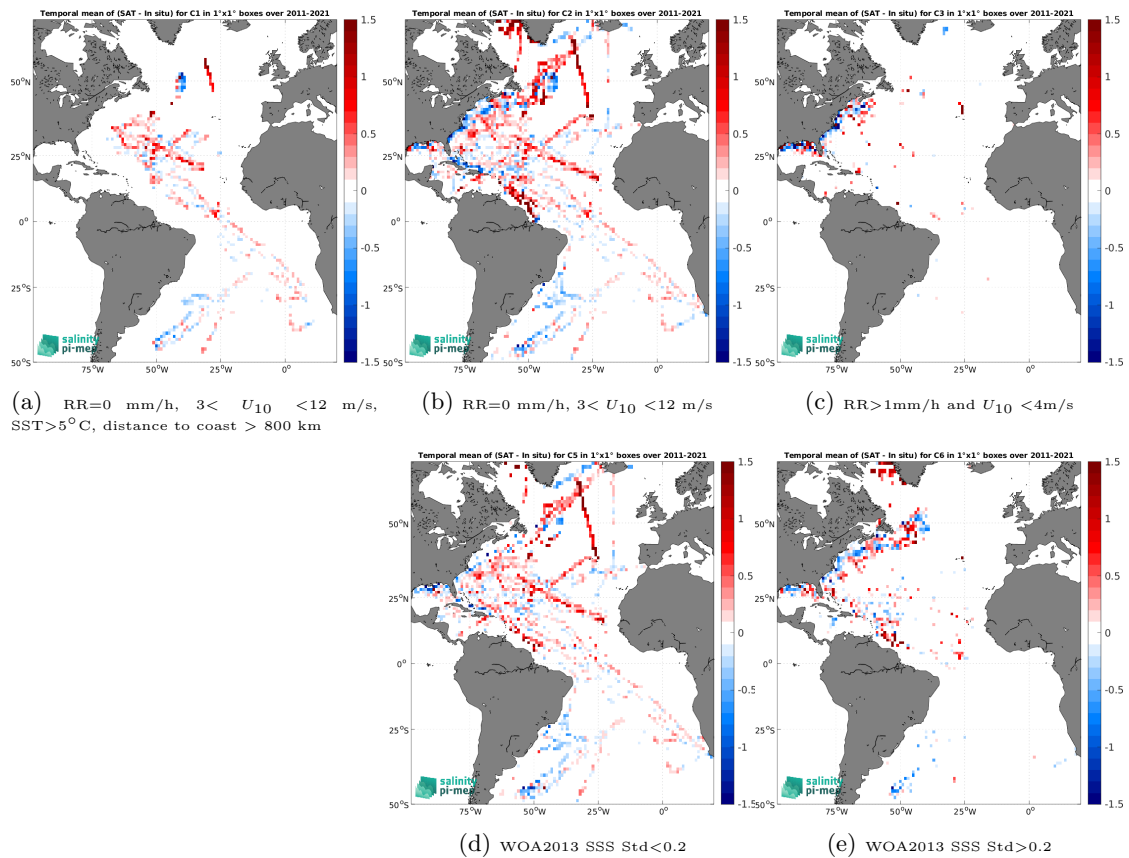
Figure 14: Temporal mean gridded over spatial boxes of size 1^\circ \times 1^\circ of \Delta\text{SSS} (SMOS SSS L3 v2 - 9-Days (BEC) - TSG (SAMOS)) for 5 different subdatasets corresponding to:RR=0 mm/h, 3 < U_{10} < 12 m/s, SST >5^\circ\text{C} , distance to coast > 800 km (a), RR=0 mm/h, 3 < U_{10} < 12 m/s (b), RR >1 mm/h and U_{10} < 4 m/s (c), WOA2013 SSS Std <0.2 (d), WOA2013 SSS Std >0.2 (e).
