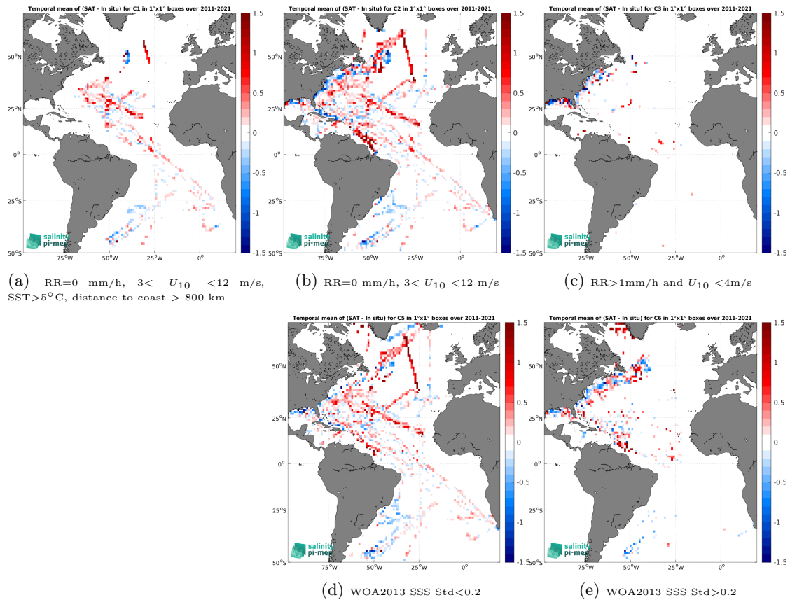
Figure 12: Temporal mean gridded over spatial boxes of size 1^\circ \times 1^\circ of \Delta SSS (SMOS SSS L3 v2 - 9-Days (BEC) - TSG (SAMOS)) for 5 different subdatasets corresponding to:RR=0 mm/h, 3 < U_{10} < 12 m/s, SST >5^\circ\text{C} , distance to coast > 800 km (a), RR=0 mm/h, 3 < U_{10} < 12 m/s (b), RR >1 mm/h and U_{10} < 4 m/s (c), WOA2013 SSS Std <0.2 (d), WOA2013 SSS Std >0.2 (e).
