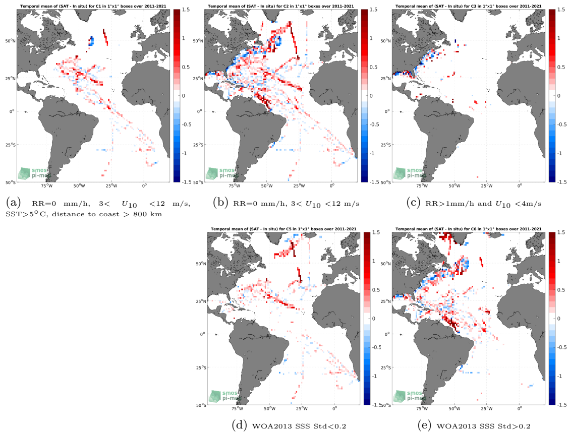
Figure 12: Temporal mean gridded over spatial boxes of size 1^\circ \times 1^\circ of \Delta\text{SSS} (SMOS SSS L3 v2 - 9-Days (BEC) - TSG (SAMOS)) for 5 different subdatasets corresponding to:RR=0 mm/h, 3 < U_{10} < 12 m/s, SST >5^\circ\text{C} , distance to coast > 800 km (a), RR=0 mm/h, 3 < U_{10} < 12 m/s (b), RR >1 mm/h and U_{10} < 4 m/s (c), WOA2013 SSS Std <0.2 (d), WOA2013 SSS Std >0.2 (e).
