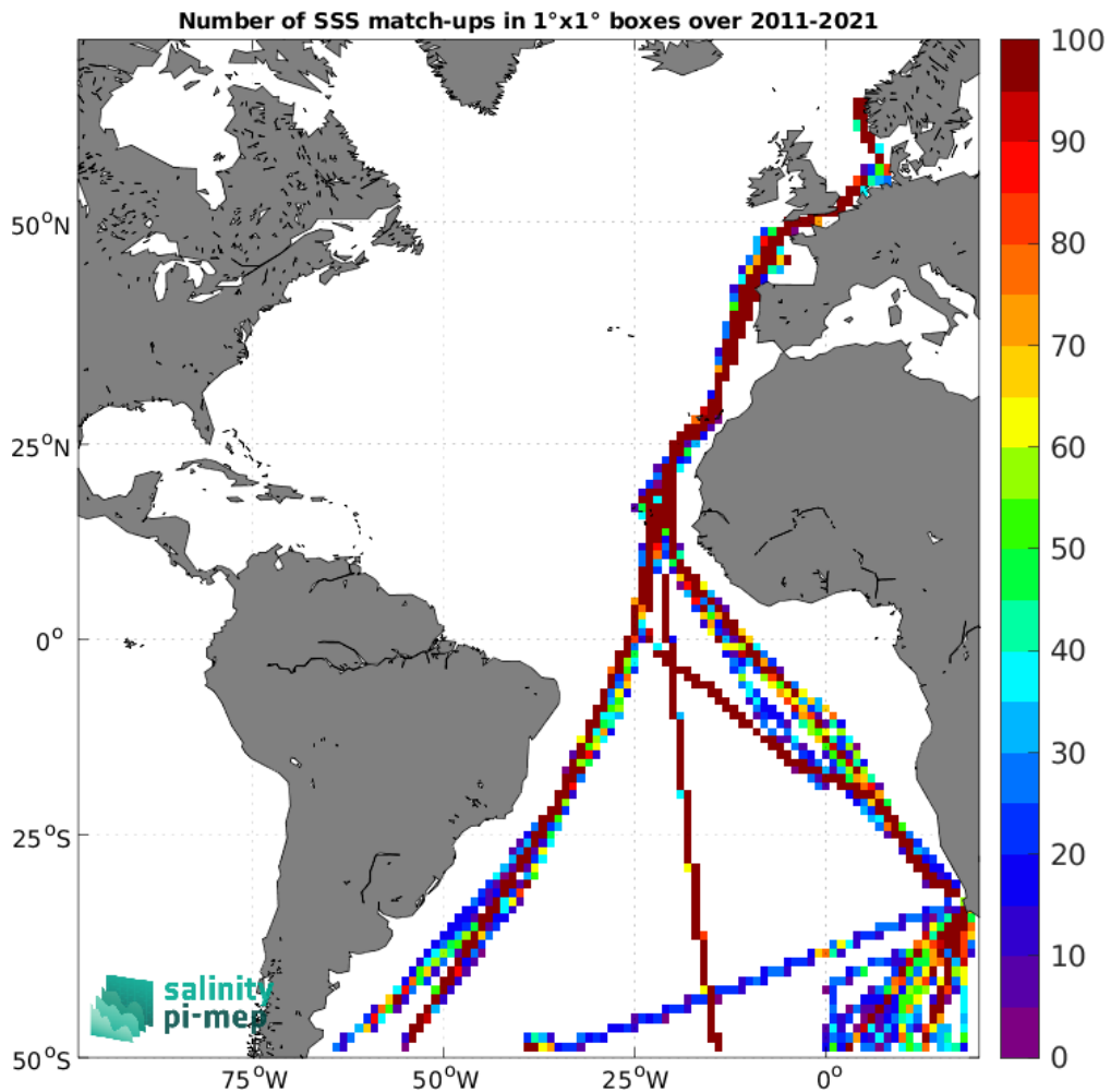
Figure 4: Number of SSS match-ups between TSG (Polarstern) SSS and the SMOS SSS L3 v2 - 9-Days (BEC) SSS product for the Atlantic Ocean Pi-MEP region over 1°×1° boxes and for the full satellite product period.
