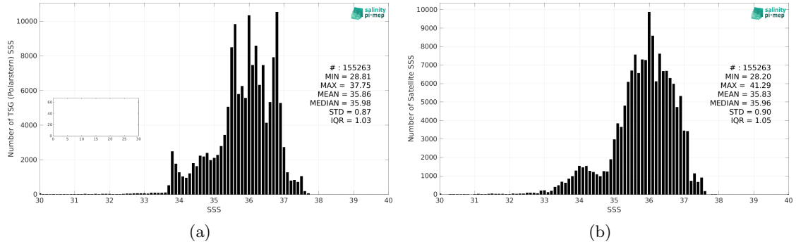
Figure 2: Histograms of SSS from TSG (Polarstern) (a) and SMOS SSS L3 v2 - 9-Days (BEC) (b) considering all match-up pairs per bins of 0.1 over the Atlantic Ocean Pi-MEP region and for the full satellite product period.
