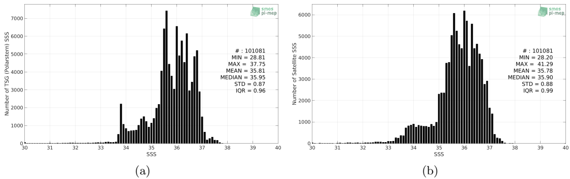
Figure 2: Histograms of SSS from TSG (Polarstern) (a) and SMOS L3 v2 - 9-Days (BEC) (b) considering all match-up pairs per bins of 0.1 over the Atlantic Ocean Pi-MEP region and for the full satellite product period.
