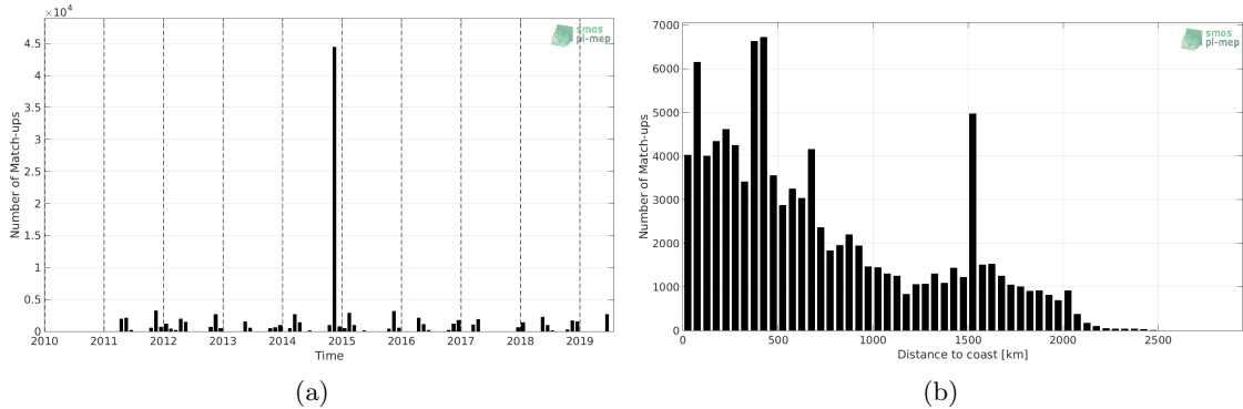
Figure 1: Number of match-ups between TSG (Polarstern) and SMOS L3 v2 - 9-Days (BEC) SSS as a function of time (a) and as function of the distance to coast (b) over the Atlantic Ocean Pi-MEP region and for the full satellite product period.
