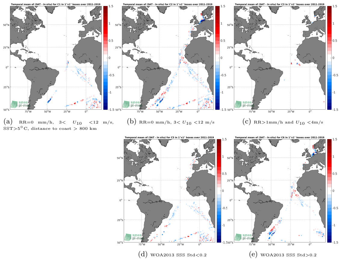
Figure 12: Temporal mean gridded over spatial boxes of size 1^\circ \times 1^\circ of \Delta SSS (SMOS L3 v2 - 9-Days (BEC) - TSG (Polarstern)) for 5 different subdatasets corresponding to:RR=0 mm/h, 3 < U_{10} < 12 m/s, SST >5^\circ\text{C} , distance to coast > 800 km (a), RR=0 mm/h, 3 < U_{10} < 12 m/s (b), RR >1 mm/h and U_{10} < 4 m/s (c), WOA2013 SSS Std <0.2 (d), WOA2013 SSS Std >0.2 (e).
