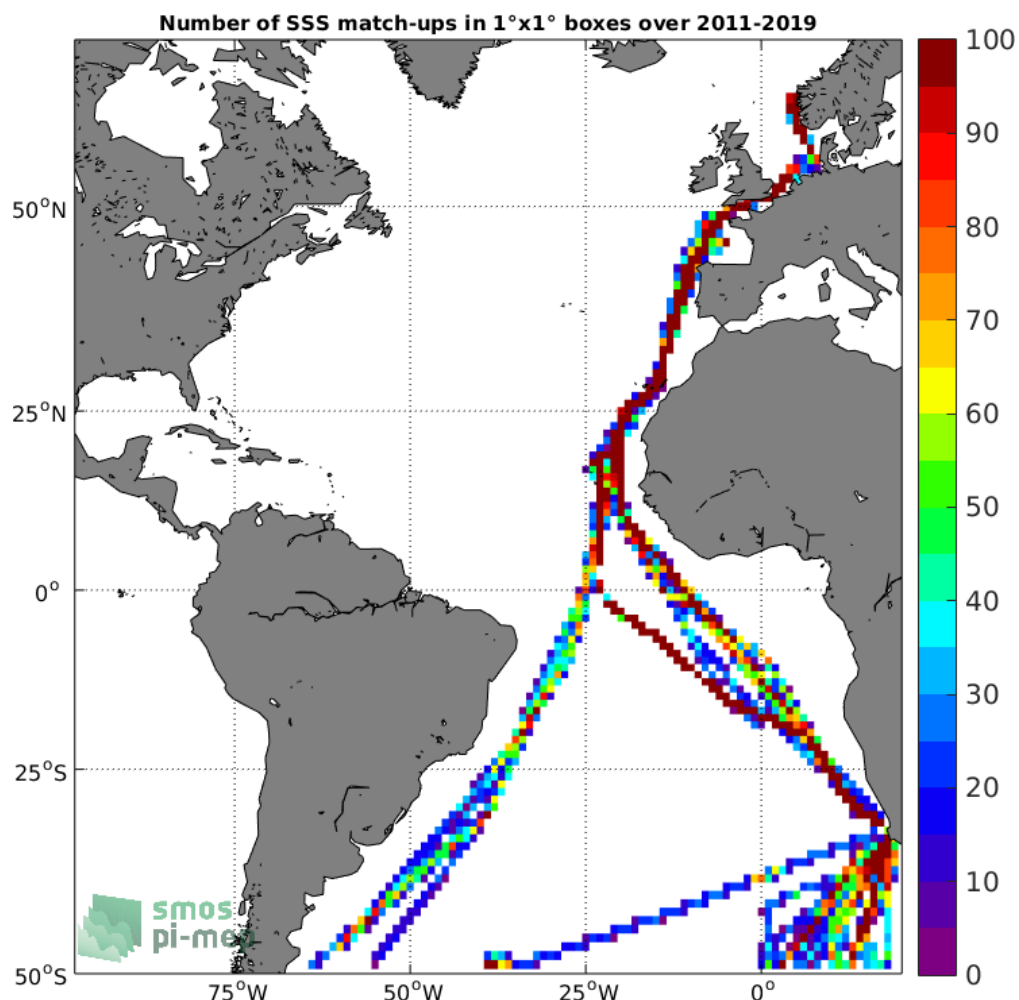
Figure 4: Number of SSS match-ups between TSG (Polarstern) SSS and the SMOS L3 v2 - 9-Days (BEC) SSS product for the Atlantic Ocean Pi-MEP region over 1°x1° boxes and for the full satellite product period.
