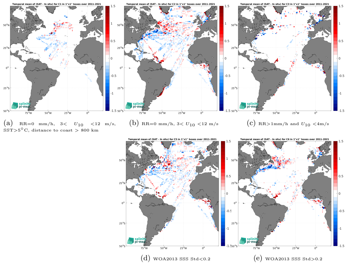
Figure 14: Temporal mean gridded over spatial boxes of size 1^\circ \times 1^\circ of \Delta\text{SSS} (SMOS SSS L3 v2 - 9-Days (BEC) - TSG (LEGOS-DM)) for 5 different subdatasets corresponding to:RR=0 mm/h, 3 < U_{10} < 12 m/s, SST>5°C, distance to coast > 800 km (a), RR=0 mm/h, 3 < U_{10} < 12 m/s (b), RR>1mm/h and U_{10} < 4 m/s (c), WOA2013 SSS Std<0.2 (d), WOA2013 SSS Std>0.2 (e).
