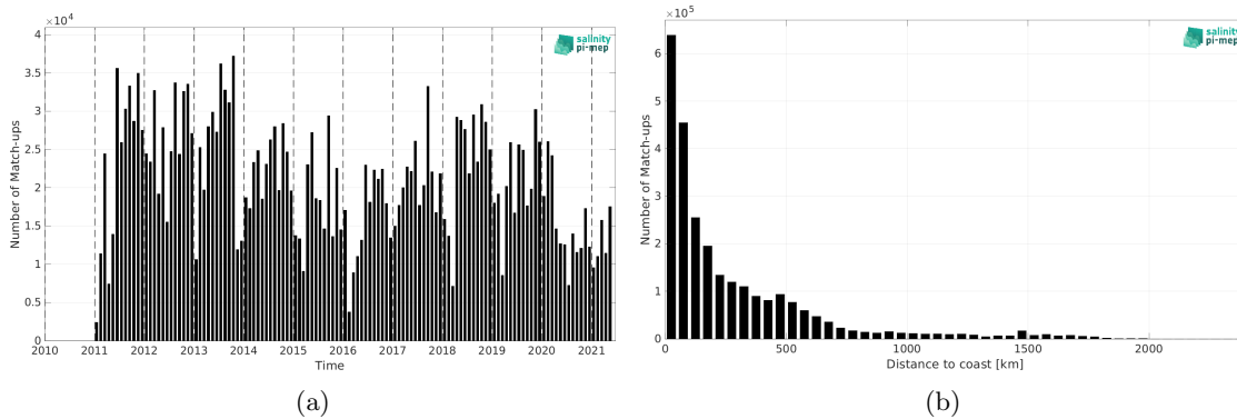
Figure 2: Number of match-ups between TSG (LEGOS-DM) and SMOS SSS L3 v2 - 9-Days (BEC) SSS as a function of time (a) and as function of the distance to coast (b) over the Atlantic Ocean Pi-MEP region and for the full satellite product period.
