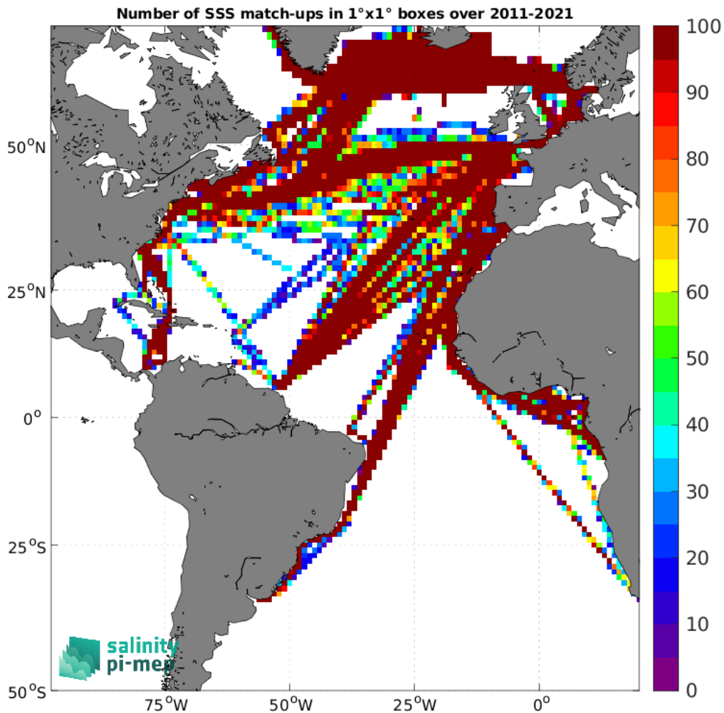
Figure 5: Number of SSS match-ups between TSG (LEGOS-DM) SSS and the SMOS SSS L3 v2 - 9-Days (BEC) SSS product for the Atlantic Ocean Pi-MEP region over 1^\circ \times 1^\circ boxes and for the full satellite product period.
