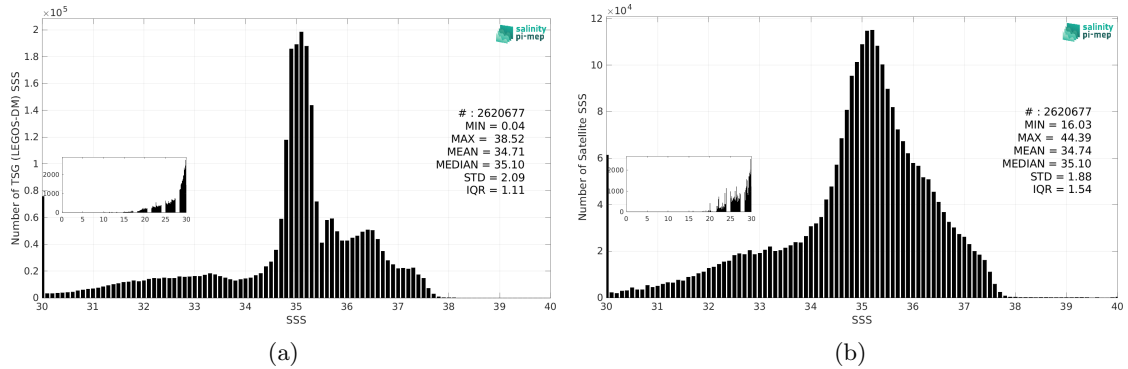
Figure 3: Histograms of SSS from TSG (LEGOS-DM) (a) and SMOS SSS L3 v2 - 9-Days (BEC) (b) considering all match-up pairs per bins of 0.1 over the Atlantic Ocean Pi-MEP region and for the full satellite product period.
