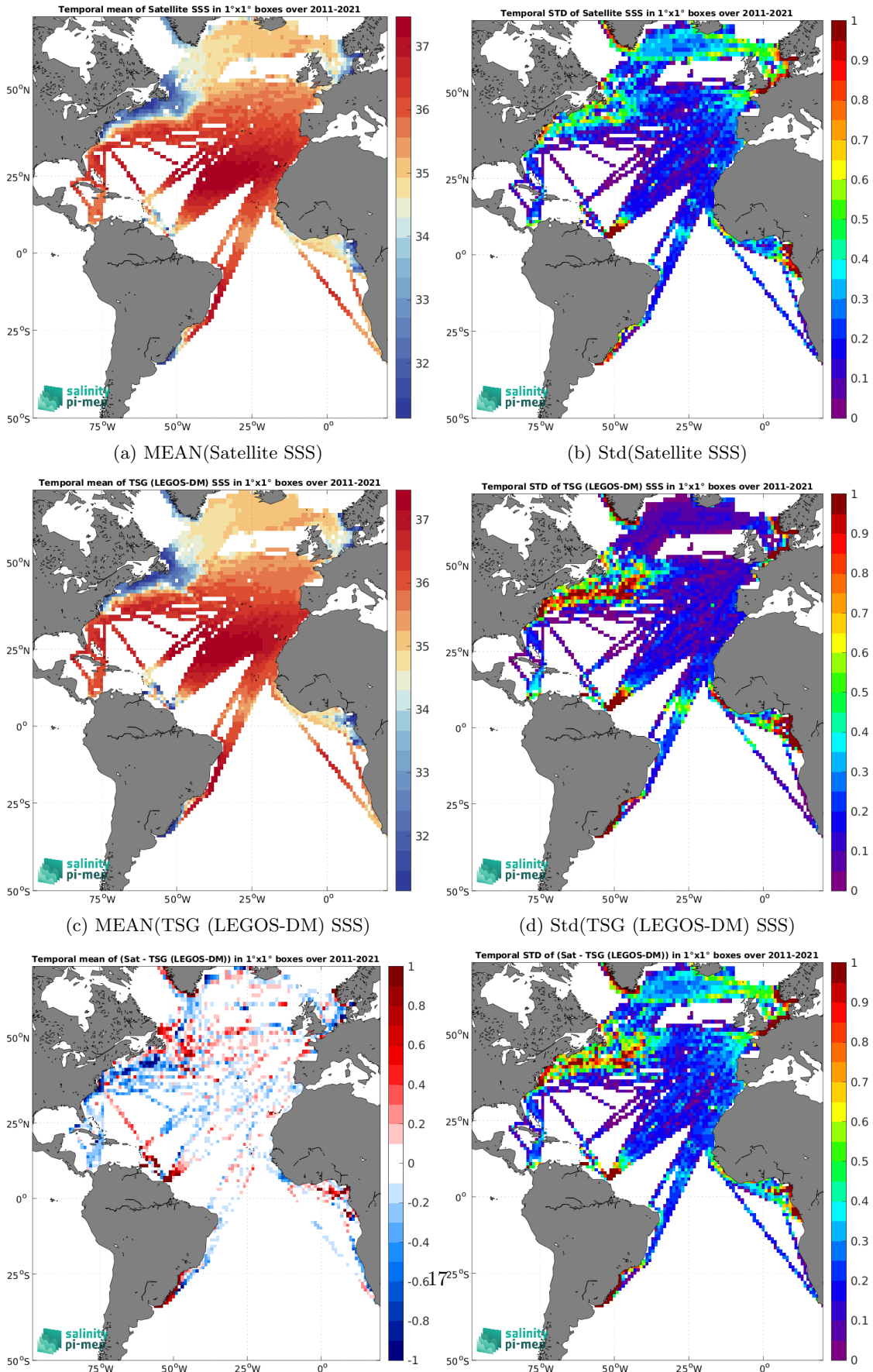
(e) MEAN( \Delta SSS) (Satellite - TSG (LEGOS-DM)) (f) Std( \Delta SSS) (Satellite - TSG (LEGOS-DM)) Figure 7: Temporal mean (left) and Std (right) of SSS from SMOS SSS L3 v2 - 9-Days (BEC) (top), TSG (LEGOS-DM) (middle), and of \Delta SSS (Satellite - TSG (LEGOS-DM)). Only match-pairs are used to generate these maps.
