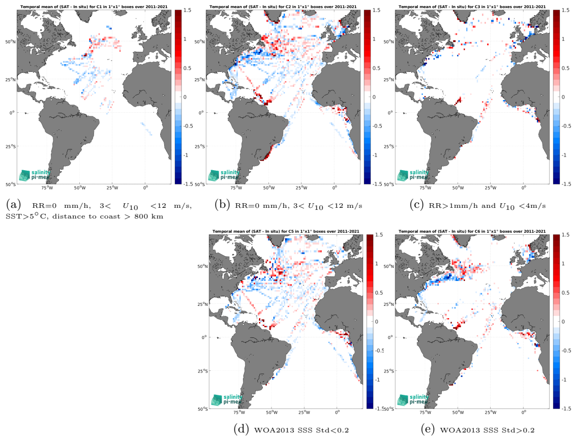
Figure 14: Temporal mean gridded over spatial boxes of size 1^\circ \times 1^\circ of \Delta SSS (SMOS SSS L3 v2 - 9-Days (BEC) - TSG (LEGOS-DM)) for 5 different subdatasets corresponding to:RR=0 mm/h, 3 < U_{10} < 12 m/s, SST >5^\circ\text{C} , distance to coast > 800 km (a), RR=0 mm/h, 3 < U_{10} < 12 m/s (b), RR >1 mm/h and U_{10} < 4 m/s (c), WOA2013 SSS Std <0.2 (d), WOA2013 SSS Std >0.2 (e).
