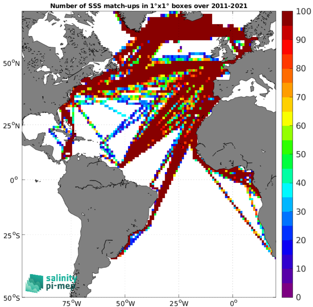
Figure 4: Number of SSS match-ups between TSG (LEGOS-DM) SSS and the SMOS SSS L3 v2 - 9-Days (BEC) SSS product for the Atlantic Ocean Pi-MEP region over 1°×1° boxes and for the full satellite product period.
