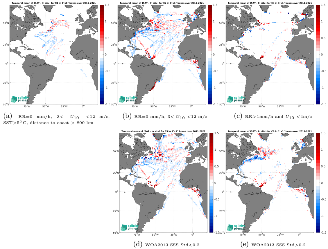
Figure 12: Temporal mean gridded over spatial boxes of size 1^\circ \times 1^\circ of \Delta SSS (SMOS SSS L3 v2 - 9-Days (BEC) - TSG (LEGOS-DM)) for 5 different subdatasets corresponding to:RR=0 mm/h, 3 < U_{10} < 12 m/s, SST >5^\circ\text{C} , distance to coast > 800 km (a), RR=0 mm/h, 3 < U_{10} < 12 m/s (b), RR >1 mm/h and U_{10} < 4 m/s (c), WOA2013 SSS Std <0.2 (d), WOA2013 SSS Std >0.2 (e).
