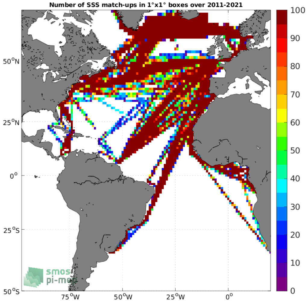
Figure 4: Number of SSS match-ups between TSG (LEGOS-DM) SSS and the SMOS SSS L3 v2 - 9-Days (BEC) SSS product for the Atlantic Ocean Pi-MEP region over 1°x1° boxes and for the full satellite product period.
