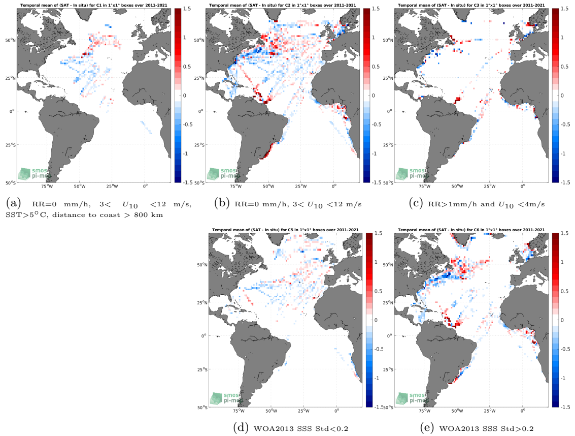
Figure 12: Temporal mean gridded over spatial boxes of size 1^\circ \times 1^\circ of \Delta SSS (SMOS SSS L3 v2 - 9-Days (BEC) - TSG (LEGOS-DM)) for 5 different subdatasets corresponding to:RR=0 mm/h, 3 < U_{10} < 12 m/s, SST >5^\circ\text{C} , distance to coast > 800 km (a), RR=0 mm/h, 3 < U_{10} < 12 m/s (b), RR >1 mm/h and U_{10} < 4 m/s (c), WOA2013 SSS Std <0.2 (d), WOA2013 SSS Std >0.2 (e).
