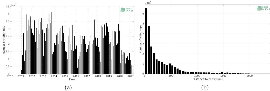
Figure 1: Number of match-ups between TSG (LEGOS-DM) and SMOS SSS L3 v2 - 9-Days (BEC) SSS as a function of time (a) and as function of the distance to coast (b) over the Atlantic Ocean Pi-MEP region and for the full satellite product period.
