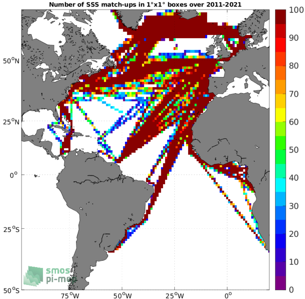
Figure 4: Number of SSS match-ups between TSG (LEGOS-DM) SSS and the SMOS SSS L3 v2 - 9-Days (BEC) SSS product for the Atlantic Ocean Pi-MEP region over 1^\circ \times 1^\circ boxes and for the full satellite product period.
