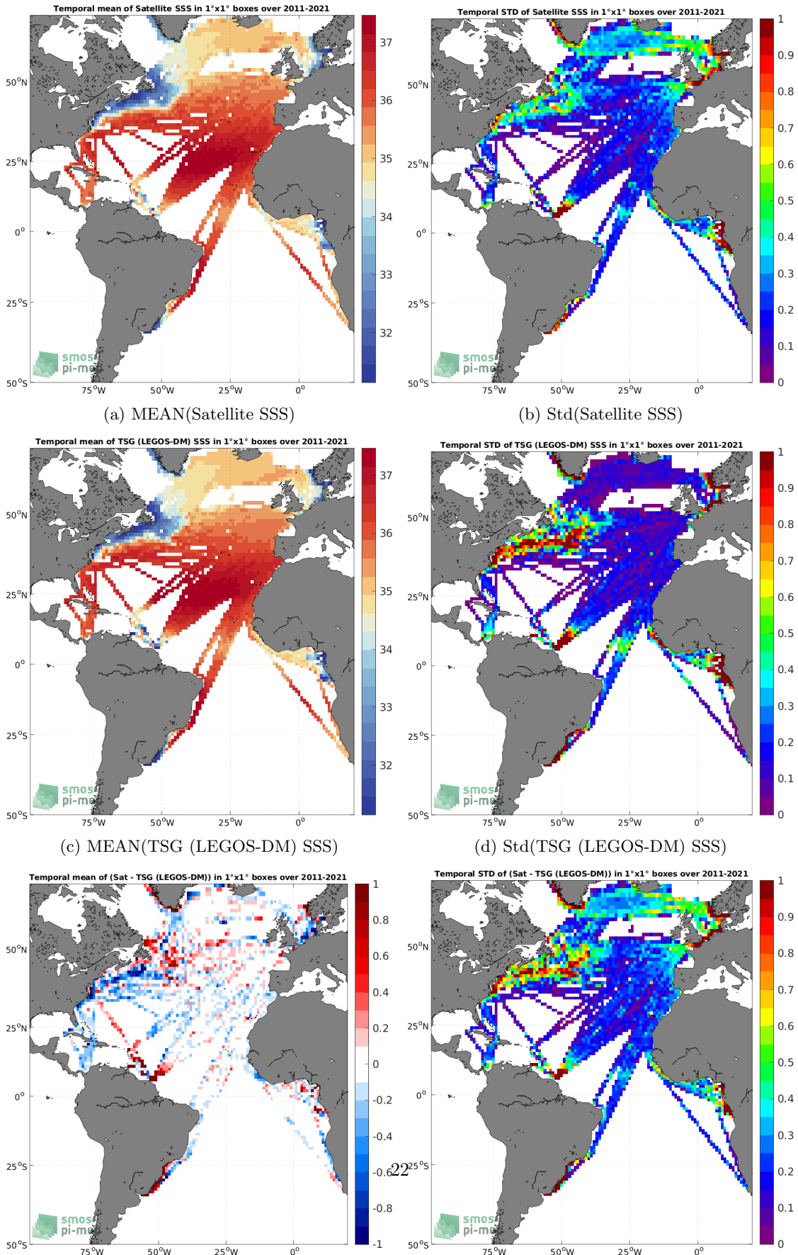
(e) MEAN( \Delta SSS) (Satellite - TSG (LEGOS-DM)) (f) Std( \Delta SSS) (Satellite - TSG (LEGOS-DM)) Figure 6: Temporal mean (left) and Std (right) of SSS from SMOS SSS L3 v2 - 9-Days (BEC) (top), TSG (LEGOS-DM) (middle), and of \Delta SSS (Satellite - TSG (LEGOS-DM)). Only match-up pairs are used to generate these maps.
