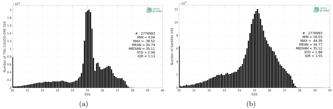
Figure 2: Histograms of SSS from TSG (LEGOS-DM) (a) and SMOS SSS L3 v2 - 9-Days (BEC) (b) considering all match-up pairs per bins of 0.1 over the Atlantic Ocean Pi-MEP region and for the full satellite product period.
