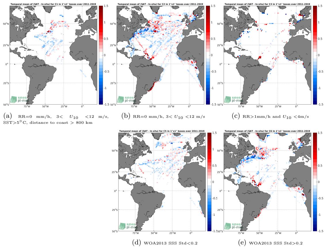
Figure 12: Temporal mean gridded over spatial boxes of size 1^\circ \times 1^\circ of \Delta\text{SSS} (SMOS SSS L3 v2 - 9-Days (BEC) - TSG (LEGOS-DM)) for 5 different subdatasets corresponding to:RR=0 mm/h, 3 < U_{10} < 12 m/s, SST>5°C, distance to coast > 800 km (a), RR=0 mm/h, 3 < U_{10} < 12 m/s (b), RR>1mm/h and U_{10} < 4 m/s (c), WOA2013 SSS Std<0.2 (d), WOA2013 SSS Std>0.2 (e).
