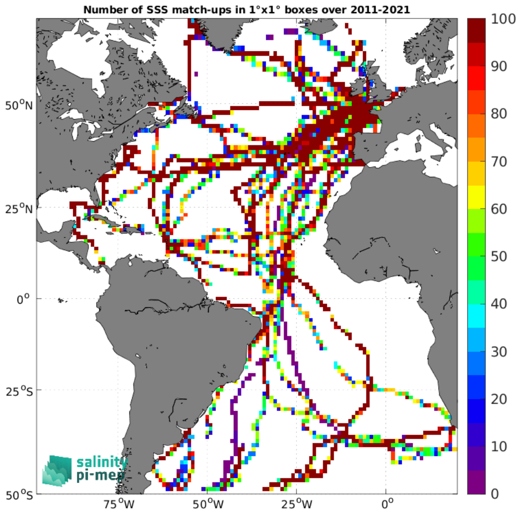
Figure 5: Number of SSS match-ups between TSG (GOSUD-Sailing-ship) SSS and the SMOS SSS L3 v2 - 9-Days (BEC) SSS product for the Atlantic Ocean Pi-MEP region over 1^\circ \times 1^\circ boxes and for the full satellite product period.
