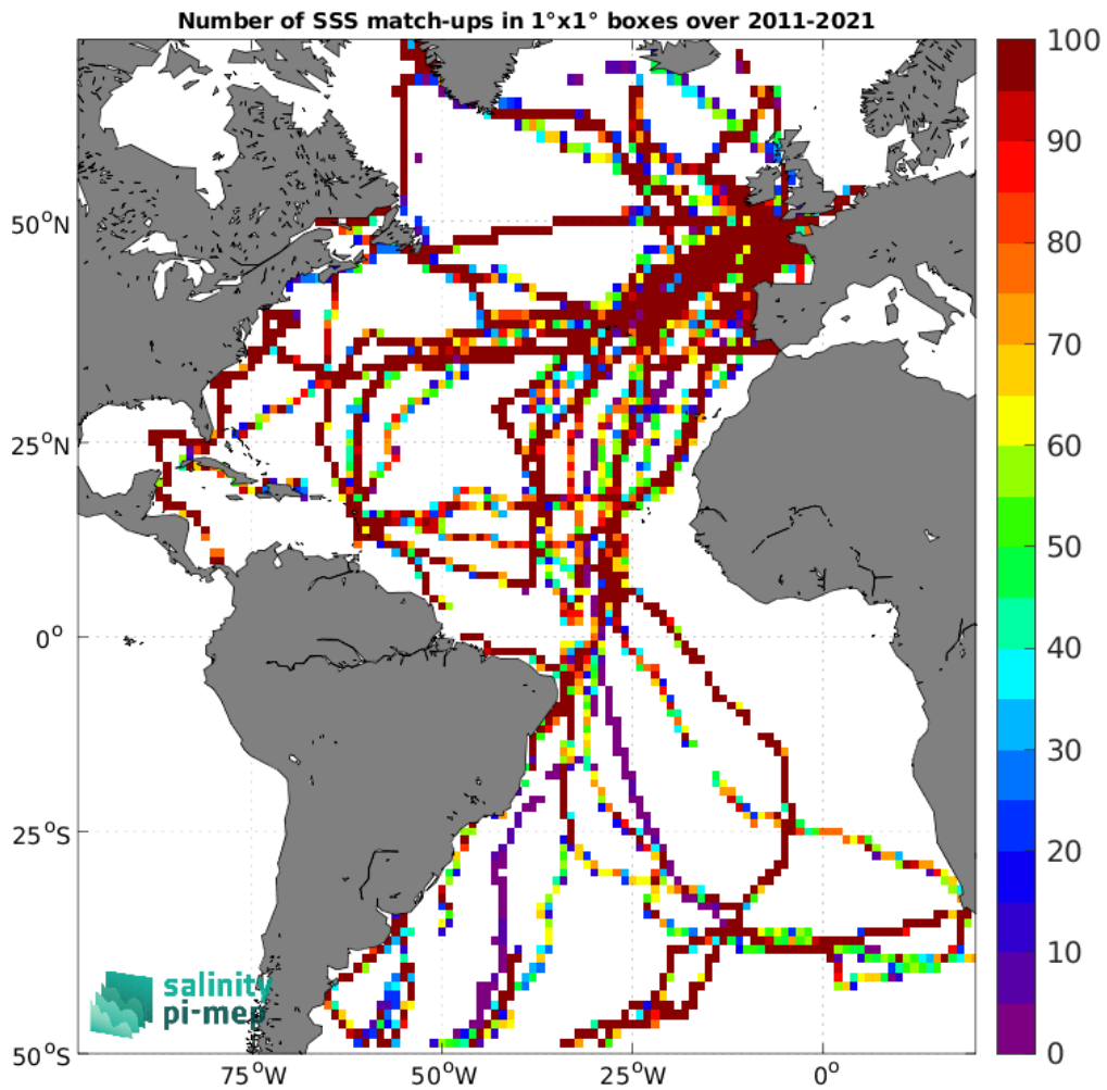
Figure 4: Number of SSS match-ups between TSG (GOSUD-Sailing-ship) SSS and the SMOS SSS L3 v2 - 9-Days (BEC) SSS product for the Atlantic Ocean Pi-MEP region over 1°x1° boxes and for the full satellite product period.
