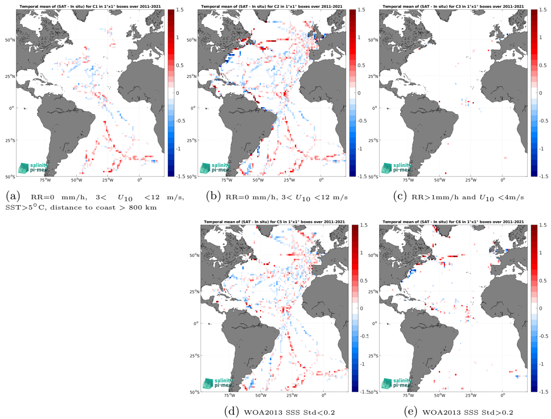
Figure 12: Temporal mean gridded over spatial boxes of size 1^\circ \times 1^\circ of \Delta\text{SSS} (SMOS SSS L3 v2 - 9-Days (BEC) - TSG (GOSUD-Sailing-ship)) for 5 different subdatasets corresponding to:RR=0 mm/h, 3 < U_{10} < 12 m/s, SST>5°C, distance to coast > 800 km (a), RR=0 mm/h, 3 < U_{10} < 12 m/s (b), RR>1mm/h and U_{10} < 4 m/s (c), WOA2013 SSS Std<0.2 (d), WOA2013 SSS Std>0.2 (e).
