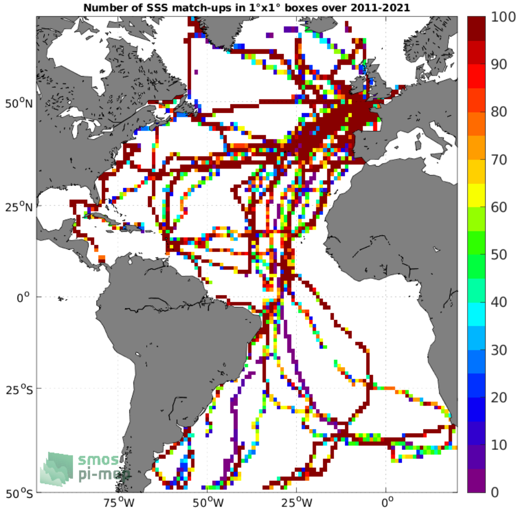
Figure 4: Number of SSS match-ups between TSG (GOSUD-Sailing-ship) SSS and the SMOS SSS L3 v2 - 9-Days (BEC) SSS product for the Atlantic Ocean Pi-MEP region over 1^\circ \times 1^\circ boxes and for the full satellite product period.
