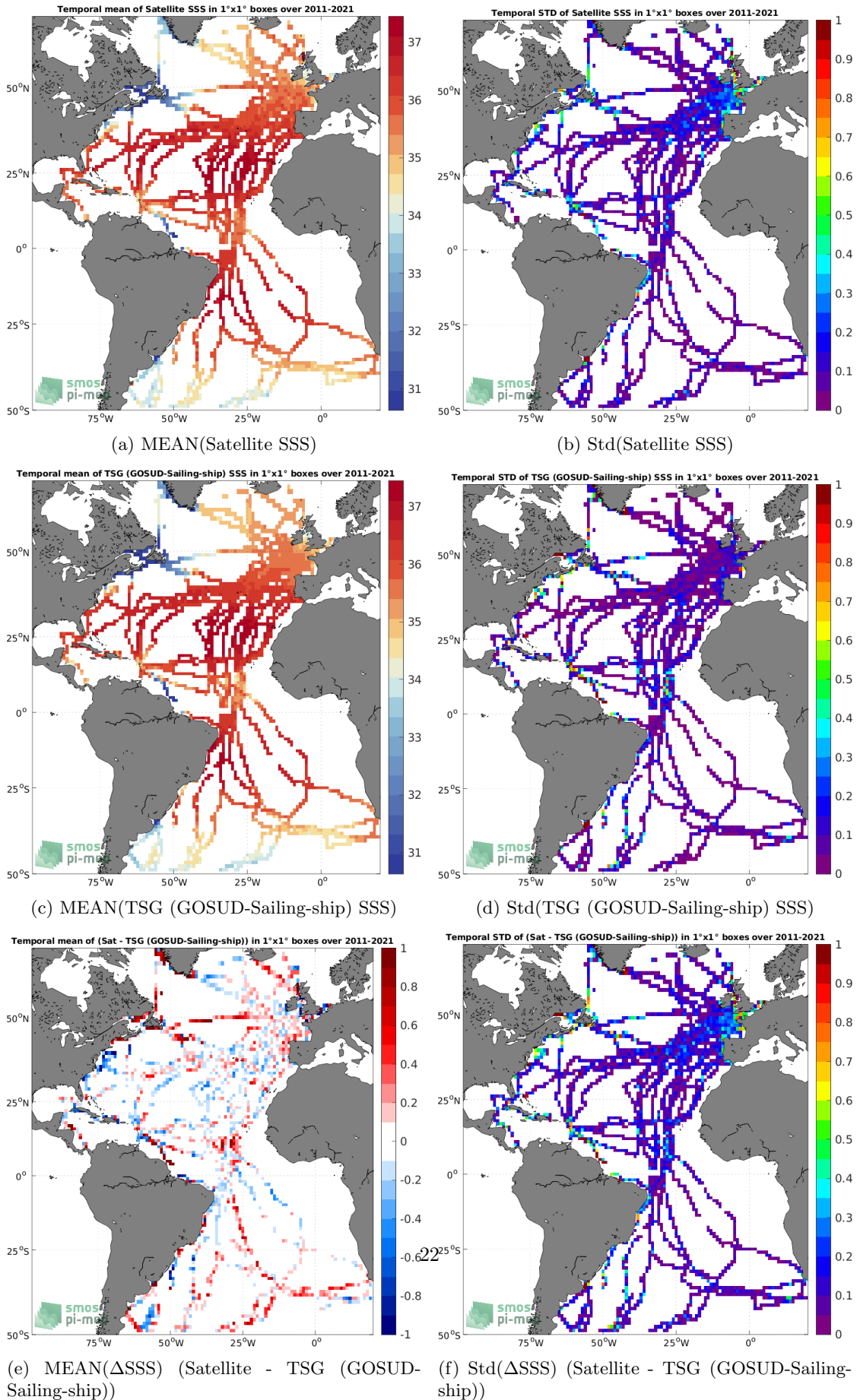
Figure 6: Temporal mean (left) and Std (right) of SSS from SMOS SSS L3 v2 - 9-Days (BEC) (top), TSG (GOSUD-Sailing-ship) (middle), and of \Delta SSS (Satellite - TSG (GOSUD-Sailing-ship)). Only match-up pairs are used to generate these maps.
