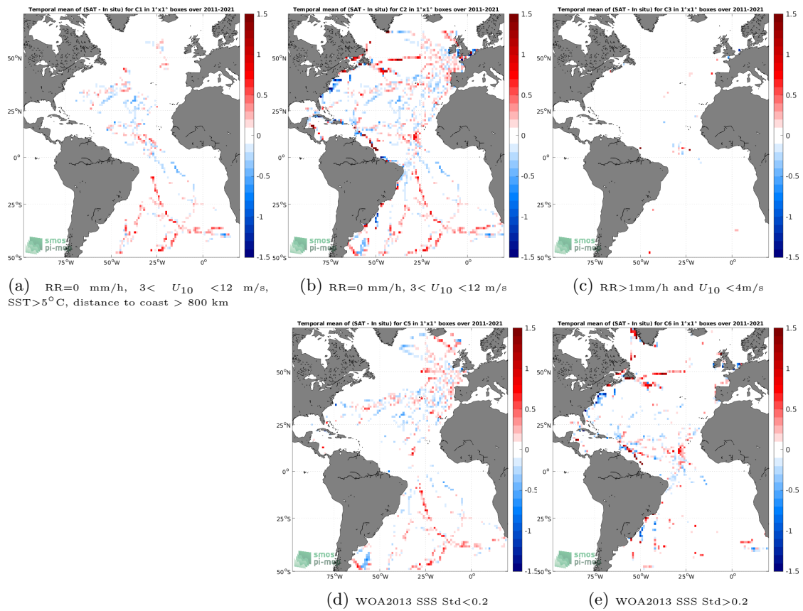
Figure 12: Temporal mean gridded over spatial boxes of size 1^\circ \times 1^\circ of \Delta SSS (SMOS SSS L3 v2 - 9-Days (BEC) - TSG (GOSUD-Sailing-ship)) for 5 different subdatasets corresponding to:RR=0 mm/h, 3 < U_{10} < 12 m/s, SST>5°C, distance to coast > 800 km (a), RR=0 mm/h, 3 < U_{10} < 12 m/s (b), RR>1mm/h and U_{10} < 4 m/s (c), WOA2013 SSS Std<0.2 (d), WOA2013 SSS Std>0.2 (e).
