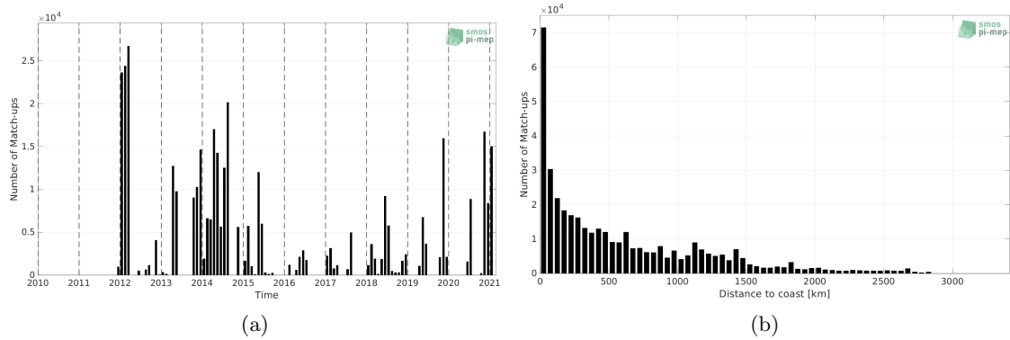
Figure 1: Number of match-ups between TSG (GOSUD-Sailing-ship) and SMOS SSS L3 v2 - 9-Days (BEC) SSS as a function of time (a) and as function of the distance to coast (b) over the Atlantic Ocean Pi-MEP region and for the full satellite product period.
