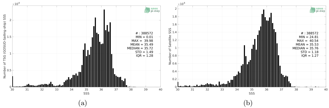
Figure 2: Histograms of SSS from TSG (GOSUD-Sailing-ship) (a) and SMOS SSS L3 v2 - 9-Days (BEC) (b) considering all match-up pairs per bins of 0.1 over the Atlantic Ocean Pi-MEP region and for the full satellite product period.
