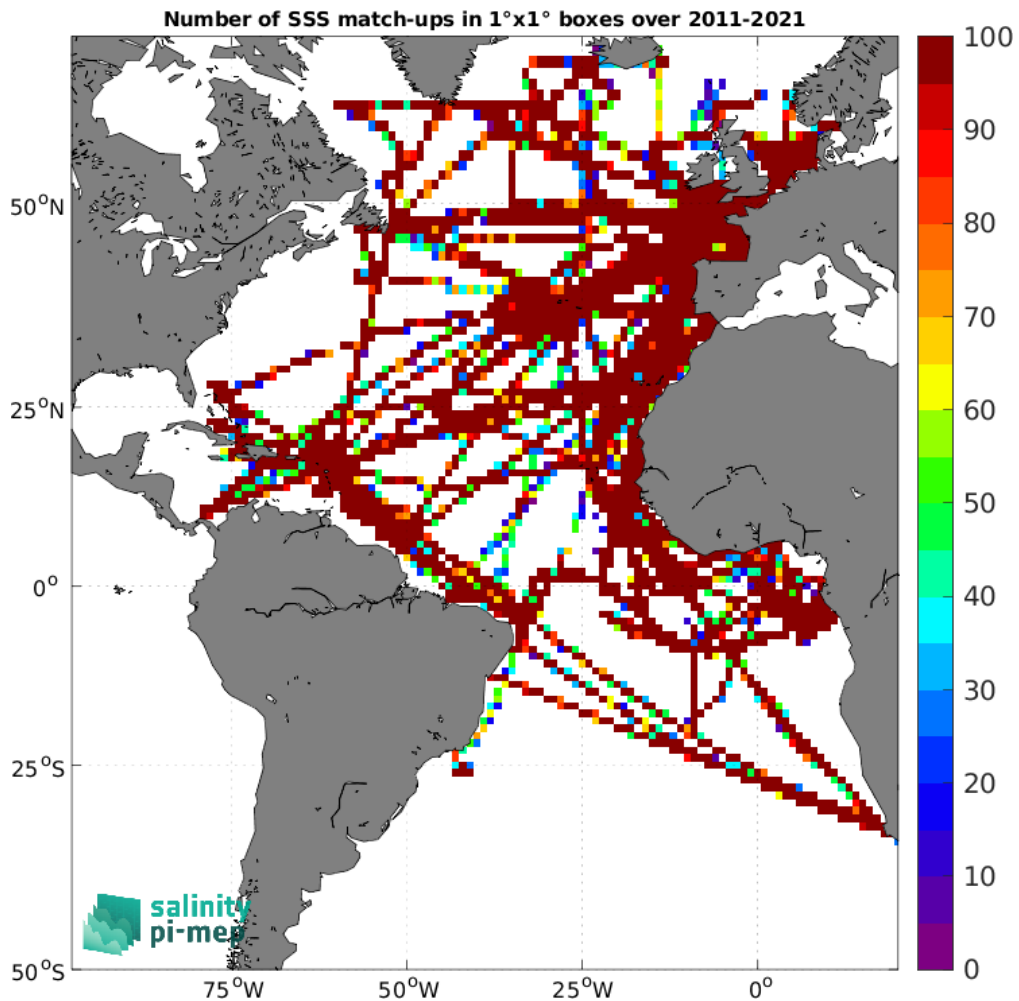
Figure 5: Number of SSS match-ups between TSG (GOSUD-Research-vessel) SSS and the SMOS SSS L3 v2 - 9-Days (BEC) SSS product for the Atlantic Ocean Pi-MEP region over 1°x1° boxes and for the full satellite product period.
