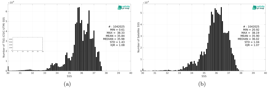
Figure 2: Histograms of SSS from TSG (CSIC-UTM) (a) and SMOS SSS L3 v2 - 9-Days (BEC) (b) considering all match-up pairs per bins of 0.1 over the Atlantic Ocean Pi-MEP region and for the full satellite product period.
