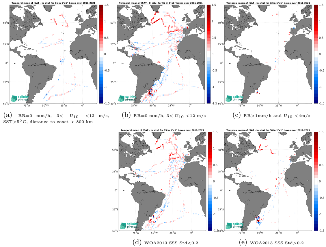
Figure 12: Temporal mean gridded over spatial boxes of size 1^\circ \times 1^\circ of \Delta SSS (SMOS SSS L3 v2 - 9-Days (BEC) - TSG (CSIC-UTM)) for 5 different subdatasets corresponding to:RR=0 mm/h, 3 < U_{10} < 12 m/s, SST >5^\circ\text{C} , distance to coast > 800 km (a), RR=0 mm/h, 3 < U_{10} < 12 m/s (b), RR >1 mm/h and U_{10} < 4 m/s (c), WOA2013 SSS Std <0.2 (d), WOA2013 SSS Std >0.2 (e).
