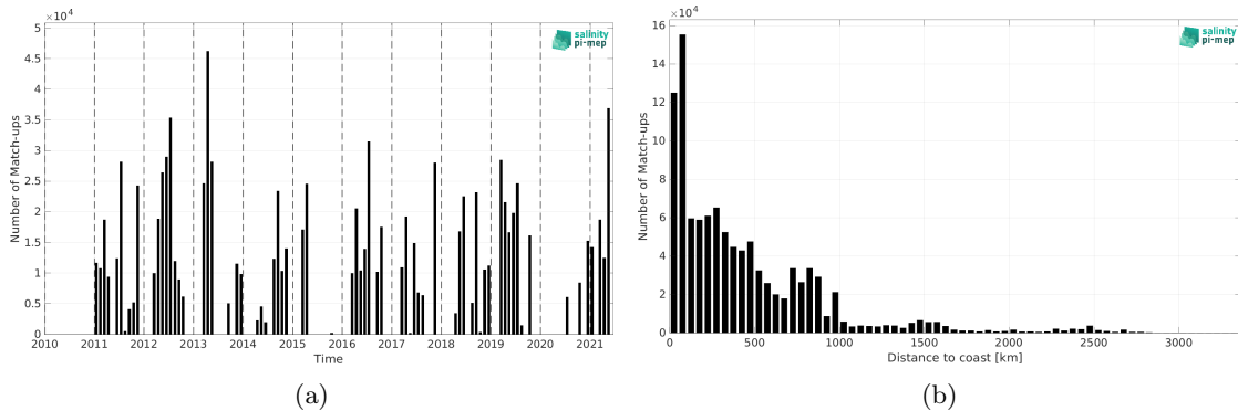
Figure 1: Number of match-ups between TSG (CSIC-UTM) and SMOS SSS L3 v2 - 9-Days (BEC) SSS as a function of time (a) and as function of the distance to coast (b) over the Atlantic Ocean Pi-MEP region and for the full satellite product period.
