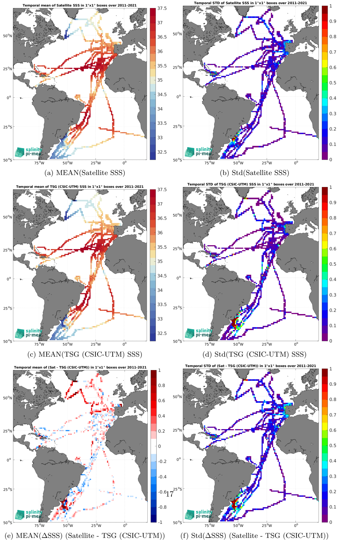
Figure 6: Temporal mean (left) and Std (right) of SSS from SMOS SSS L3 v2 - 9-Days (BEC) (top), TSG (CSIC-UTM) (middle), and of \Delta SSS (Satellite - TSG (CSIC-UTM)). Only match-up pairs are used to generate these maps.
