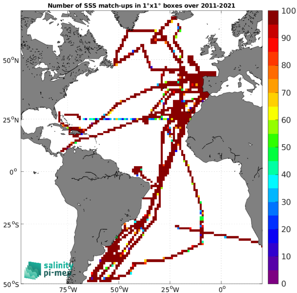
Figure 4: Number of SSS match-ups between TSG (CSIC-UTM) SSS and the SMOS SSS L3 v2 - 9-Days (BEC) SSS product for the Atlantic Ocean Pi-MEP region over 1°×1° boxes and for the full satellite product period.
