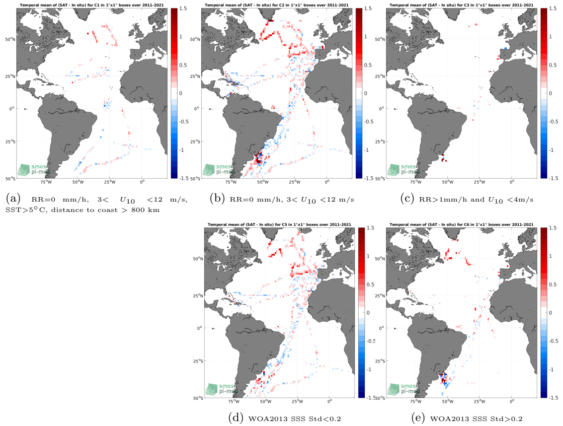
Figure 12: Temporal mean gridded over spatial boxes of size 1^\circ \times 1^\circ of \Delta SSS (SMOS SSS L3 v2 - 9-Days (BEC) - TSG (CSIC-UTM)) for 5 different subdatasets corresponding to:RR=0 mm/h, 3 < U_{10} < 12 m/s, SST >5^\circ\text{C} , distance to coast > 800 km (a), RR=0 mm/h, 3 < U_{10} < 12 m/s (b), RR >1 mm/h and U_{10} < 4 m/s (c), WOA2013 SSS Std <0.2 (d), WOA2013 SSS Std >0.2 (e).
