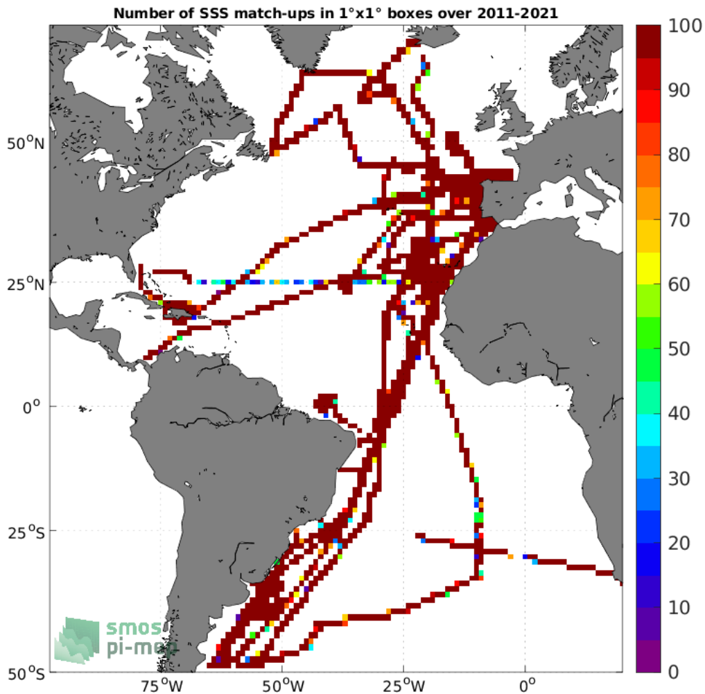
Figure 4: Number of SSS match-ups between TSG (CSIC-UTM) SSS and the SMOS SSS L3 v2 - 9-Days (BEC) SSS product for the Atlantic Ocean Pi-MEP region over 1°x1° boxes and for the full satellite product period.
