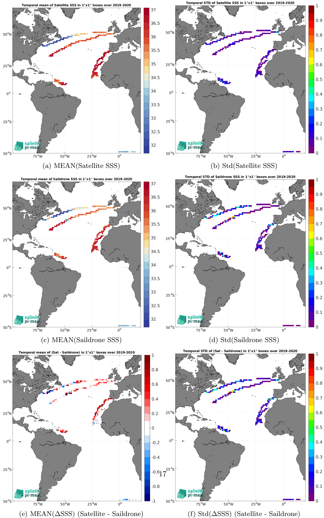
Figure 7: Temporal mean (left) and Std (right) of SSS from SMOS SSS L3 v2 - 9-Days (BEC) (top), Saildrone (middle), and of \Delta SSS (Satellite - Saildrone). Only match-up pairs are used to generate these maps.
