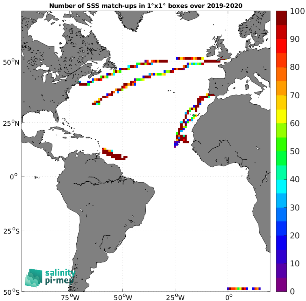
Figure 5: Number of SSS match-ups between Saildrone SSS and the SMOS SSS L3 v2 - 9-Days (BEC) SSS product for the Atlantic Ocean Pi-MEP region over 1^\circ \times 1^\circ boxes and for the full satellite product period.
