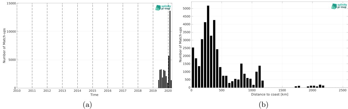
Figure 2: Number of match-ups between Saildrone and SMOS SSS L3 v2 - 9-Days (BEC) SSS as a function of time (a) and as function of the distance to coast (b) over the Atlantic Ocean Pi-MEP region and for the full satellite product period.
