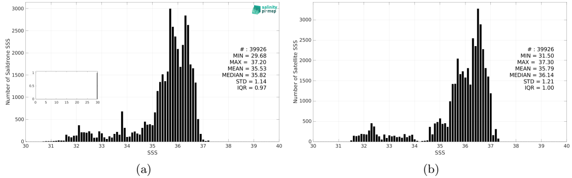
Figure 3: Histograms of SSS from Saildrone (a) and SMOS SSS L3 v2 - 9-Days (BEC) (b) considering all match-up pairs per bins of 0.1 over the Atlantic Ocean Pi-MEP region and for the full satellite product period.
