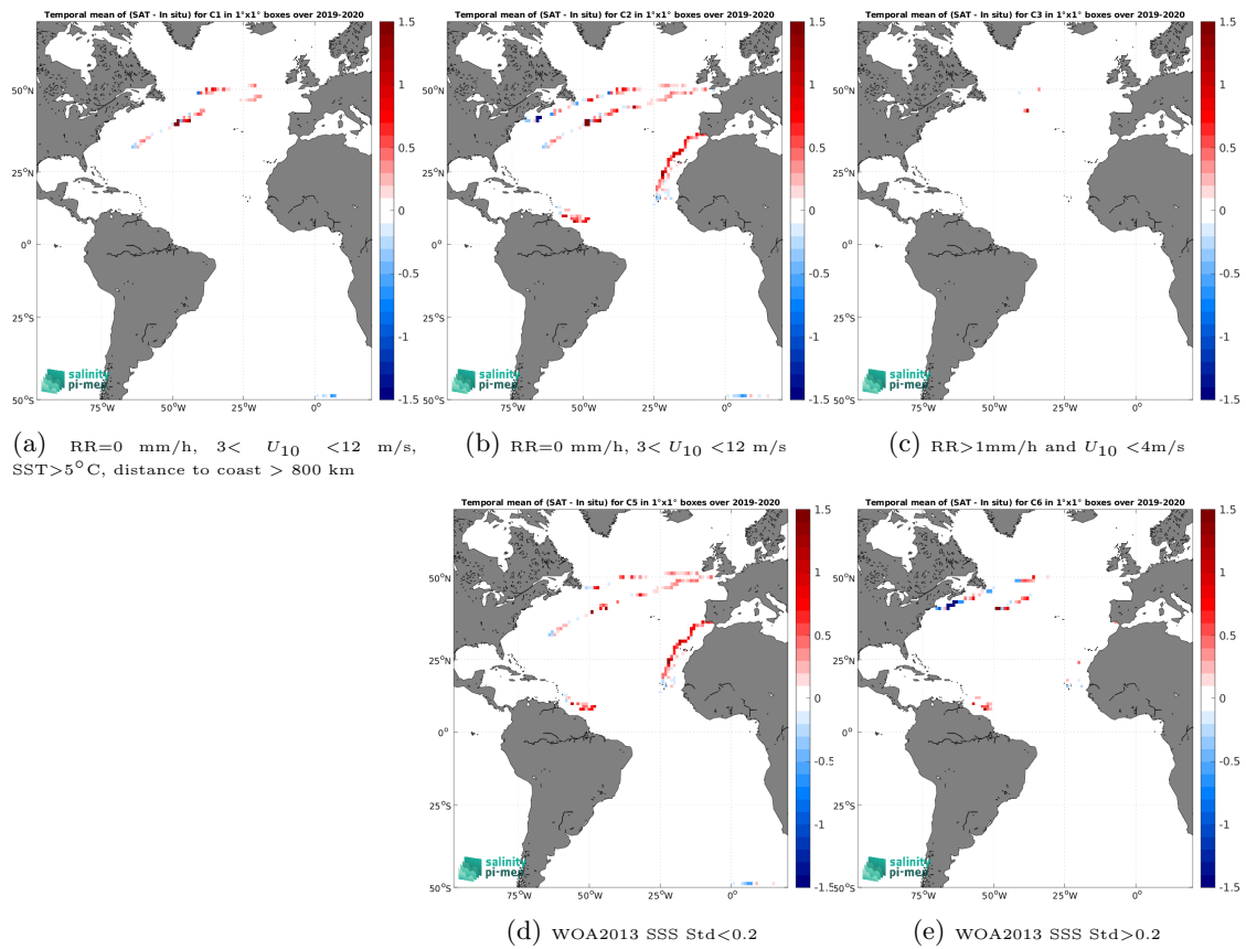
Figure 14: Temporal mean gridded over spatial boxes of size 1^\circ \times 1^\circ of \Delta\text{SSS} (SMOS SSS L3 v2 - 9-Days (BEC) - Saldrone) for 5 different subdatasets corresponding to:RR=0 mm/h, 3 < U_{10} < 12 m/s, SST>5°C, distance to coast > 800 km (a), RR=0 mm/h, 3 < U_{10} < 12 m/s (b), RR>1mm/h and U_{10} < 4 m/s (c), WOA2013 SSS Std<0.2 (d), WOA2013 SSS Std>0.2 (e).
