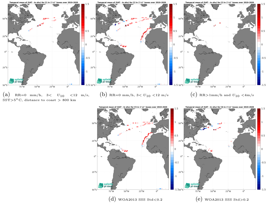
Figure 12: Temporal mean gridded over spatial boxes of size 1^\circ \times 1^\circ of \Delta\text{SSS} (SMOS SSS L3 v2 - 9-Days (BEC) - Sailability) for 5 different subdatasets corresponding to:RR=0 mm/h, 3 < U_{10} < 12 m/s, SST >5^\circ\text{C} , distance to coast > 800 km (a), RR=0 mm/h, 3 < U_{10} < 12 m/s (b), RR >1 mm/h and U_{10} < 4 m/s (c), WOA2013 SSS Std <0.2 (d), WOA2013 SSS Std >0.2 (e).
