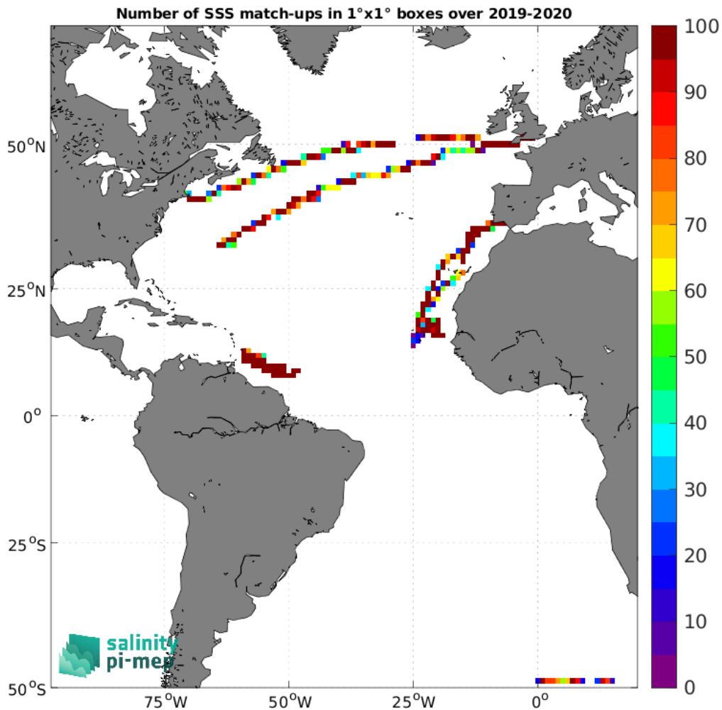
Figure 4: Number of SSS match-ups between Saildrone SSS and the SMOS SSS L3 v2 - 9-Days (BEC) SSS product for the Atlantic Ocean Pi-MEP region over 1°×1° boxes and for the full satellite product period.
