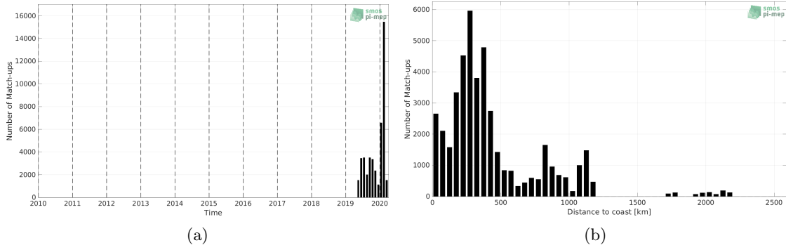
Figure 1: Number of match-ups between Saildrone and SMOS SSS L3 v2 - 9-Days (BEC) SSS as a function of time (a) and as function of the distance to coast (b) over the Atlantic Ocean Pi-MEP region and for the full satellite product period.
