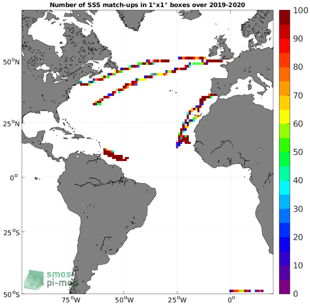
Figure 4: Number of SSS match-ups between Saildrone SSS and the SMOS SSS L3 v2 - 9-Days (BEC) SSS product for the Atlantic Ocean Pi-MEP region over 1^\circ \times 1^\circ boxes and for the full satellite product period.
