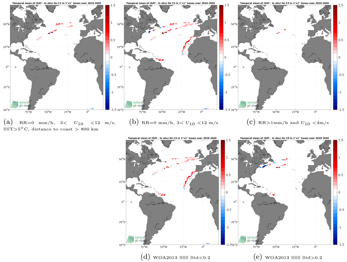
Figure 12: Temporal mean gridded over spatial boxes of size 1^\circ \times 1^\circ of \Delta SSS (SMOS SSS L3 v2 - 9-Days (BEC) - Sailydrone) for 5 different subdatasets corresponding to:RR=0 mm/h, 3 < U_{10} < 12 m/s, SST >5^\circ\text{C} , distance to coast > 800 km (a), RR=0 mm/h, 3 < U_{10} < 12 m/s (b), RR >1 mm/h and U_{10} < 4 m/s (c), WOA2013 SSS Std <0.2 (d), WOA2013 SSS Std >0.2 (e).
