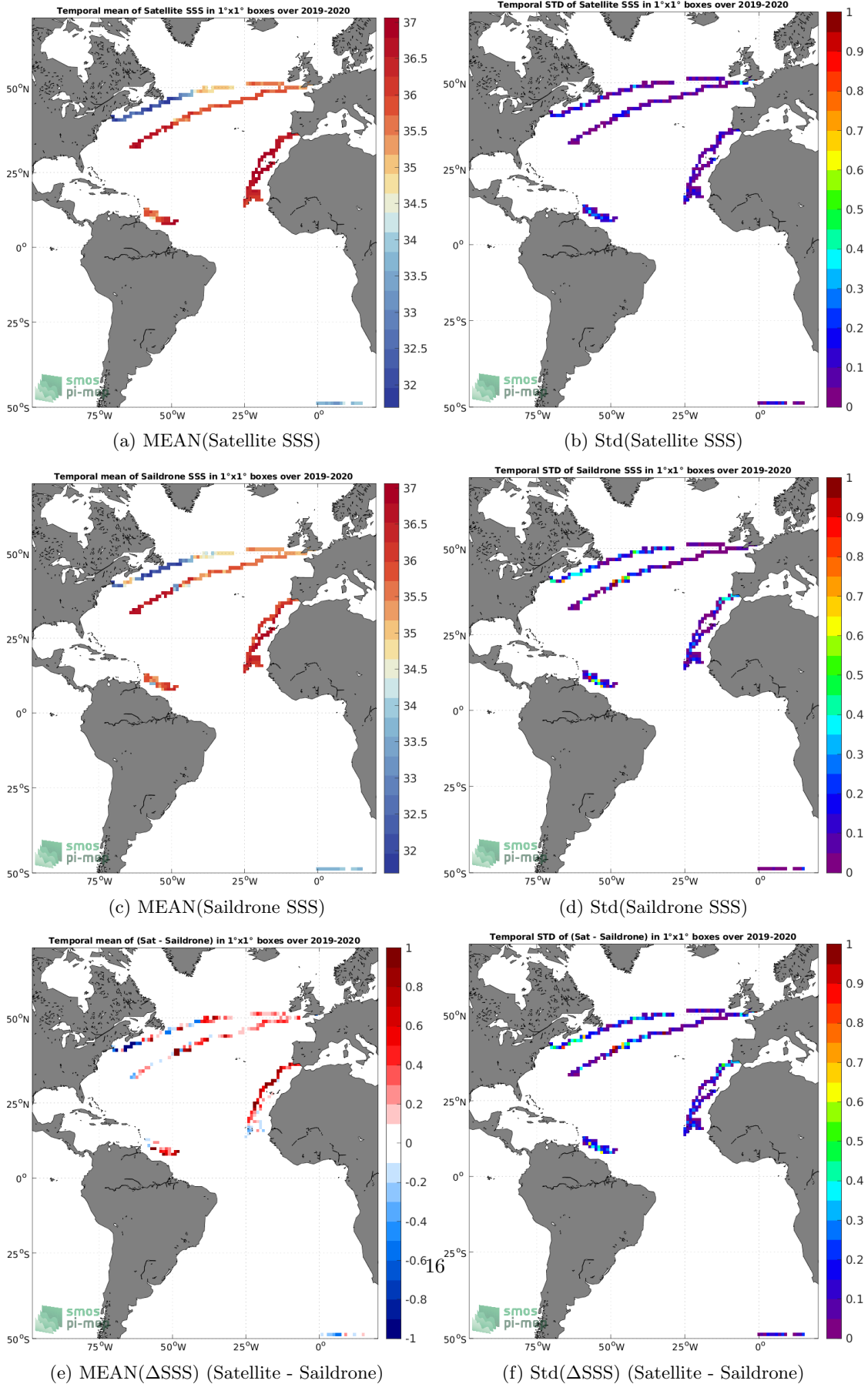
Figure 6: Temporal mean (left) and Std (right) of SSS from SMOS SSS L3 v2 - 9-Days (BEC) (top), Saildrone (middle), and of \Delta SSS (Satellite - Saildrone). Only match-up pairs are used to generate these maps.
