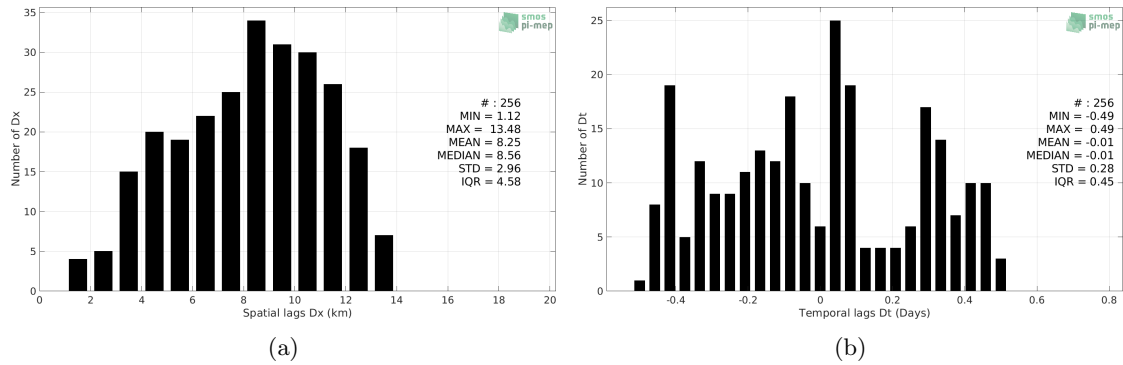
Figure 5: Histograms of the spatial (a) and temporal (b) lags between the location/time of the Sea mammals measurement and the date of the corresponding SMOS SSS L3 v2 - 9-Days (BEC) SSS pixel.
