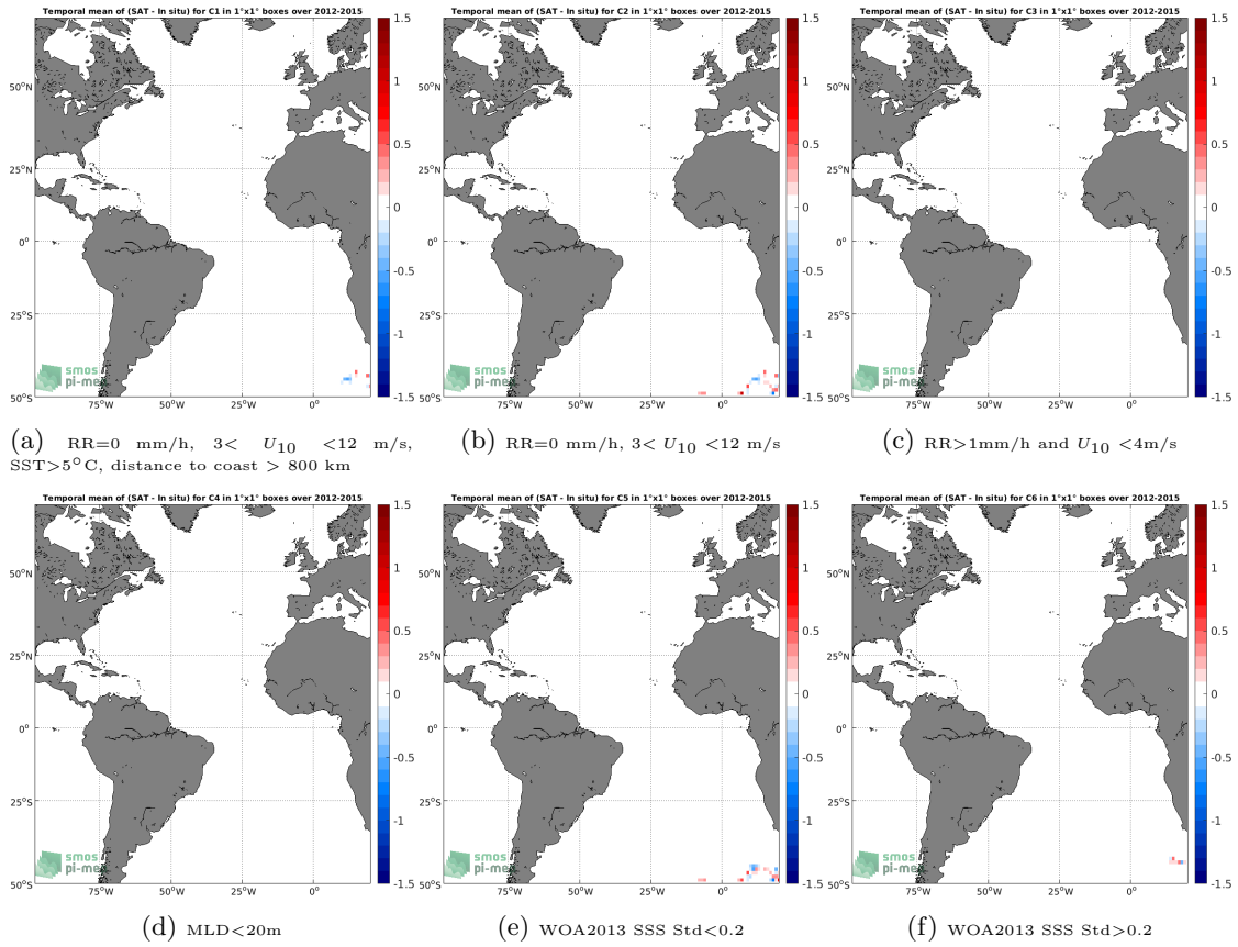
Figure 12: Temporal mean gridded over spatial boxes of size 1^\circ \times 1^\circ of \Delta SSS (SMOS SSS L3 v2 - 9-Days (BEC) - Sea mammals) for 6 different subdatasets corresponding to:RR=0 mm/h, 3 < U_{10} < 12 m/s, SST>5°C, distance to coast > 800 km (a), RR=0 mm/h, 3 < U_{10} < 12 m/s (b), RR>1mm/h and U_{10} < 4 m/s (c),MLD<20m (d),WOA2013 SSS Std<0.2 (e),WOA2013 SSS Std>0.2 (f).
