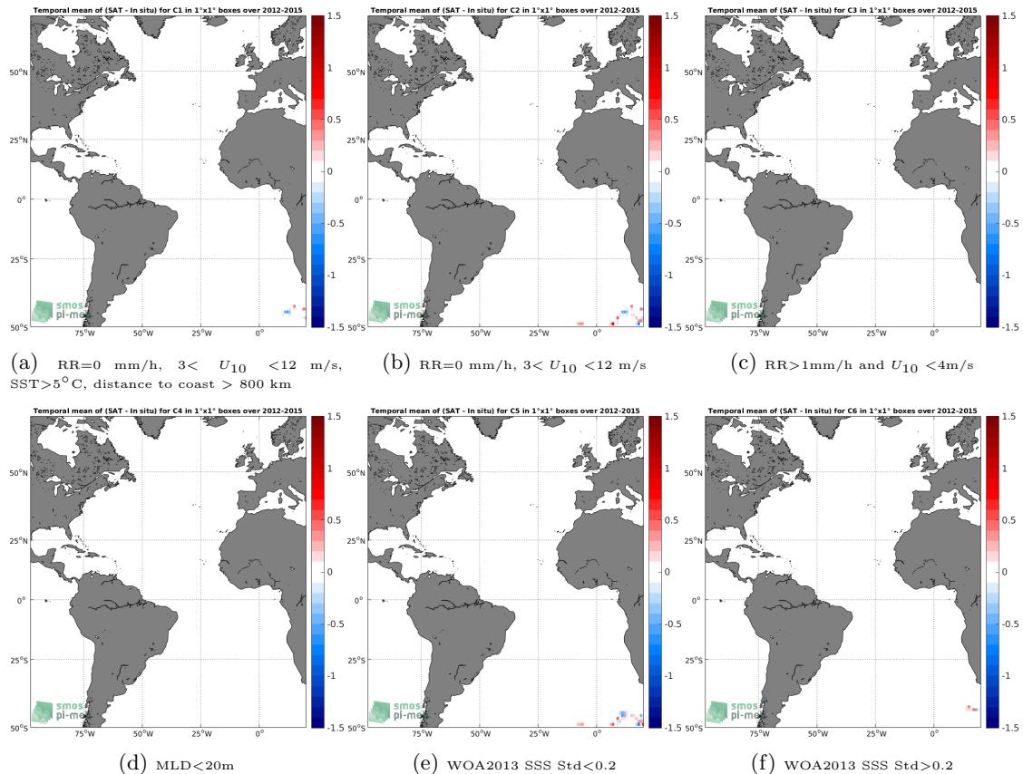
Figure 12: Temporal mean gridded over spatial boxes of size 1^{\circ}\times 1^{\circ} of \Delta\text{SSS} (SMOS L3 v2 - 9-Days (BEC) - Sea mammals) for 6 different subdatasets corresponding to:RR=0 mm/h, 3 < U_{10} < 12 m/s, SST > 5^{\circ}\text{C} , distance to coast > 800 km (a), RR=0 mm/h, 3 < U_{10} < 12 m/s (b), RR > 1\text{mm/h} and U_{10} < 4\text{m/s} (c),MLD < 20\text{m} (d),WOA2013 SSS Std < 0.2 (e),WOA2013 SSS Std > 0.2 (f).
