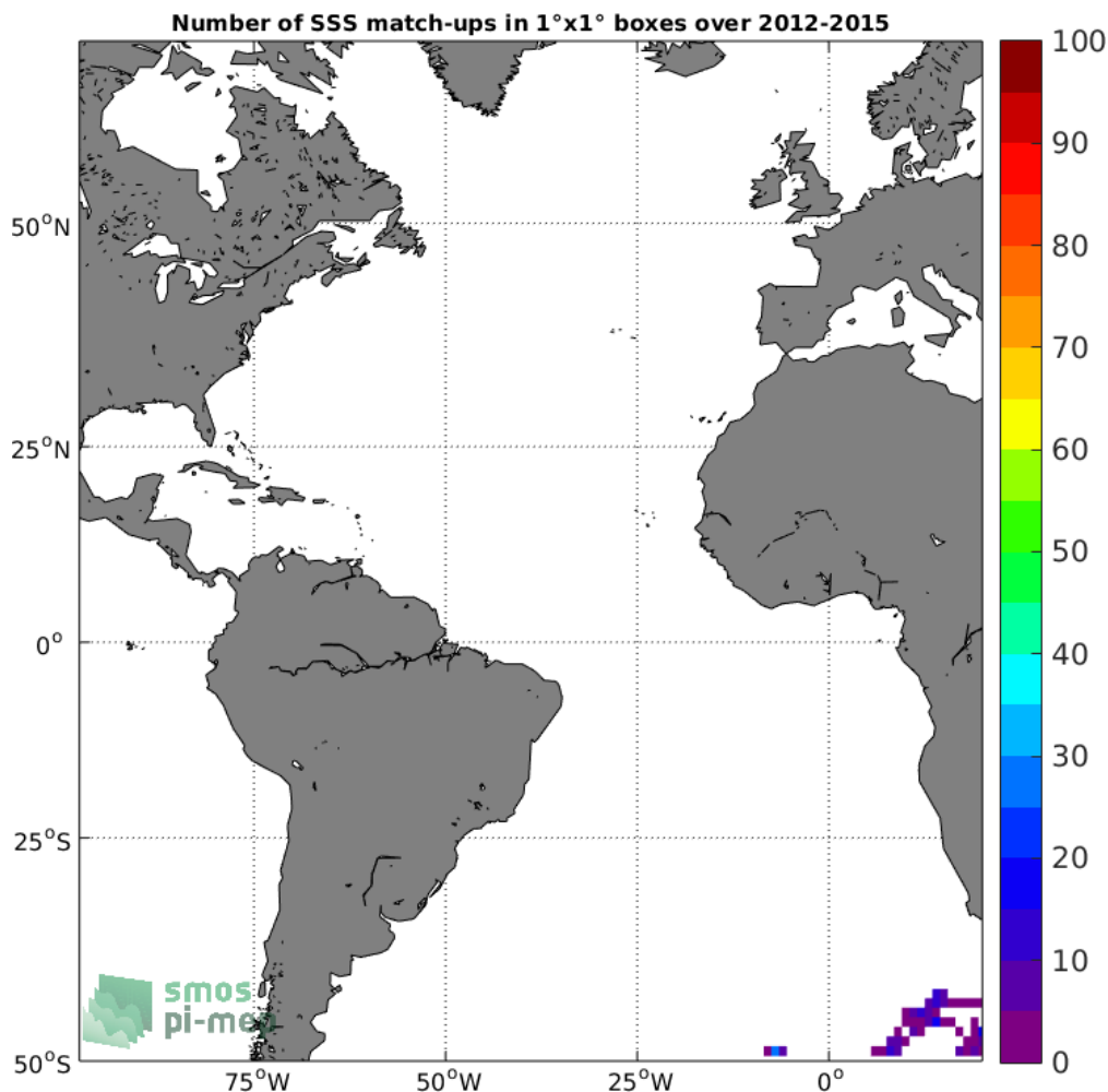
Figure 4: Number of SSS match-ups between Sea mammals SSS and the SMOS L3 v2 - 9-Days (BEC) SSS product for the Atlantic Ocean Pi-MEP region over 1°x1° boxes and for the full satellite product period.
