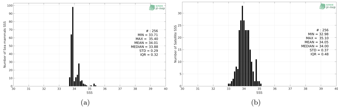
Figure 2: Histograms of SSS from Sea mammals (a) and SMOS L3 v2 - 9-Days (BEC) (b) considering all match-up pairs per bins of 0.1 over the Atlantic Ocean Pi-MEP region and for the full satellite product period.
