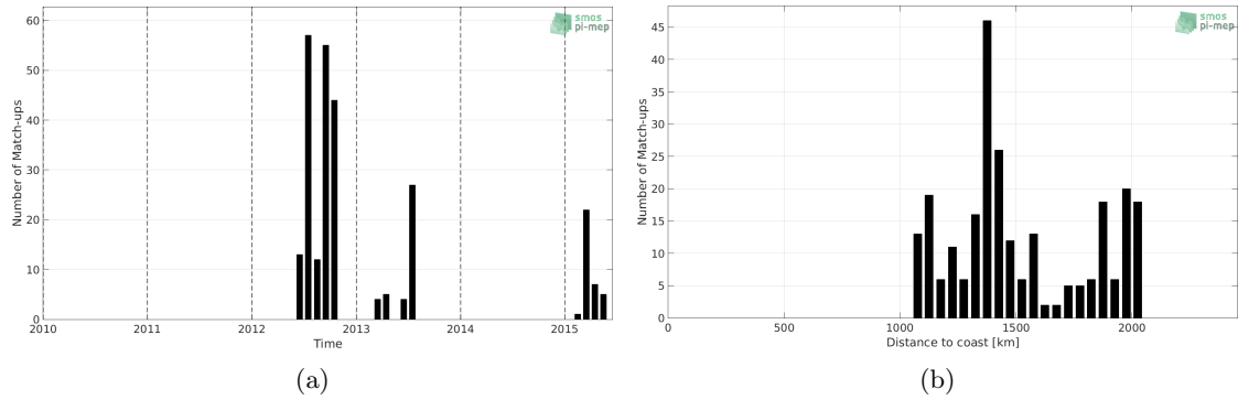
Figure 1: Number of match-ups between Sea mammals and SMOS L3 v2 - 9-Days (BEC) SSS as a function of time (a) and as function of the distance to coast (b) over the Atlantic Ocean Pi-MEP region and for the full satellite product period.
