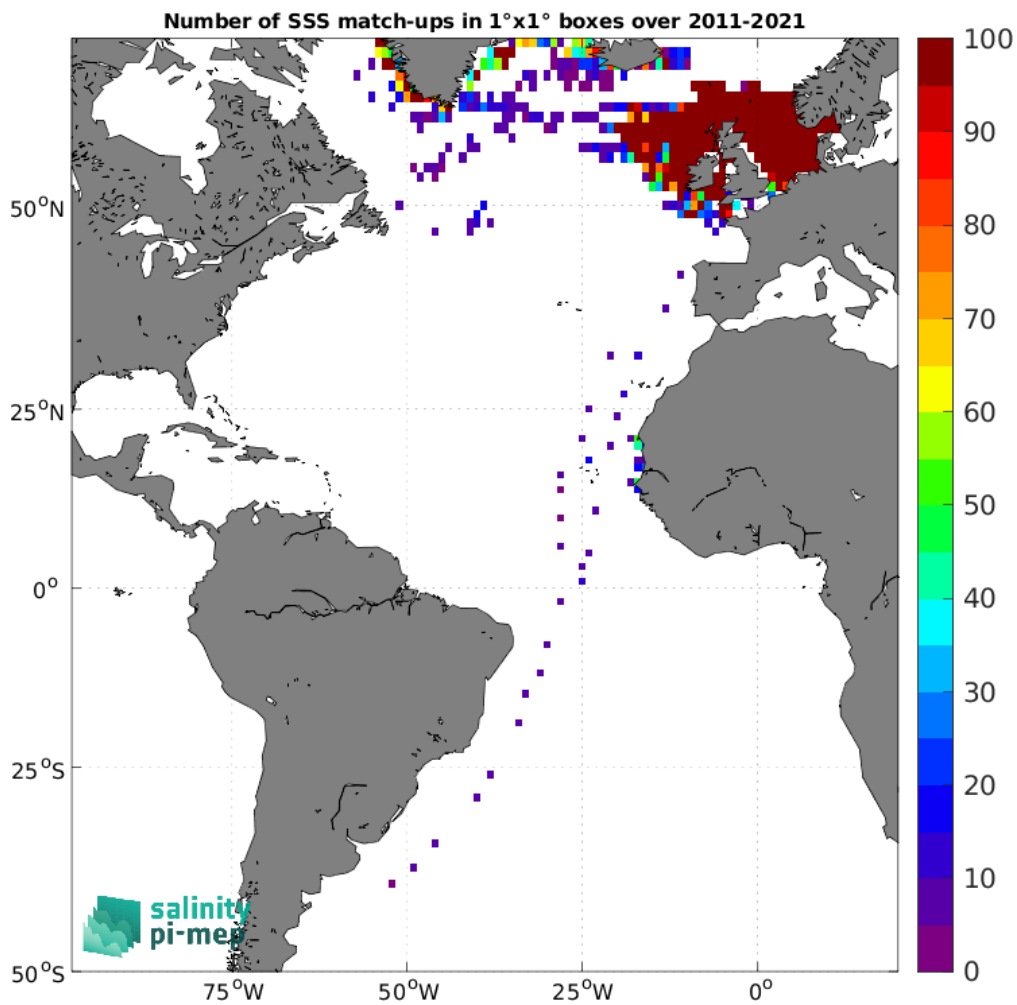
Figure 5: Number of SSS match-ups between ICES SSS and the SMOS SSS L3 v2 - 9-Days (BEC) SSS product for the Atlantic Ocean Pi-MEP region over 1°×1° boxes and for the full satellite product period.
