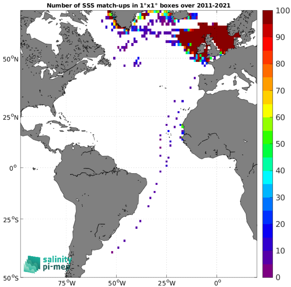
Figure 4: Number of SSS match-ups between ICES SSS and the SMOS SSS L3 v2 - 9-Days (BEC) SSS product for the Atlantic Ocean Pi-MEP region over 1^{\circ} \times 1^{\circ} boxes and for the full satellite product period.
