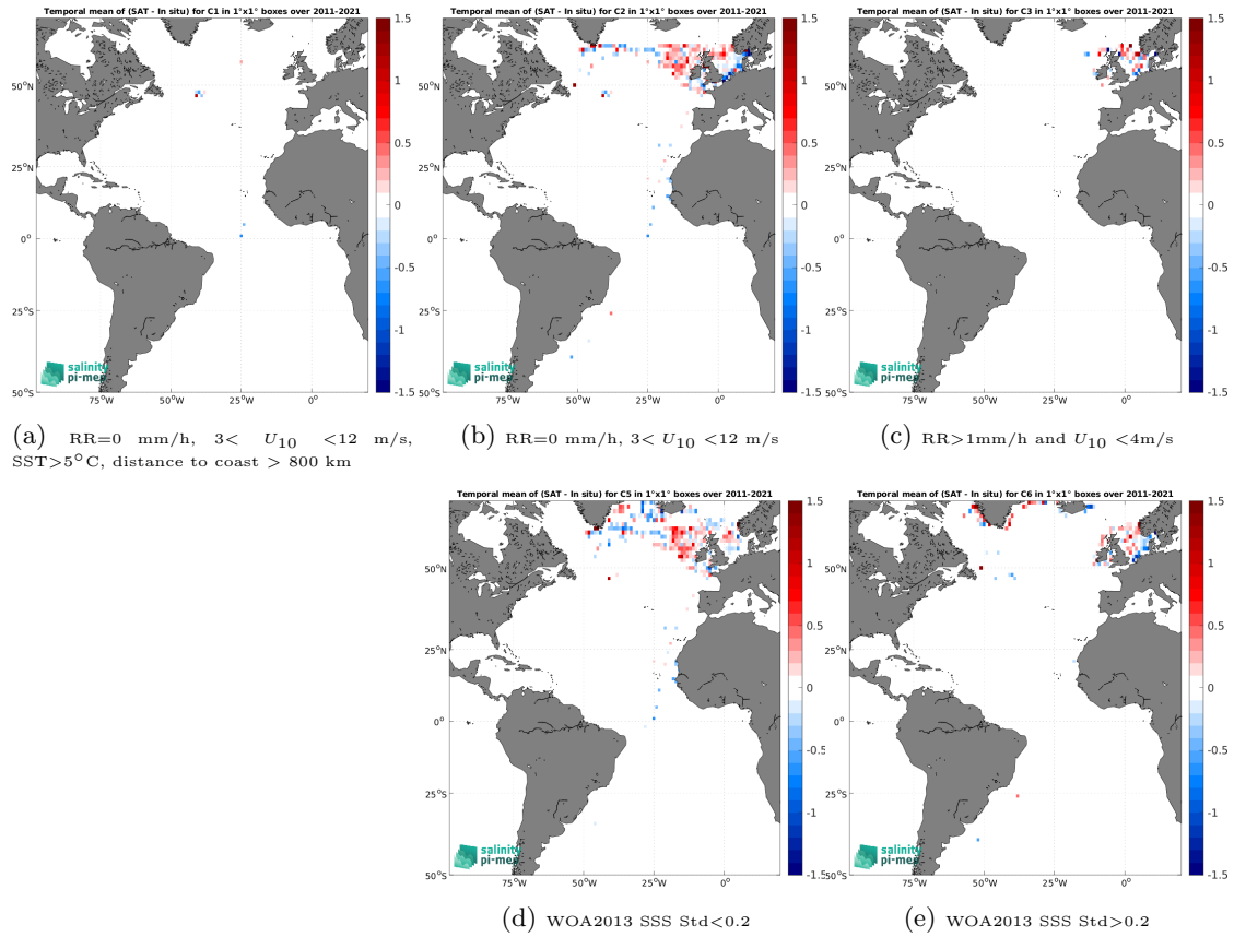
Figure 12: Temporal mean gridded over spatial boxes of size 1^\circ \times 1^\circ of \Delta SSS (SMOS SSS L3 v2 - 9-Days (BEC) - ICES) for 5 different subdatasets corresponding to:RR=0 mm/h, 3 < U_{10} < 12 m/s, SST >5^\circ\text{C} , distance to coast > 800 km (a), RR=0 mm/h, 3 < U_{10} < 12 m/s (b), RR >1 mm/h and U_{10} < 4 m/s (c), WOA2013 SSS Std <0.2 (d), WOA2013 SSS Std >0.2 (e).
