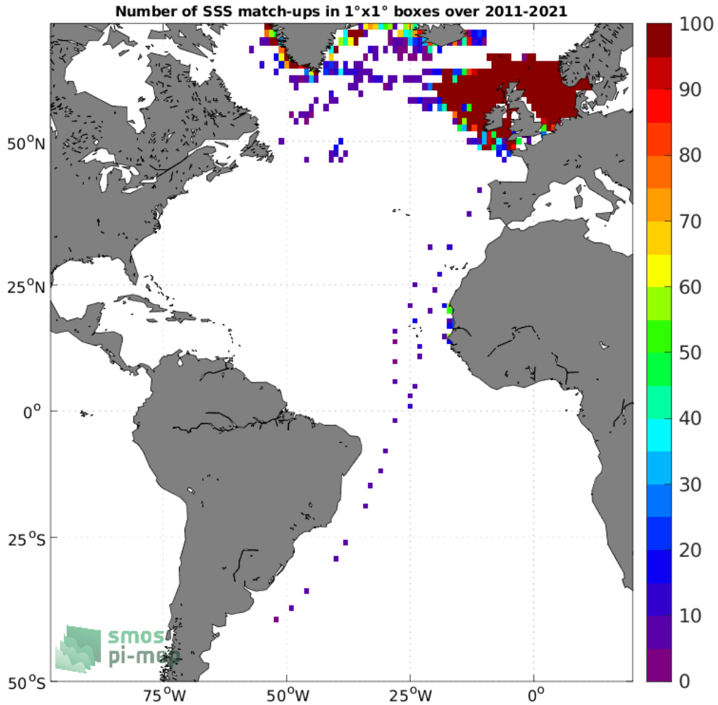
Figure 4: Number of SSS match-ups between ICES SSS and the SMOS SSS L3 v2 - 9-Days (BEC) SSS product for the Atlantic Ocean Pi-MEP region over 1°x1° boxes and for the full satellite product period.
