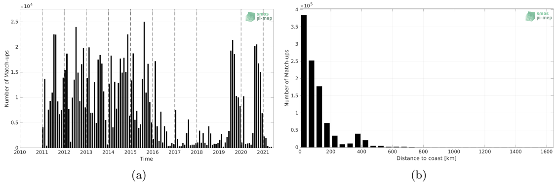
Figure 1: Number of match-ups between ICES and SMOS SSS L3 v2 - 9-Days (BEC) SSS as a function of time (a) and as function of the distance to coast (b) over the Atlantic Ocean Pi-MEP region and for the full satellite product period.
