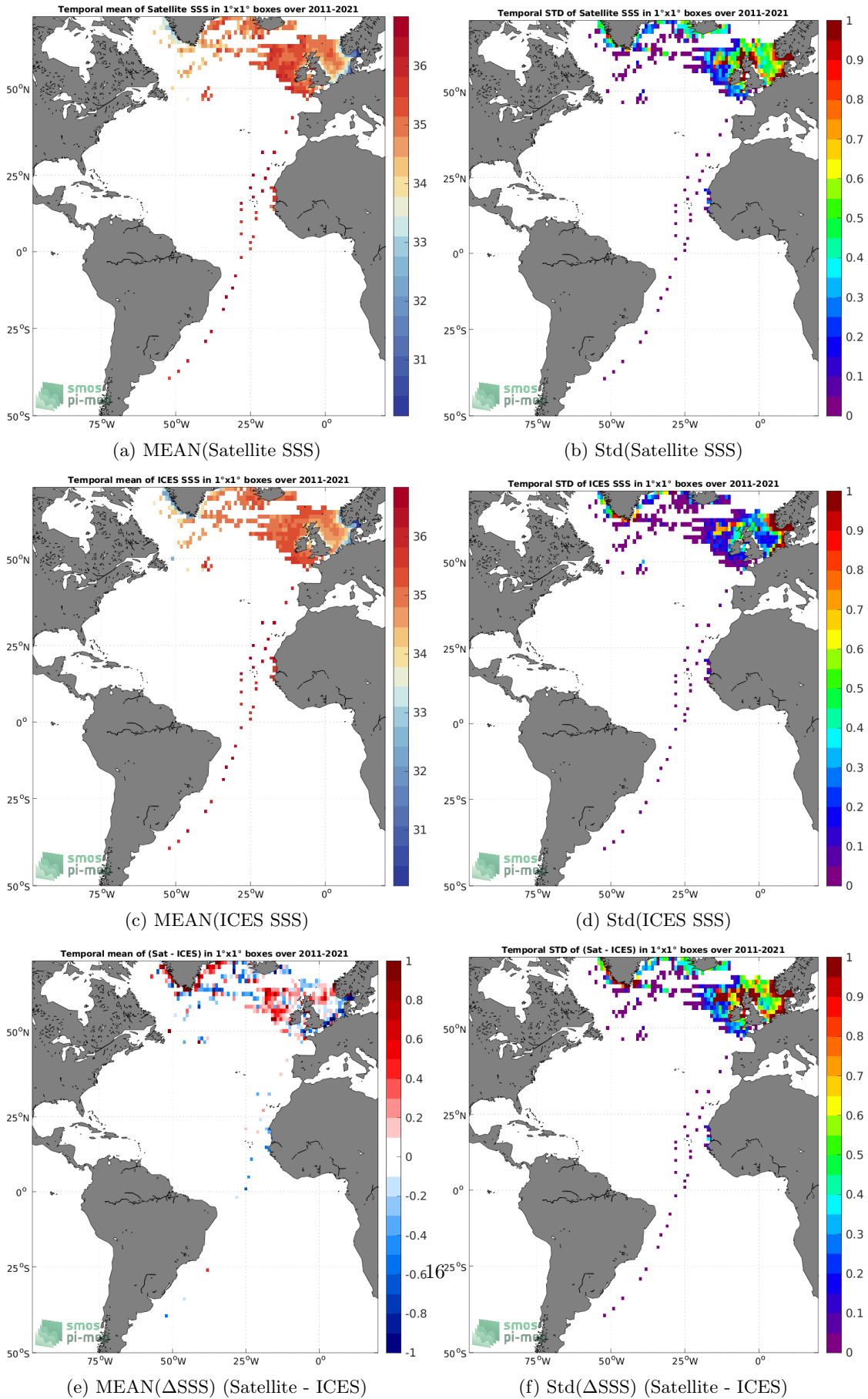
Figure 6: Temporal mean (left) and Std (right) of SSS from SMOS SSS L3 v2 - 9-Days (BEC) (top), ICES (middle), and of \Delta SSS (Satellite - ICES). Only match-up pairs are used to generate these maps.
