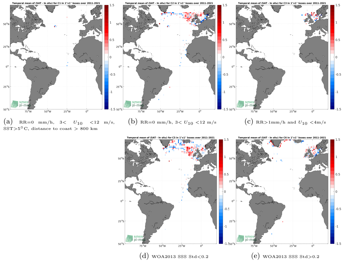
Figure 12: Temporal mean gridded over spatial boxes of size 1^\circ \times 1^\circ of \Delta SSS (SMOS SSS L3 v2 - 9-Days (BEC) - ICES) for 5 different subdatasets corresponding to:RR=0 mm/h, 3 < U_{10} < 12 m/s, SST >5^\circ\text{C} , distance to coast > 800 km (a), RR=0 mm/h, 3 < U_{10} < 12 m/s (b), RR >1 mm/h and U_{10} < 4 m/s (c), WOA2013 SSS Std <0.2 (d), WOA2013 SSS Std >0.2 (e).
