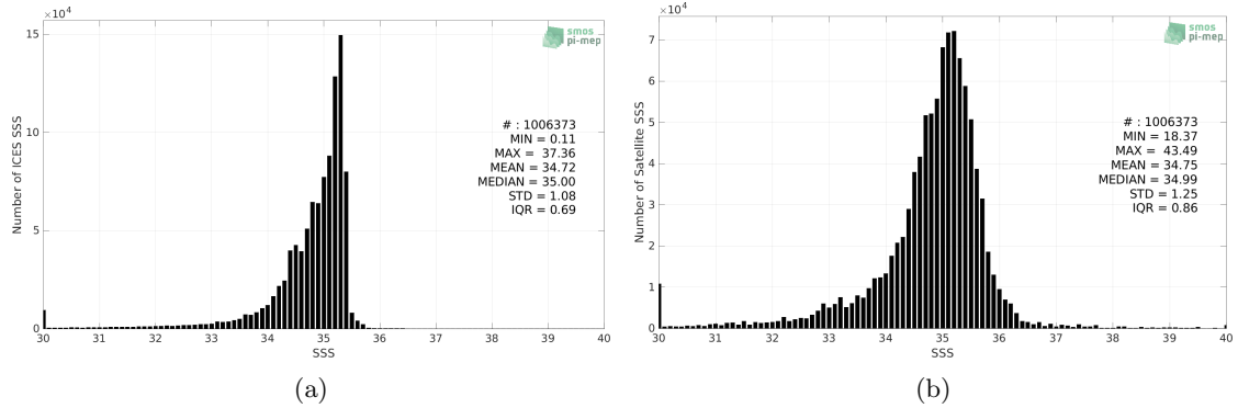
Figure 2: Histograms of SSS from ICES (a) and SMOS SSS L3 v2 - 9-Days (BEC) (b) considering all match-up pairs per bins of 0.1 over the Atlantic Ocean Pi-MEP region and for the full satellite product period.
