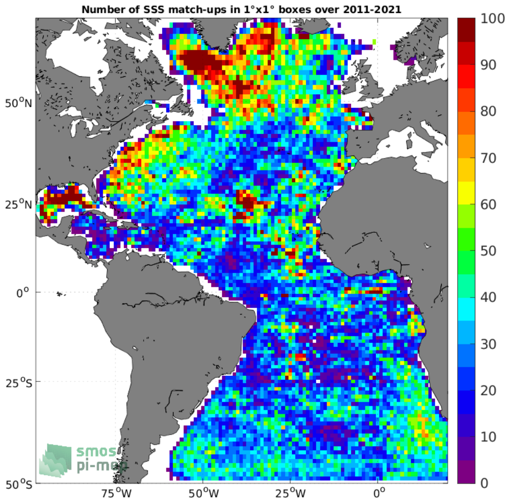
Figure 4: Number of SSS match-ups between Argo SSS and the SMOS SSS L3 v2 - 9-Days (BEC) SSS product for the Atlantic Ocean Pi-MEP region over 1°×1° boxes and for the full satellite product period.
