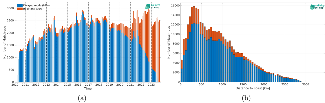
Figure 1: Number of match-ups between Argo and SMOS SSS L2-AVERAGED v700 (ESA) SSS as a function of time (a) and as function of the distance to coast (b) over the Atlantic Ocean Pi-MEP region and for the full satellite product period.
