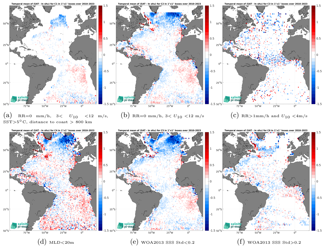
Figure 12: Temporal mean gridded over spatial boxes of size 1^\circ \times 1^\circ of \Delta SSS (SMOS SSS L2-AVERAGED v700 (ESA) - Argo) for 6 different subdatasets corresponding to:RR=0 mm/h, 3 < U_{10} < 12 m/s, SST > 5^\circ C, distance to coast > 800 km (a), RR=0 mm/h, 3 < U_{10} < 12 m/s (b), RR > 1 mm/h and U_{10} < 4 m/s (c),MLD < 20 m (d),WOA2013 SSS Std < 0.2 (e),WOA2013 SSS Std > 0.2 (f).
