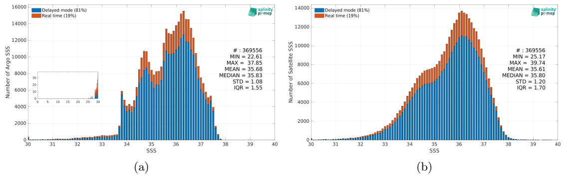
Figure 2: Histograms of SSS from Argo (a) and SMOS SSS L2-AVERAGED v700 (ESA) (b) considering all match-up pairs per bins of 0.1 over the Atlantic Ocean Pi-MEP region and for the full satellite product period.
