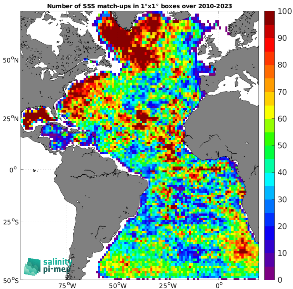
Figure 4: Number of SSS match-ups between Argo SSS and the SMOS SSS L2-AVERAGED v700 (ESA) SSS product for the Atlantic Ocean Pi-MEP region over 1^\circ \times 1^\circ boxes and for the full satellite product period.
