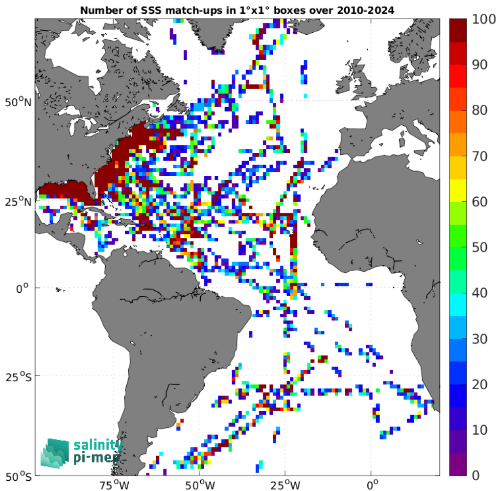
Figure 5: Number of SSS match-ups between TSG (SAMOS) SSS and the SMOS SSS L2 v700 (ESA) SSS product for the Atlantic Ocean Pi-MEP region over 1°×1° boxes and for the full satellite product period.
