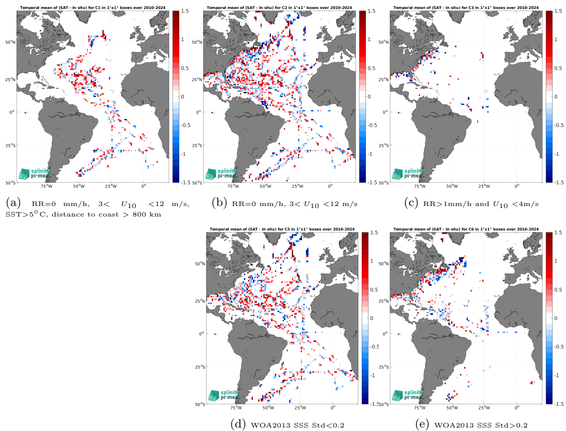
Figure 14: Temporal mean gridded over spatial boxes of size 1^\circ \times 1^\circ of \Delta\text{SSS} (SMOS SSS L2 v700 (ESA) - TSG (SAMOS)) for 5 different subdatasets corresponding to:RR=0 mm/h, 3 < U_{10} < 12 m/s, SST>5°C, distance to coast > 800 km (a), RR=0 mm/h, 3 < U_{10} < 12 m/s (b), RR>1mm/h and U_{10} < 4 m/s (c), WOA2013 SSS Std<0.2 (d), WOA2013 SSS Std>0.2 (e).
