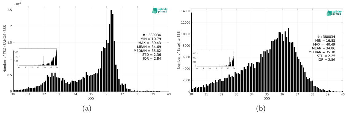
Figure 3: Histograms of SSS from TSG (SAMOS) (a) and SMOS SSS L2 v700 (ESA) (b) considering all match-up pairs per bins of 0.1 over the Atlantic Ocean Pi-MEP region and for the full satellite product period.
