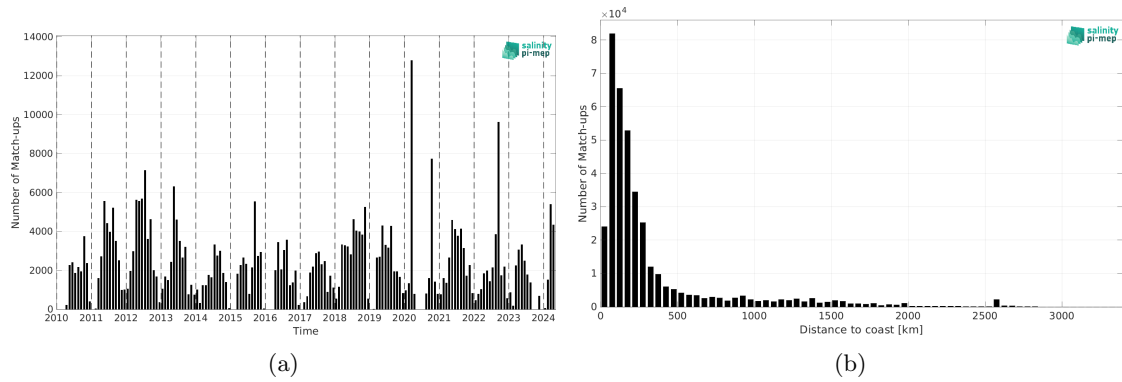
Figure 2: Number of match-ups between TSG (SAMOS) and SMOS SSS L2 v700 (ESA) SSS as a function of time (a) and as function of the distance to coast (b) over the Atlantic Ocean Pi-MEP region and for the full satellite product period.
