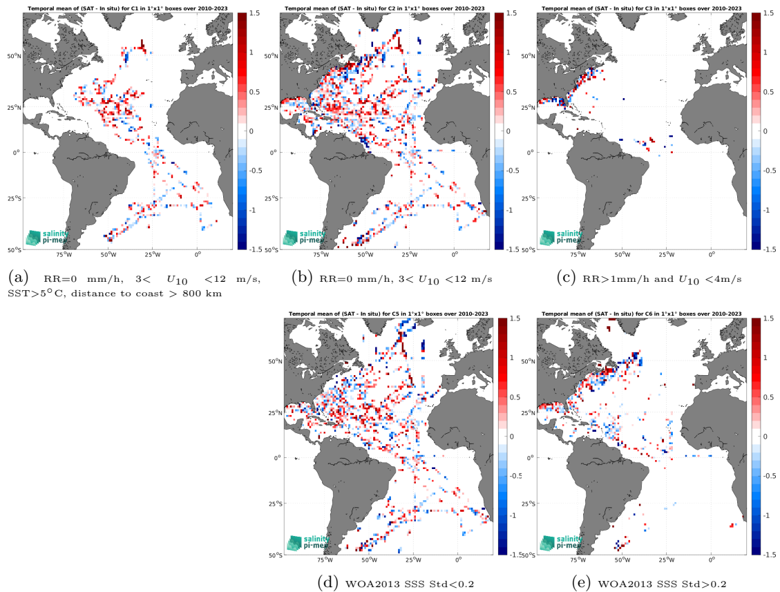
Figure 12: Temporal mean gridded over spatial boxes of size 1^\circ \times 1^\circ of \Delta\text{SSS} (SMOS SSS L2 v700 (ESA) - TSG (SAMOS)) for 5 different subdatasets corresponding to:RR=0 mm/h, 3 < U_{10} < 12 m/s, SST >5^\circ\text{C} , distance to coast > 800 km (a), RR=0 mm/h, 3 < U_{10} < 12 m/s (b), RR >1 mm/h and U_{10} < 4 m/s (c), WOA2013 SSS Std <0.2 (d), WOA2013 SSS Std >0.2 (e).
