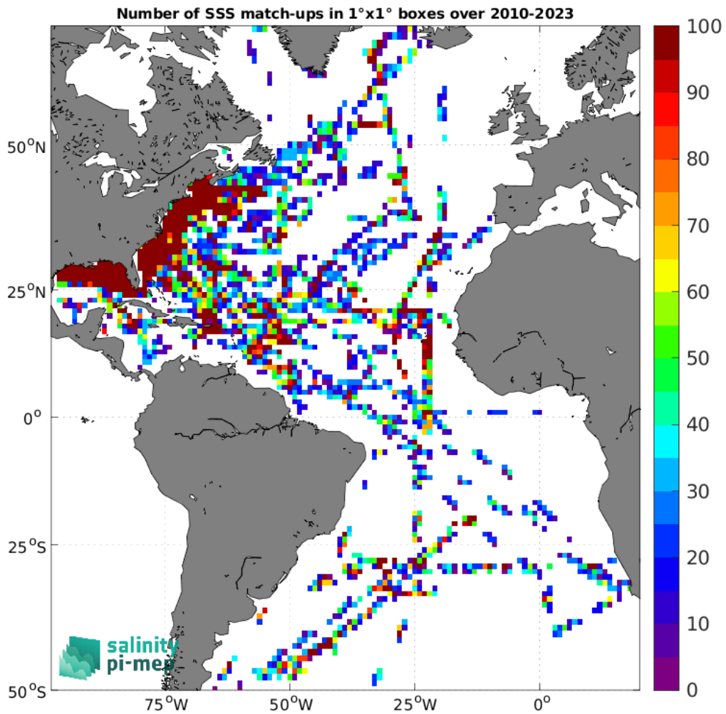
Figure 4: Number of SSS match-ups between TSG (SAMOS) SSS and the SMOS SSS L2 v700 (ESA) SSS product for the Atlantic Ocean Pi-MEP region over 1^\circ \times 1^\circ boxes and for the full satellite product period.
