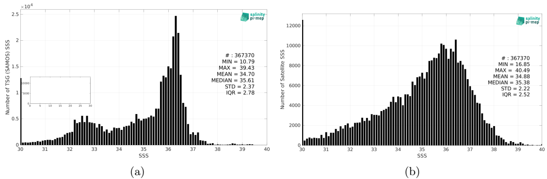
Figure 2: Histograms of SSS from TSG (SAMOS) (a) and SMOS SSS L2 v700 (ESA) (b) considering all match-up pairs per bins of 0.1 over the Atlantic Ocean Pi-MEP region and for the full satellite product period.
