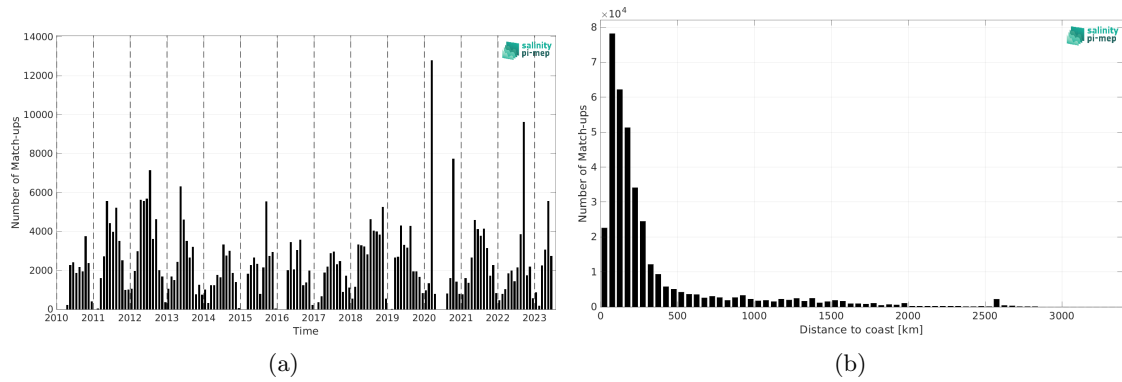
Figure 1: Number of match-ups between TSG (SAMOS) and SMOS SSS L2 v700 (ESA) SSS as a function of time (a) and as function of the distance to coast (b) over the Atlantic Ocean Pi-MEP region and for the full satellite product period.
