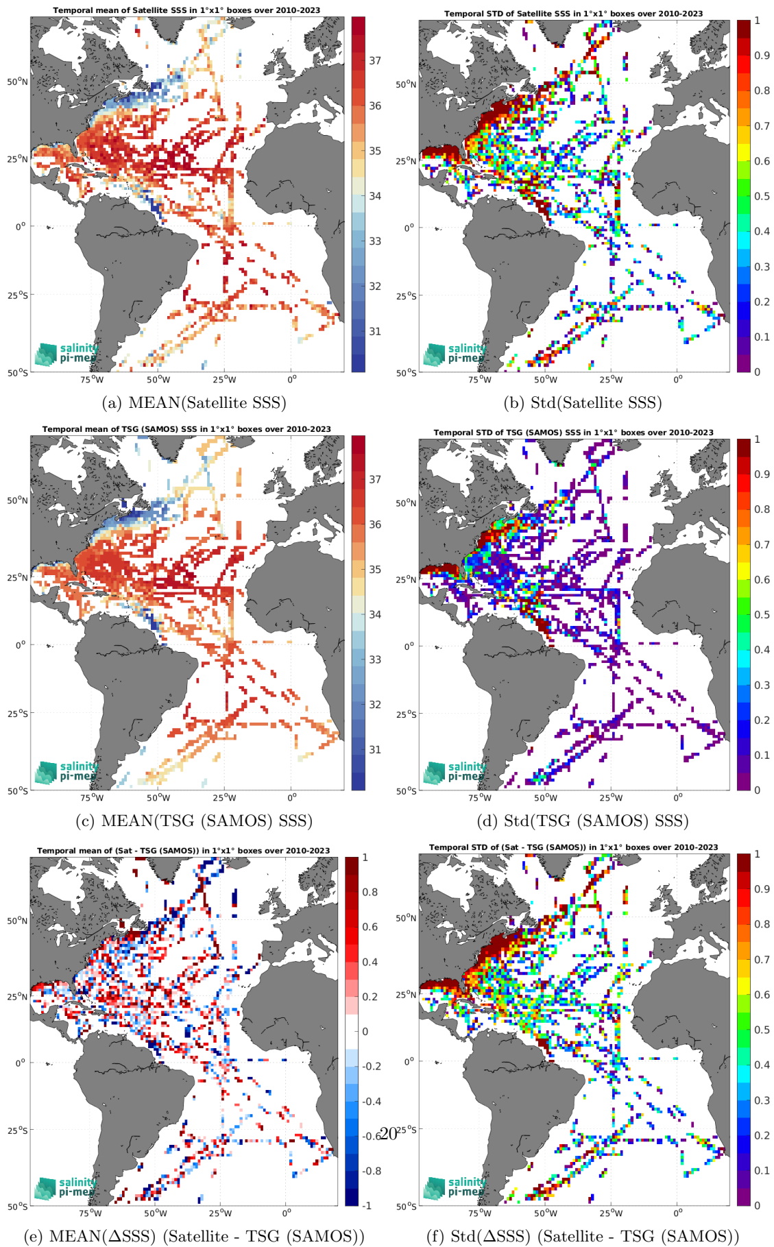
Figure 6: Temporal mean (left) and Std (right) of SSS from SMOS SSS L2 v700 (ESA) (top), TSG (SAMOS) (middle), and of \Delta SSS (Satellite - TSG (SAMOS)). Only match-up pairs are used to generate these maps.
