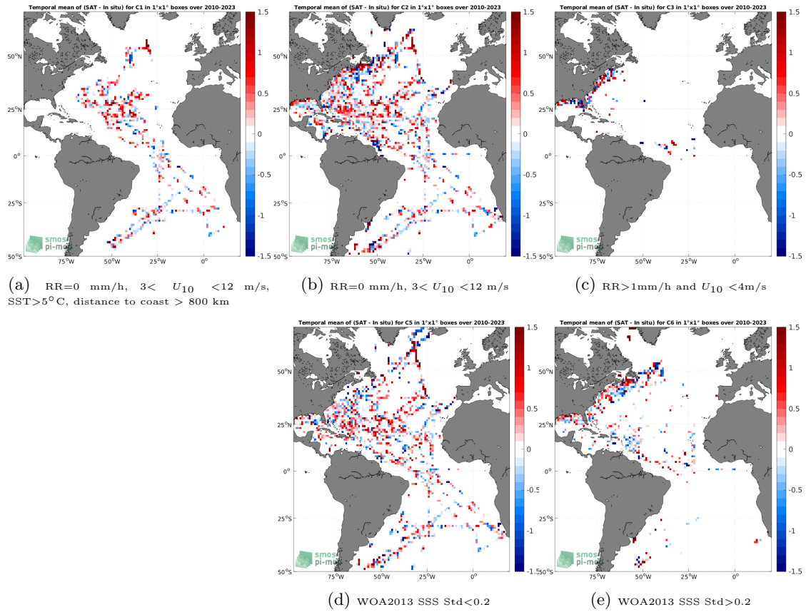
Figure 12: Temporal mean gridded over spatial boxes of size 1^\circ \times 1^\circ of \Delta SSS (SMOS SSS L2 v700 (ESA) - TSG (SAMOS)) for 5 different subdatasets corresponding to:RR=0 mm/h, 3 < U_{10} < 12 m/s, SST >5^\circ\text{C} , distance to coast > 800 km (a), RR=0 mm/h, 3 < U_{10} < 12 m/s (b), RR >1 mm/h and U_{10} < 4 m/s (c), WOA2013 SSS Std <0.2 (d), WOA2013 SSS Std >0.2 (e).
