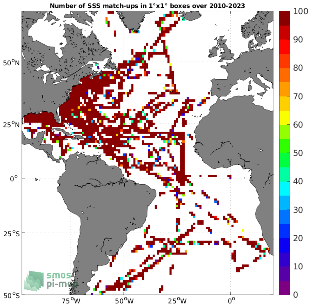
Figure 4: Number of SSS match-ups between TSG (SAMOS) SSS and the SMOS SSS L2 v700 (ESA) SSS product for the Atlantic Ocean Pi-MEP region over 1°x1° boxes and for the full satellite product period.
