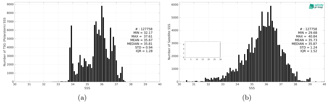
Figure 3: Histograms of SSS from TSG (Polarstern) (a) and SMOS SSS L2 v700 (ESA) (b) considering all match-up pairs per bins of 0.1 over the Atlantic Ocean Pi-MEP region and for the full satellite product period.
