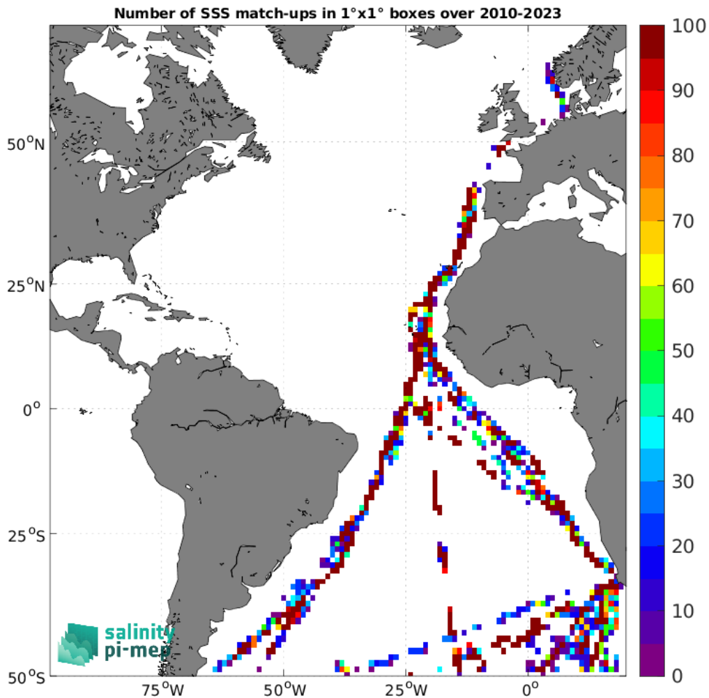
Figure 5: Number of SSS match-ups between TSG (Polarstern) SSS and the SMOS SSS L2 v700 (ESA) SSS product for the Atlantic Ocean Pi-MEP region over 1°×1° boxes and for the full satellite product period.
