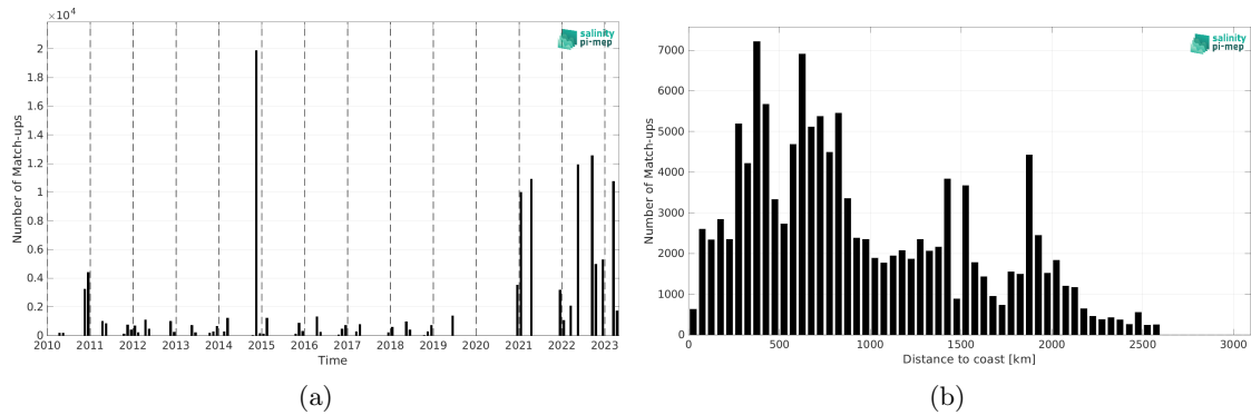
Figure 2: Number of match-ups between TSG (Polarstern) and SMOS SSS L2 v700 (ESA) SSS as a function of time (a) and as function of the distance to coast (b) over the Atlantic Ocean Pi-MEP region and for the full satellite product period.
