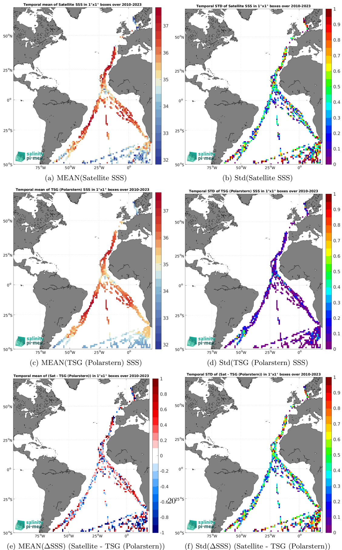
Figure 7: Temporal mean (left) and Std (right) of SSS from SMOS SSS L2 v700 (ESA) (top), TSG (Polarstern) (middle), and of \Delta SSS (Satellite - TSG (Polarstern)). Only match-up pairs are used to generate these maps.
