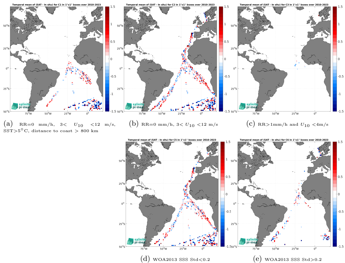
Figure 14: Temporal mean gridded over spatial boxes of size 1^\circ \times 1^\circ of \Delta\text{SSS} (SMOS SSS L2 v700 (ESA) - TSG (Polarstern)) for 5 different subdatasets corresponding to:RR=0 mm/h, 3 < U_{10} < 12 m/s, SST>5°C, distance to coast > 800 km (a), RR=0 mm/h, 3 < U_{10} < 12 m/s (b), RR>1mm/h and U_{10} < 4 m/s (c), WOA2013 SSS Std<0.2 (d), WOA2013 SSS Std>0.2 (e).
