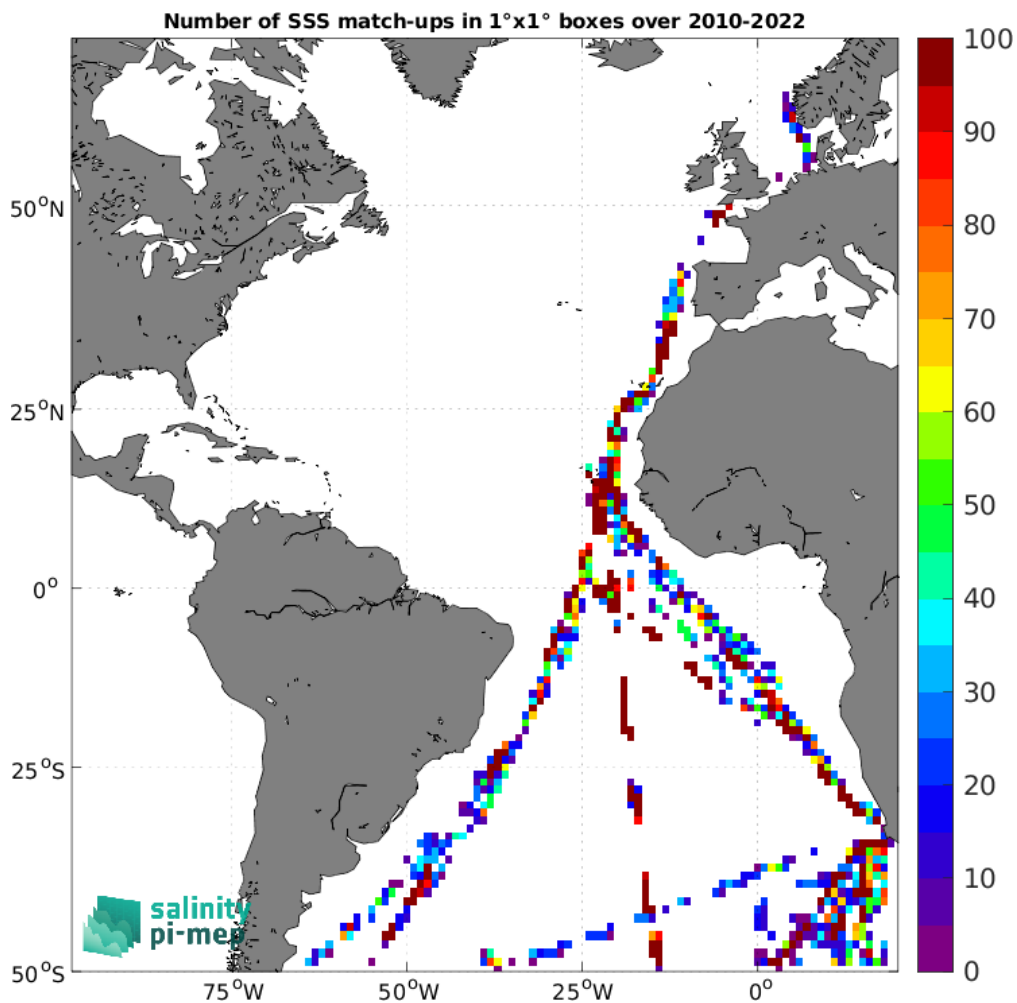
Figure 4: Number of SSS match-ups between TSG (Polarstern) SSS and the SMOS SSS L2 v700 (ESA) SSS product for the Atlantic Ocean Pi-MEP region over 1°×1° boxes and for the full satellite product period.
