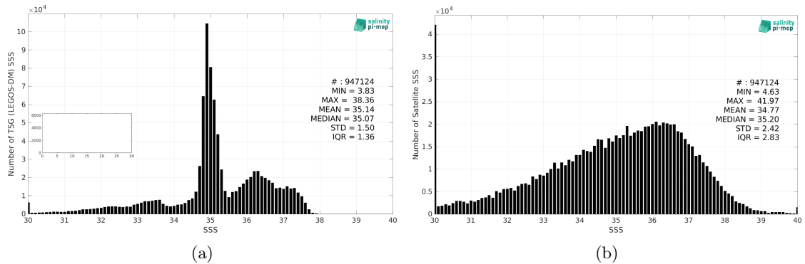
Figure 2: Histograms of SSS from TSG (LEGOS-DM) (a) and SMOS SSS L2 v700 (ESA) (b) considering all match-up pairs per bins of 0.1 over the Atlantic Ocean Pi-MEP region and for the full satellite product period.
