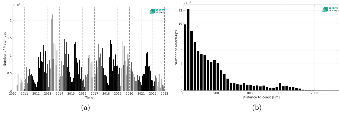
Figure 1: Number of match-ups between TSG (LEGOS-DM) and SMOS SSS L2 v700 (ESA) SSS as a function of time (a) and as function of the distance to coast (b) over the Atlantic Ocean Pi-MEP region and for the full satellite product period.
