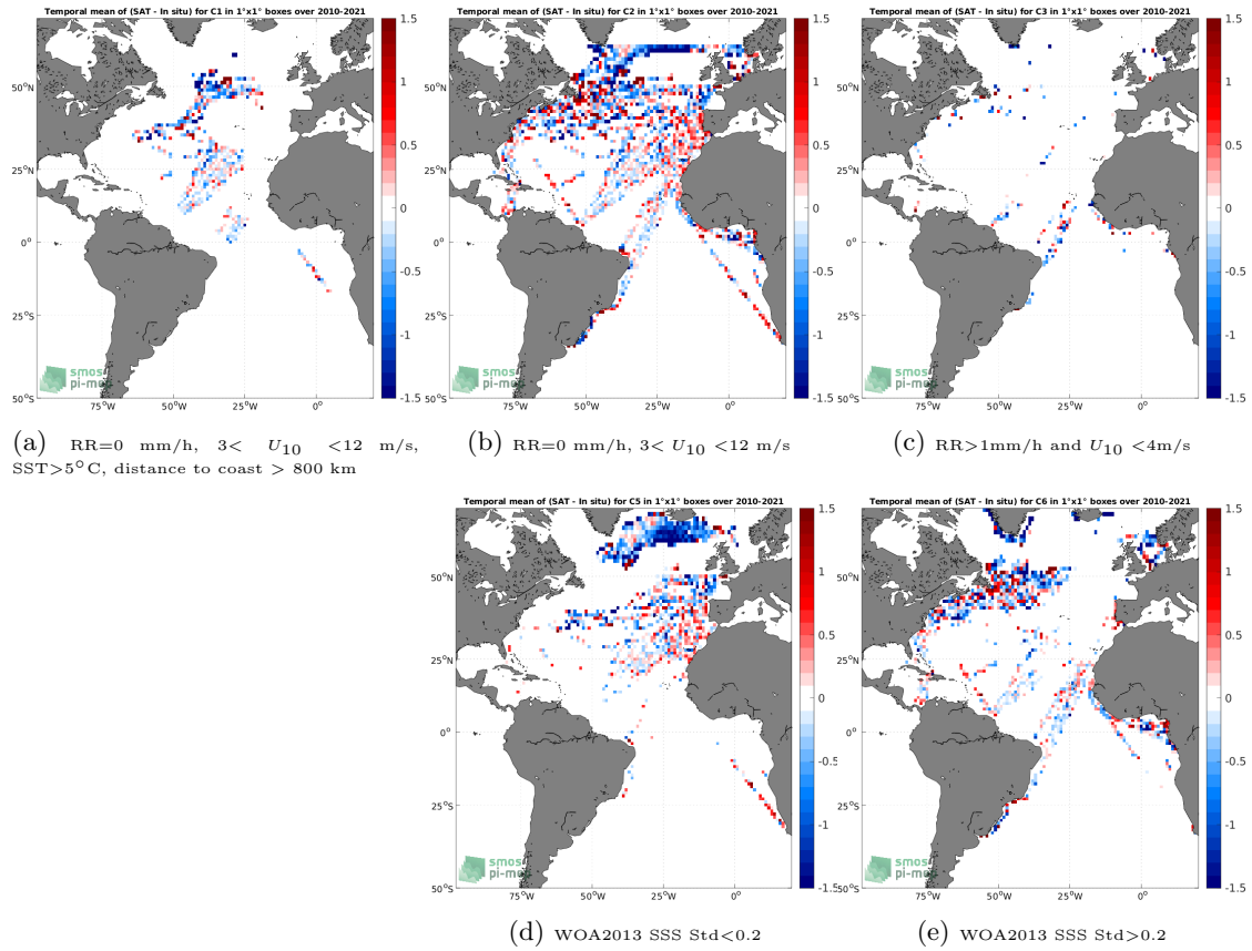
Figure 12: Temporal mean gridded over spatial boxes of size 1^\circ \times 1^\circ of \Delta SSS (SMOS SSS L2 v700 (ESA) - TSG (LEGOS-DM)) for 5 different subdatasets corresponding to:RR=0 mm/h, 3 < U_{10} < 12 m/s, SST >5^\circ\text{C} , distance to coast > 800 km (a), RR=0 mm/h, 3 < U_{10} < 12 m/s (b), RR >1 mm/h and U_{10} < 4 m/s (c), WOA2013 SSS Std <0.2 (d), WOA2013 SSS Std >0.2 (e).
