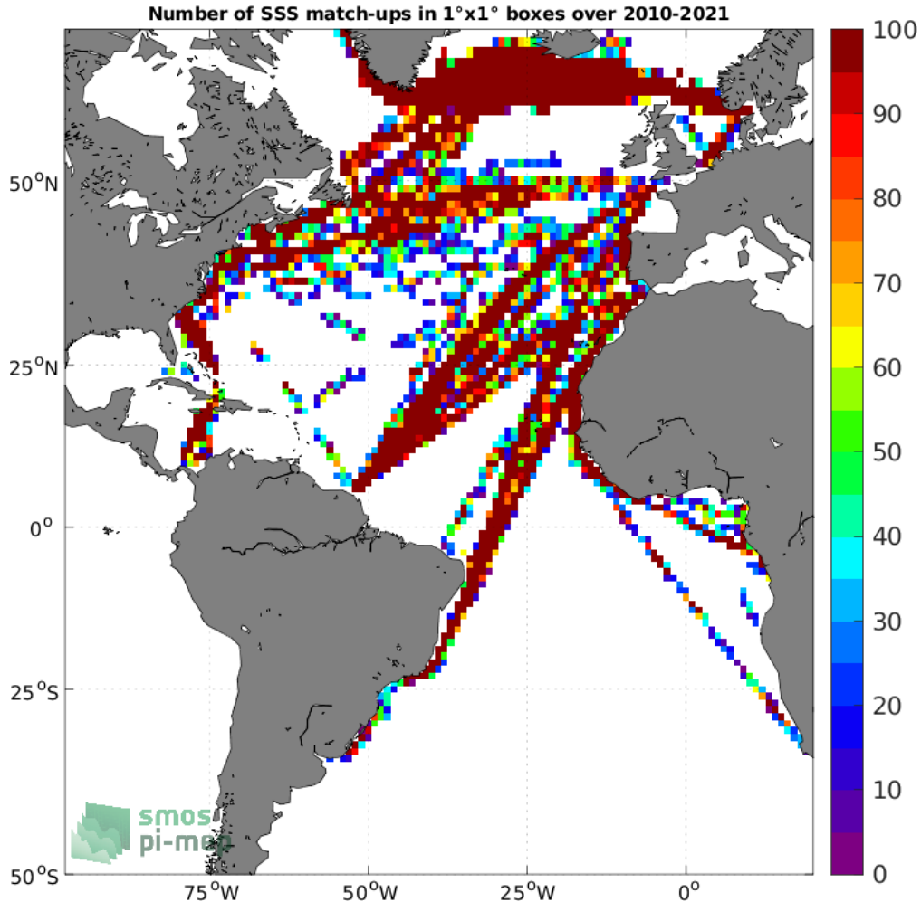
Figure 4: Number of SSS match-ups between TSG (LEGOS-DM) SSS and the SMOS SSS L2 v700 (ESA) SSS product for the Atlantic Ocean Pi-MEP region over 1^\circ \times 1^\circ boxes and for the full satellite product period.
