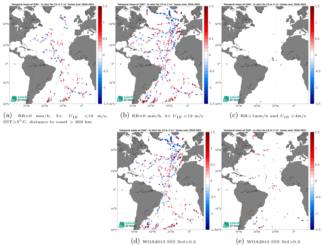
Figure 14: Temporal mean gridded over spatial boxes of size 1^\circ \times 1^\circ of \Delta\text{SSS} (SMOS SSS L2 v700 (ESA) - TSG (GOSUD-Sailing-ship)) for 5 different subdatasets corresponding to:RR=0 mm/h, 3 < U_{10} < 12 m/s, SST >5^\circ\text{C} , distance to coast > 800 km (a), RR=0 mm/h, 3 < U_{10} < 12 m/s (b), RR >1 mm/h and U_{10} < 4 m/s (c), WOA2013 SSS Std <0.2 (d), WOA2013 SSS Std >0.2 (e).
