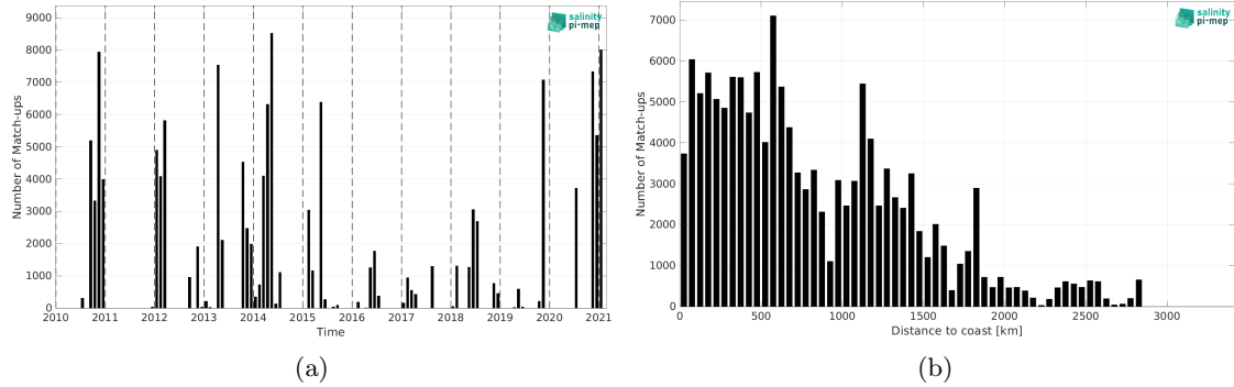
Figure 2: Number of match-ups between TSG (GOSUD-Sailing-ship) and SMOS SSS L2 v700 (ESA) SSS as a function of time (a) and as function of the distance to coast (b) over the Atlantic Ocean Pi-MEP region and for the full satellite product period.
