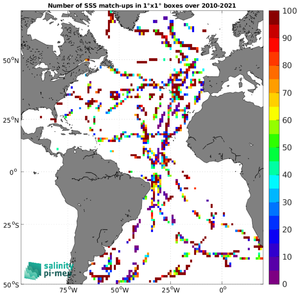
Figure 5: Number of SSS match-ups between TSG (GOSUD-Sailing-ship) SSS and the SMOS SSS L2 v700 (ESA) SSS product for the Atlantic Ocean Pi-MEP region over 1°x1° boxes and for the full satellite product period.
