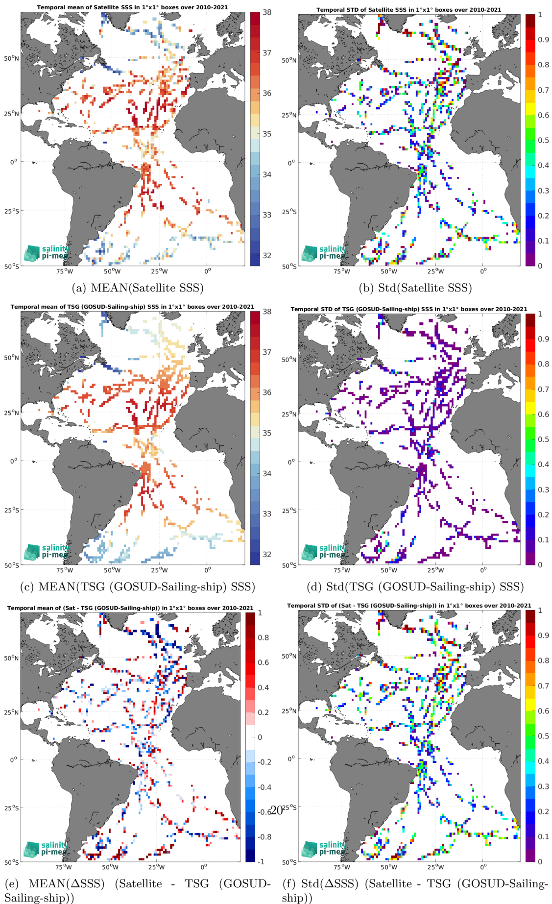
Figure 7: Temporal mean (left) and Std (right) of SSS from SMOS SSS L2 v700 (ESA) (top), TSG (GOSUD-Sailing-ship) (middle), and of \Delta SSS (Satellite - TSG (GOSUD-Sailing-ship)). Only match-up pairs are used to generate these maps.
