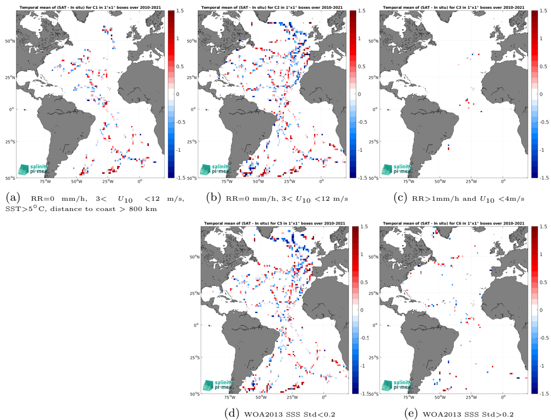
Figure 12: Temporal mean gridded over spatial boxes of size 1^\circ \times 1^\circ of \Delta\text{SSS} (SMOS SSS L2 v700 (ESA) - TSG (GOSUD-Sailing-ship)) for 5 different subdatasets corresponding to:RR=0 mm/h, 3 < U_{10} < 12 m/s, SST >5^\circ\text{C} , distance to coast > 800 km (a), RR=0 mm/h, 3 < U_{10} < 12 m/s (b), RR >1 mm/h and U_{10} < 4 m/s (c), WOA2013 SSS Std <0.2 (d), WOA2013 SSS Std >0.2 (e).
